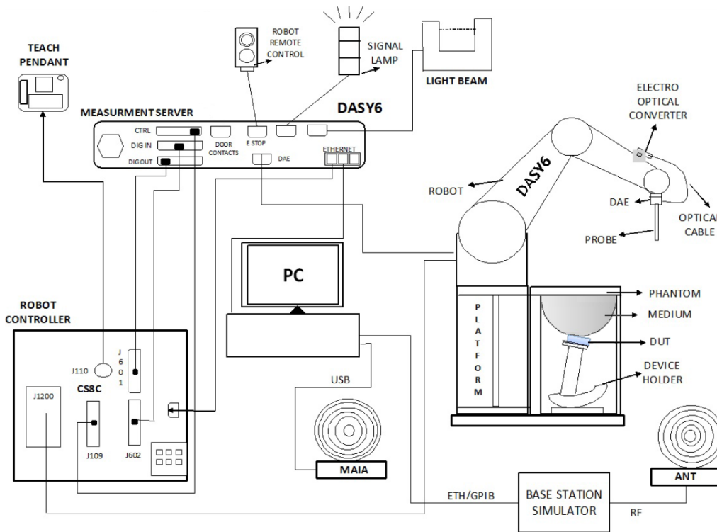
Fig-4.1 SPEAG DASY6 System Setup
