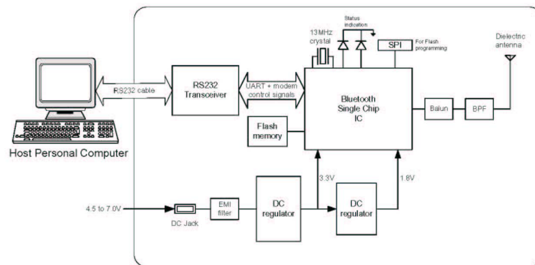
Figure 1: Bluetooth Serial Port Dongle Block Diagram
