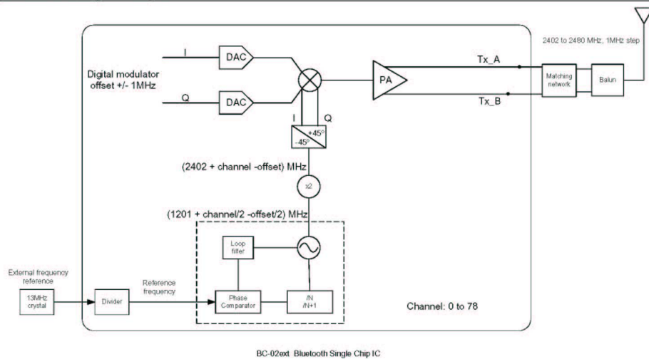
Figure 3 Bluetooth Single Chip IC- Transmitter Circuit
