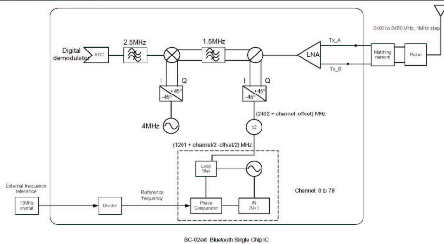
Figure 2: Bluetooth Single Chip IC- Receiver Circuit
