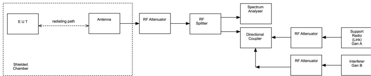
Figure i Test Setup
