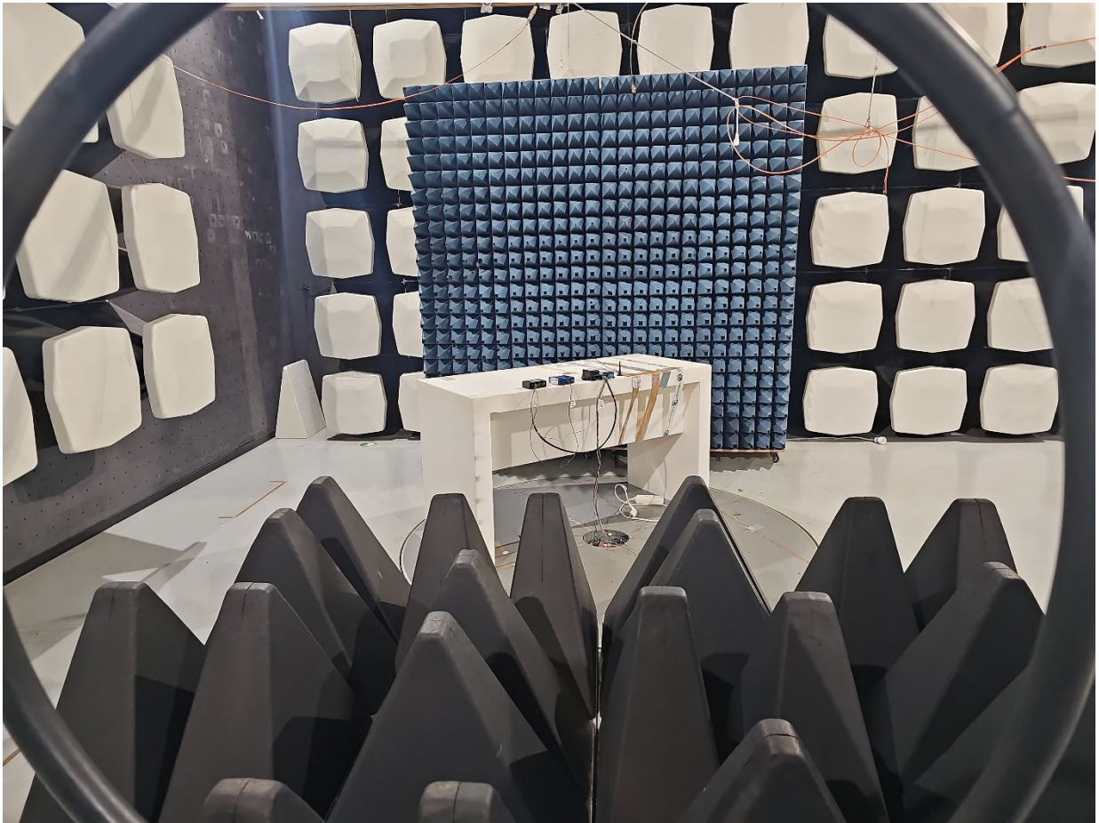
Fig. Mea.: 3 : Radiated RF Parameter Internal Antenna Image 3
