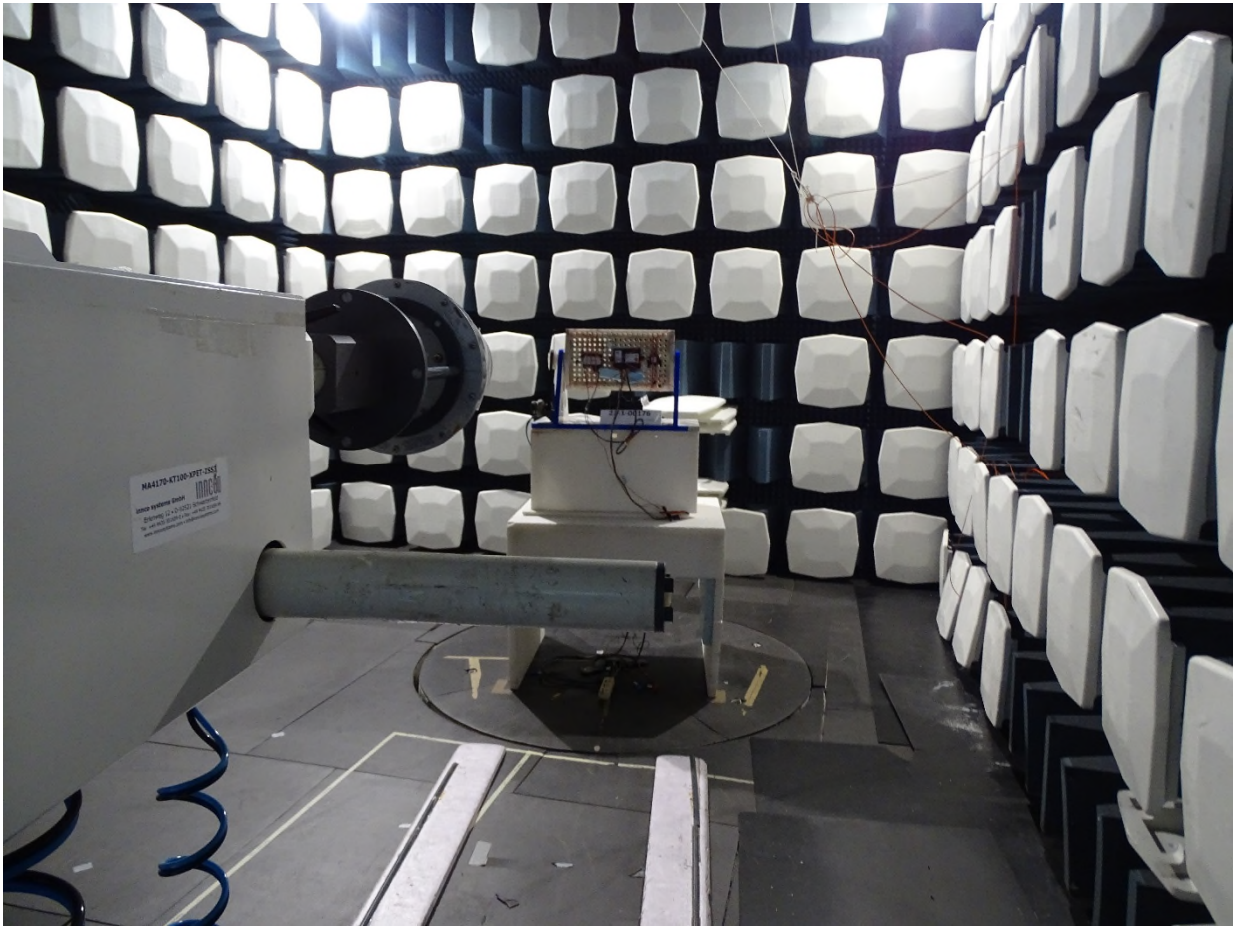
Fig. Mea.: 7 : Radiated RF Parameter Internal Antenna Image 7
