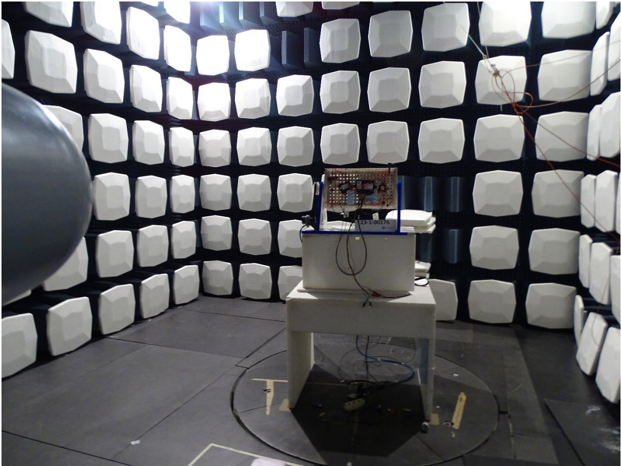
Fig. Mea.: 6 : Radiated RF Parameter External Antenna Image 6
