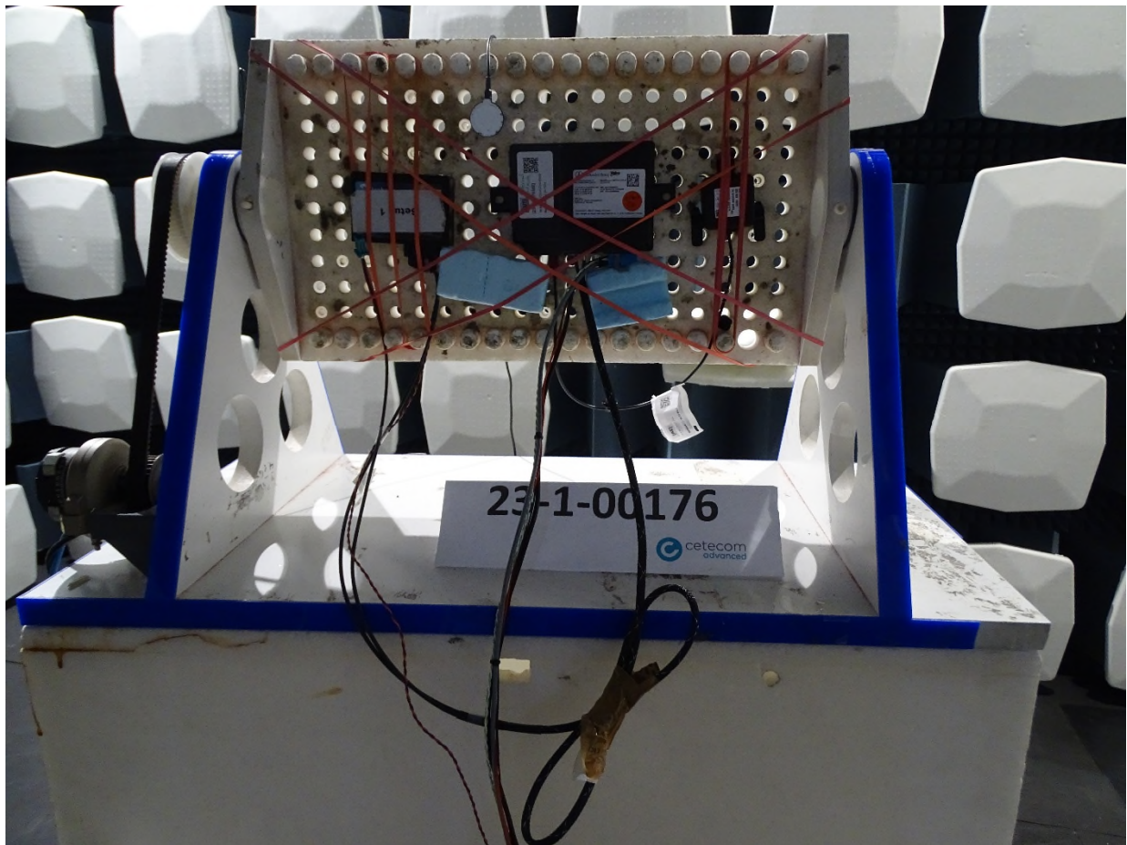
Fig. Mea.: 8 : Radiated RF Parameter Internal Antenna Image 8
