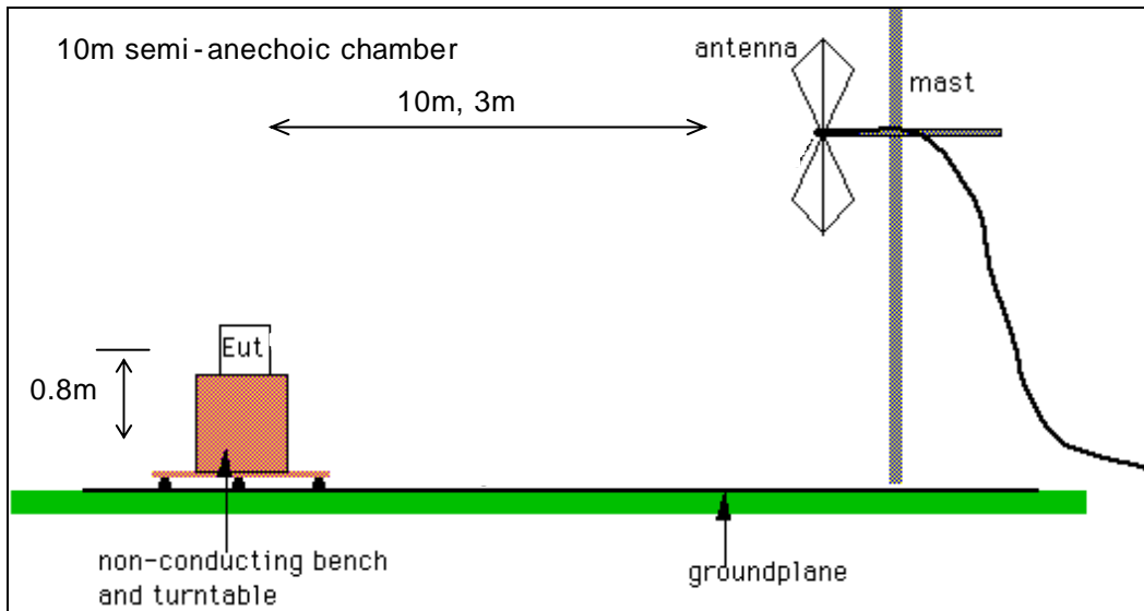
<General test set-up for radiated emissions>
