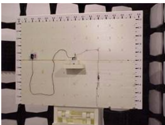
Picture 3. FCC Part 15 AC powerline conducted emissions
