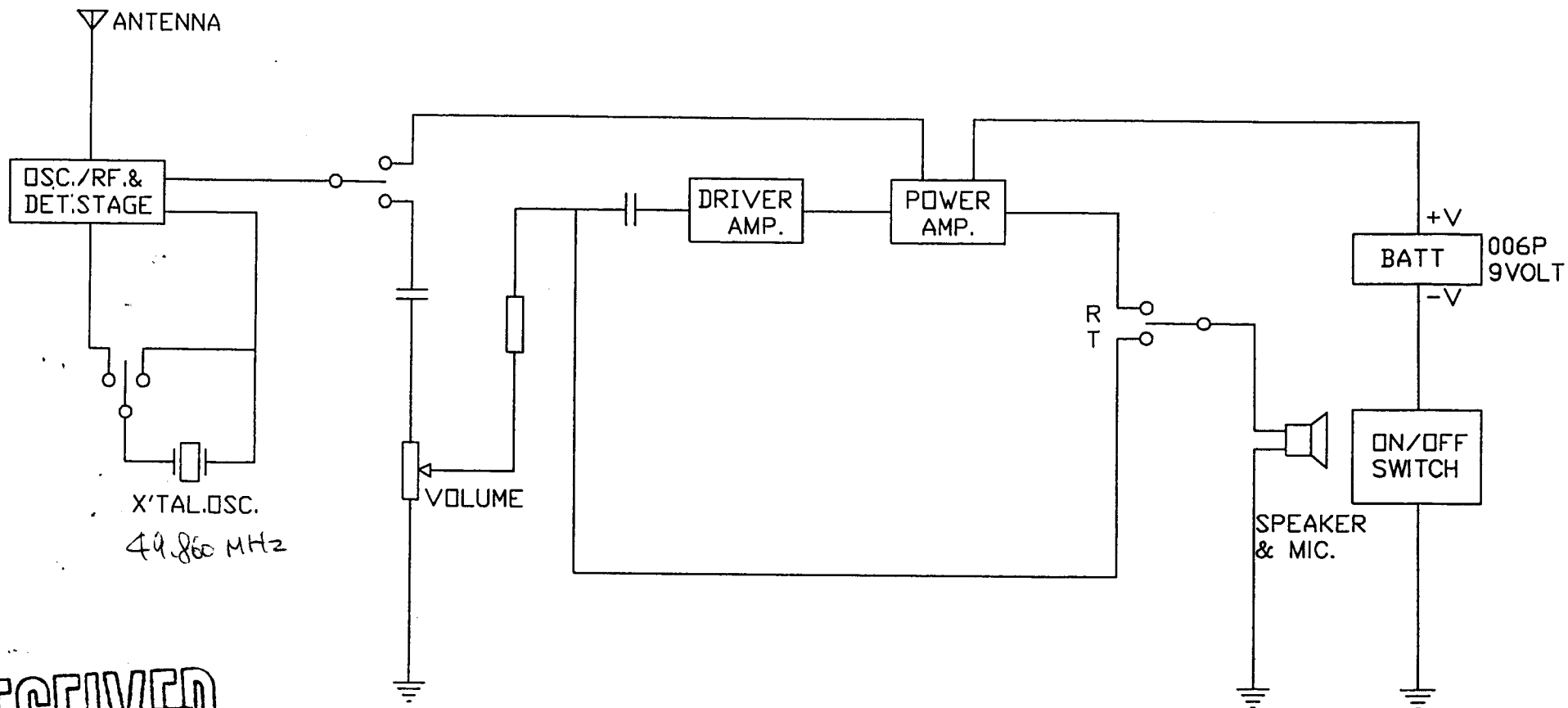
BLOCK DIAGRAM
