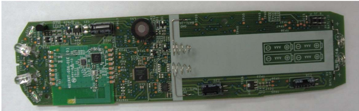
FRONTSIDE MAIN BOARD
