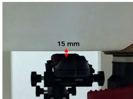
Fig.4 EUT back to flat phantom
