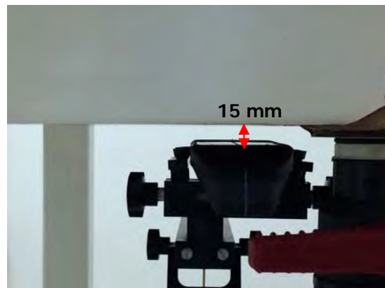
Fig.3 EUT front to flat phantom
