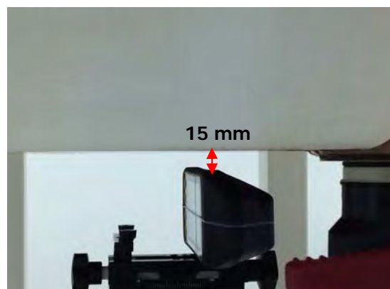
Fig.6 EUT left to flat phantom
