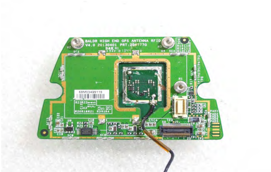
Open View of EUT-10
