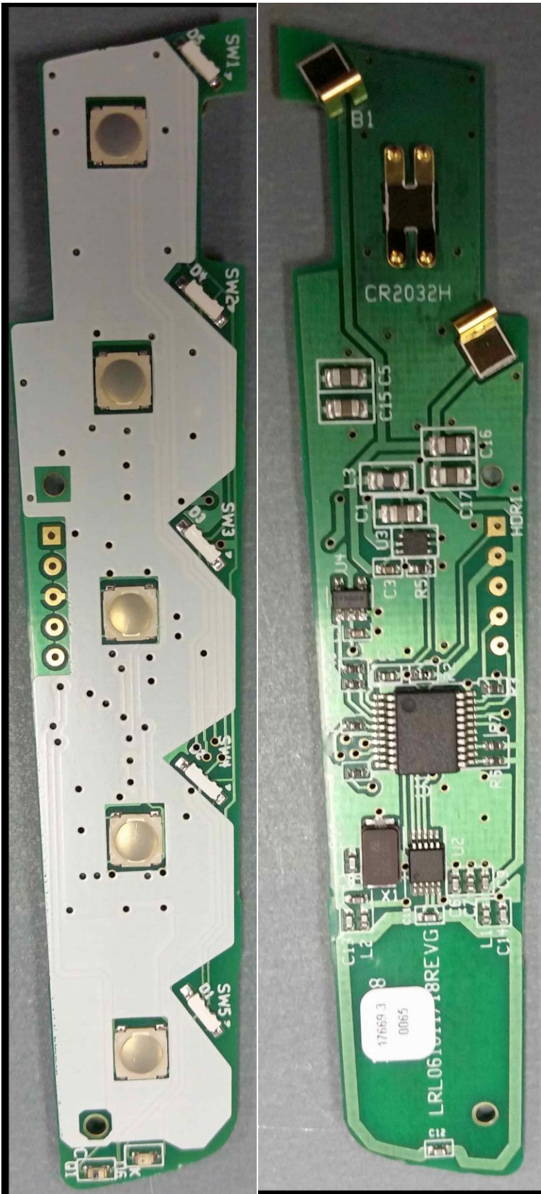
PCB Top (Left) , Bottom (Right)
