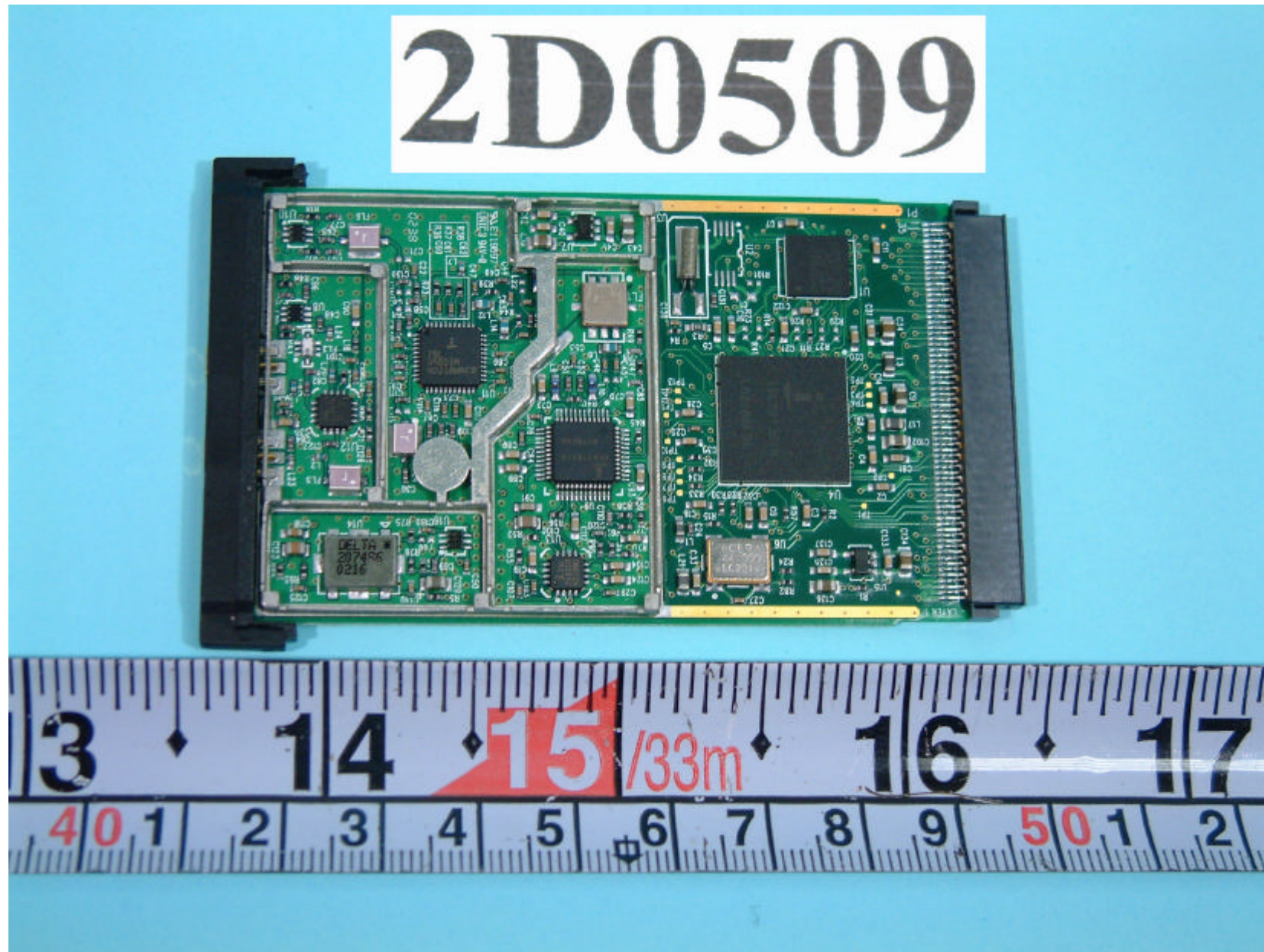
FRONT SIDE OF MAIN BOARD (RF MODULE)
