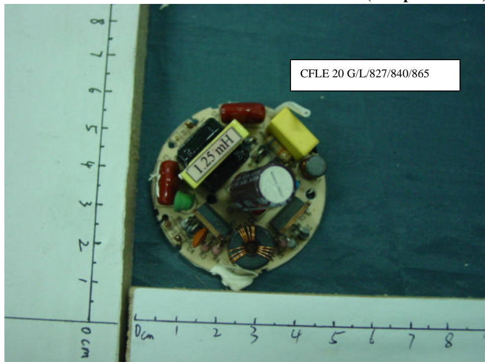
FIGURE 33 Energy Saving Lamp Main Board (Soldered Side)
