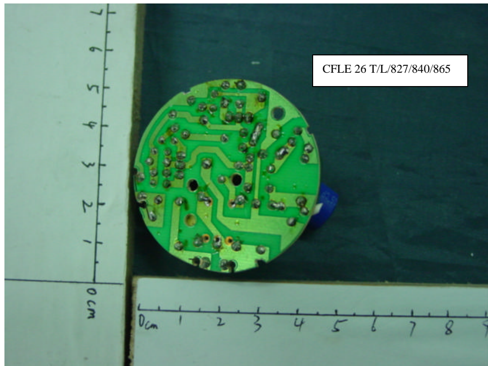
FIGURE 18 Energy Saving Lamp Main Board (Component Side)
