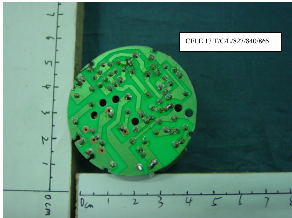
FIGURE 20 Energy Saving Lamp Main Board (Component Side)
