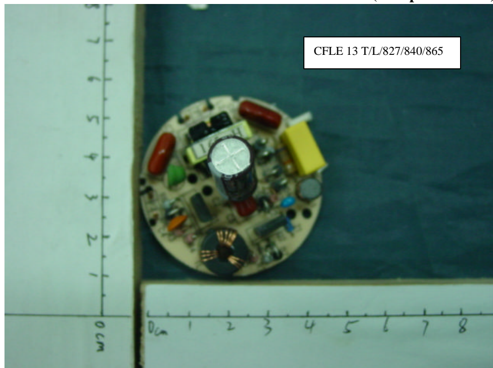
FIGURE 7 Energy Saving Lamp Main Board (Soldered Side)
