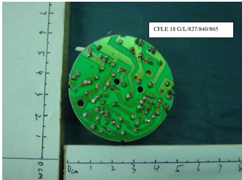
FIGURE 32 Energy Saving Lamp Main Board (Component Side)
