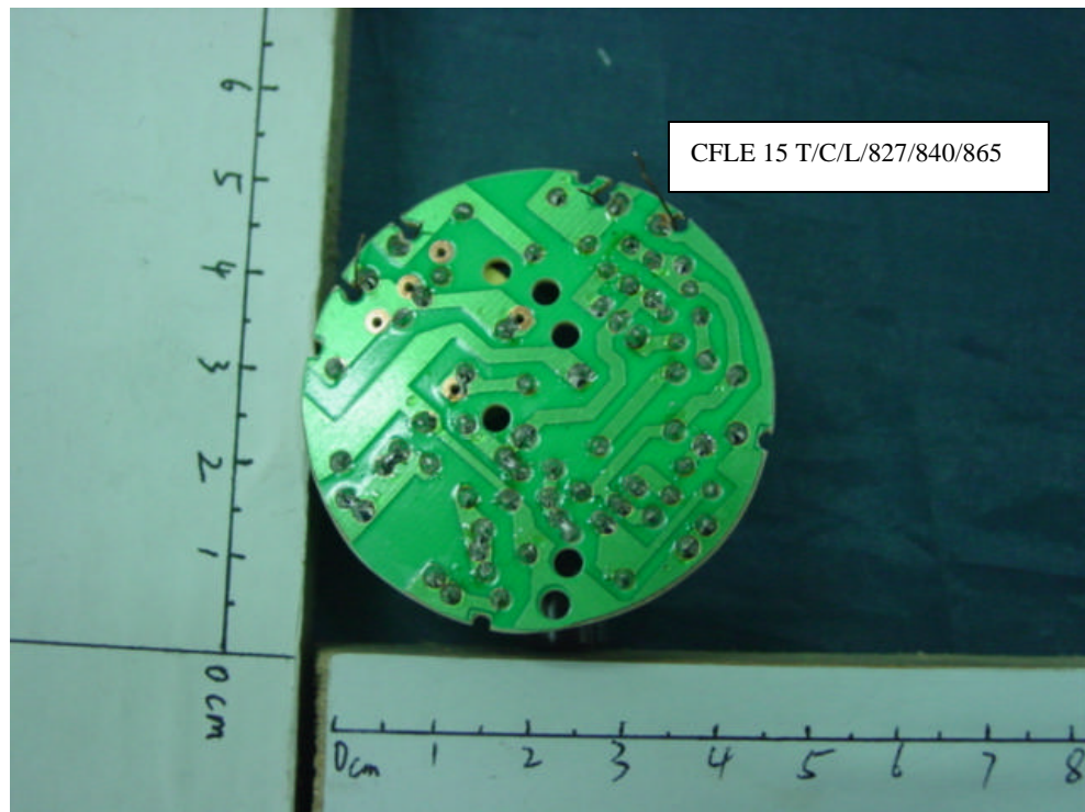
FIGURE 22 Energy Saving Lamp Main Board (Component Side)
