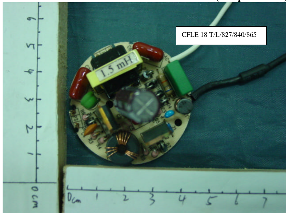
FIGURE 11 Energy Saving Lamp Main Board (Soldered Side)
