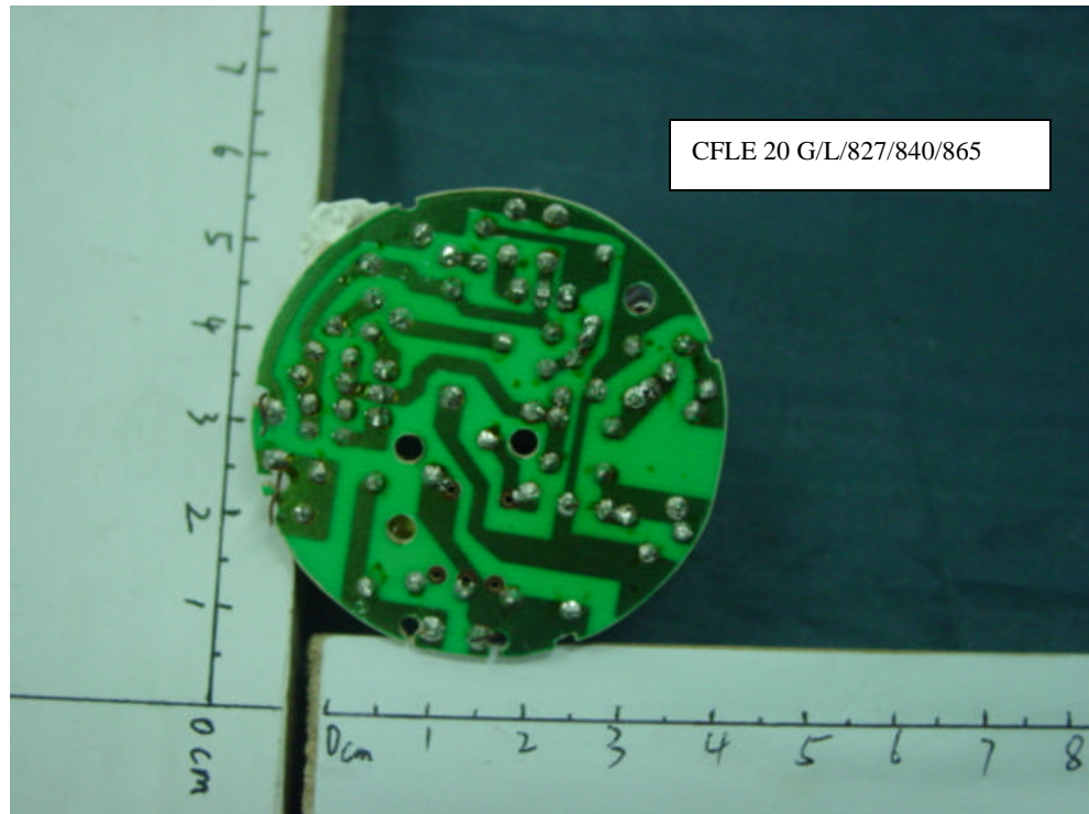
FIGURE 34 Energy Saving Lamp Main Board (Component Side)
