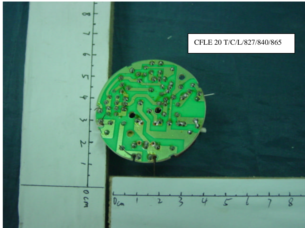
FIGURE 26 Energy Saving Lamp Main Board (Component Side)
