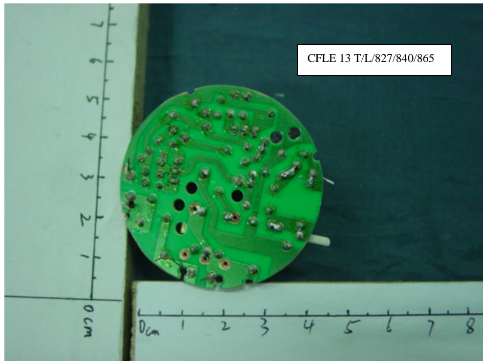
FIGURE 8 Energy Saving Lamp Main Board (Component Side)
