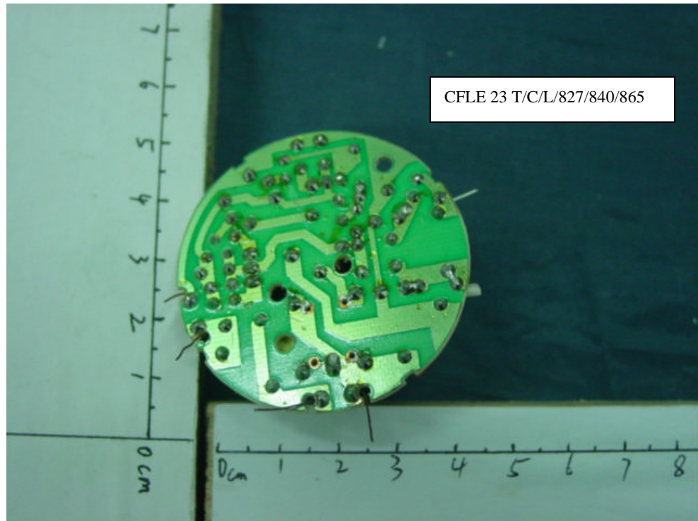
FIGURE 28 Energy Saving Lamp Main Board (Component Side)
