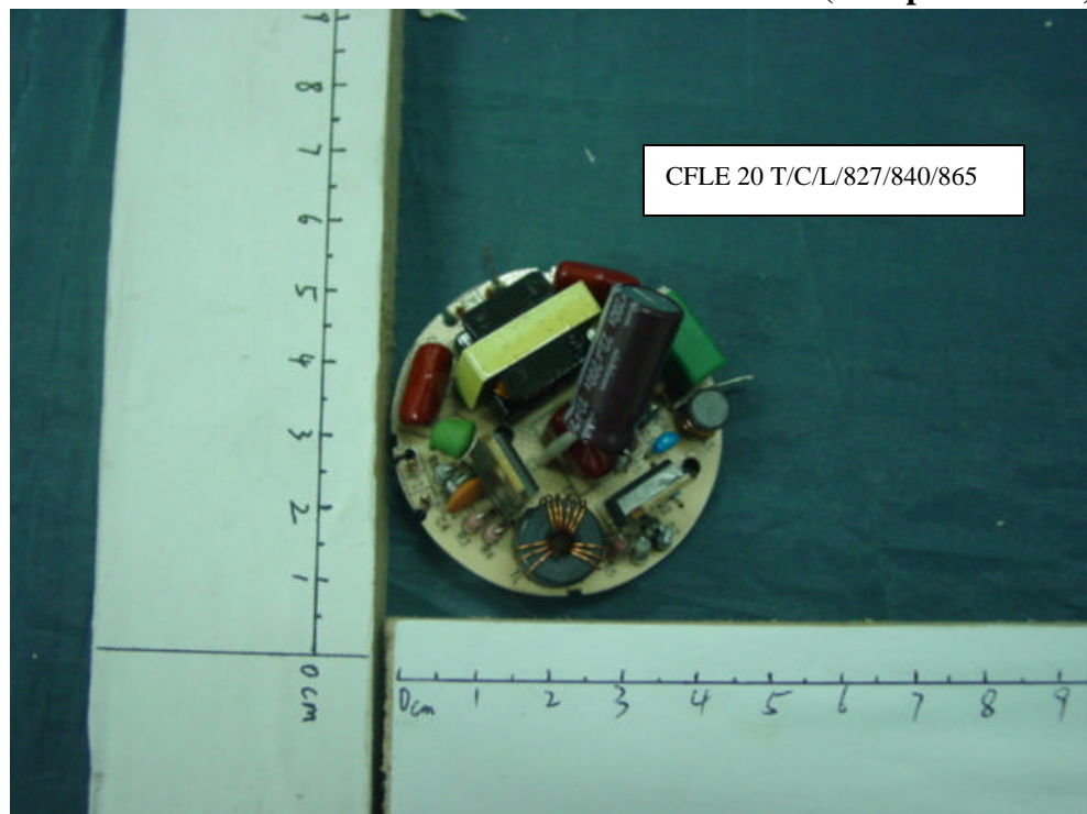
FIGURE 25 Energy Saving Lamp Main Board (Soldered Side)
