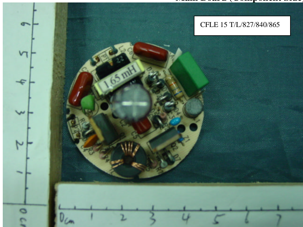
FIGURE 9 Energy Saving Lamp Main Board (Soldered Side)
