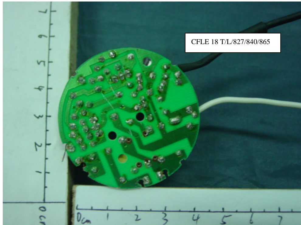
FIGURE 12 Energy Saving Lamp Main Board (Component Side)
