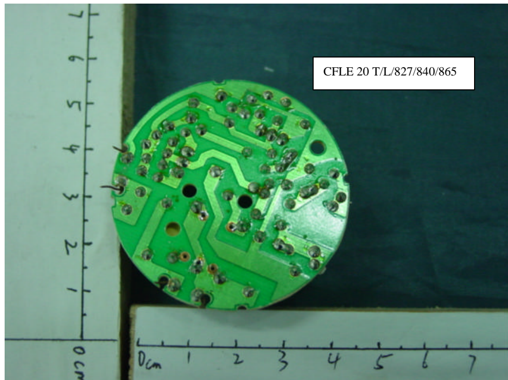
FIGURE 14 Energy Saving Lamp Main Board (Component Side)
