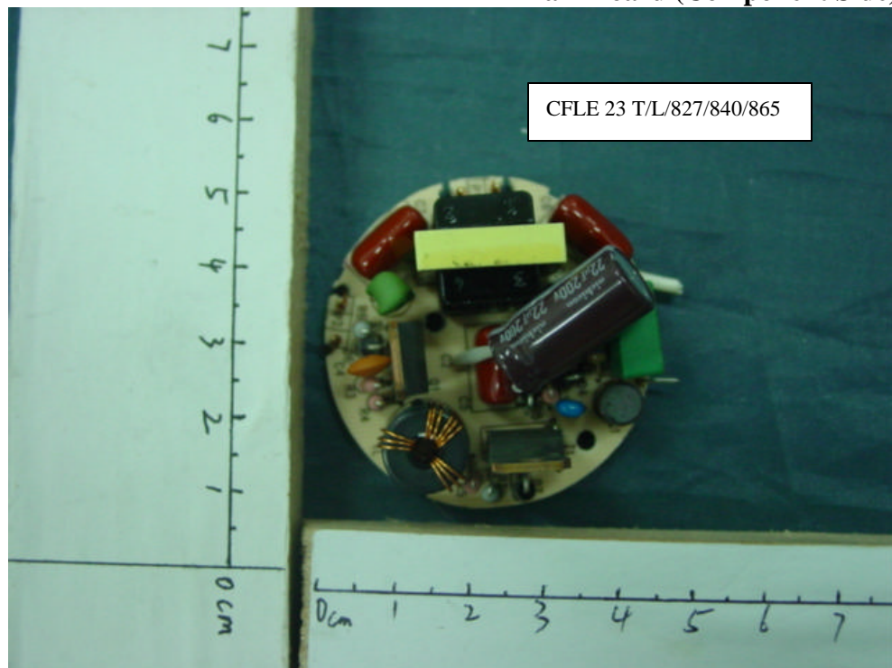
FIGURE 15 Energy Saving Lamp Main Board (Soldered Side)
