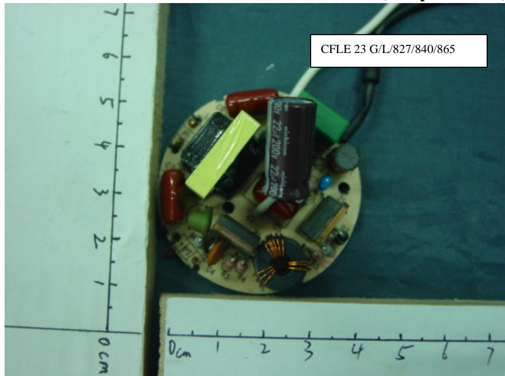
FIGURE 35 Energy Saving Lamp Main Board (Soldered Side)
