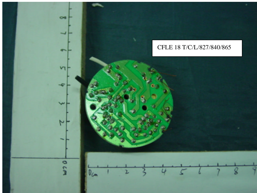
FIGURE 24 Energy Saving Lamp Main Board (Component Side)
