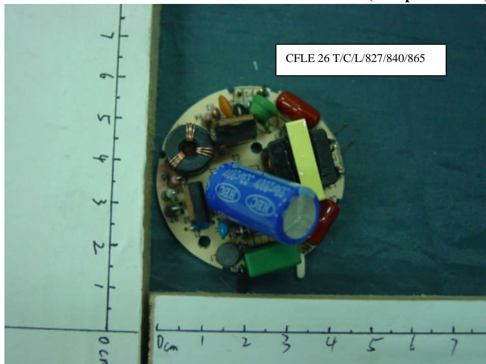
FIGURE 29 Energy Saving Lamp Main Board (Soldered Side)
