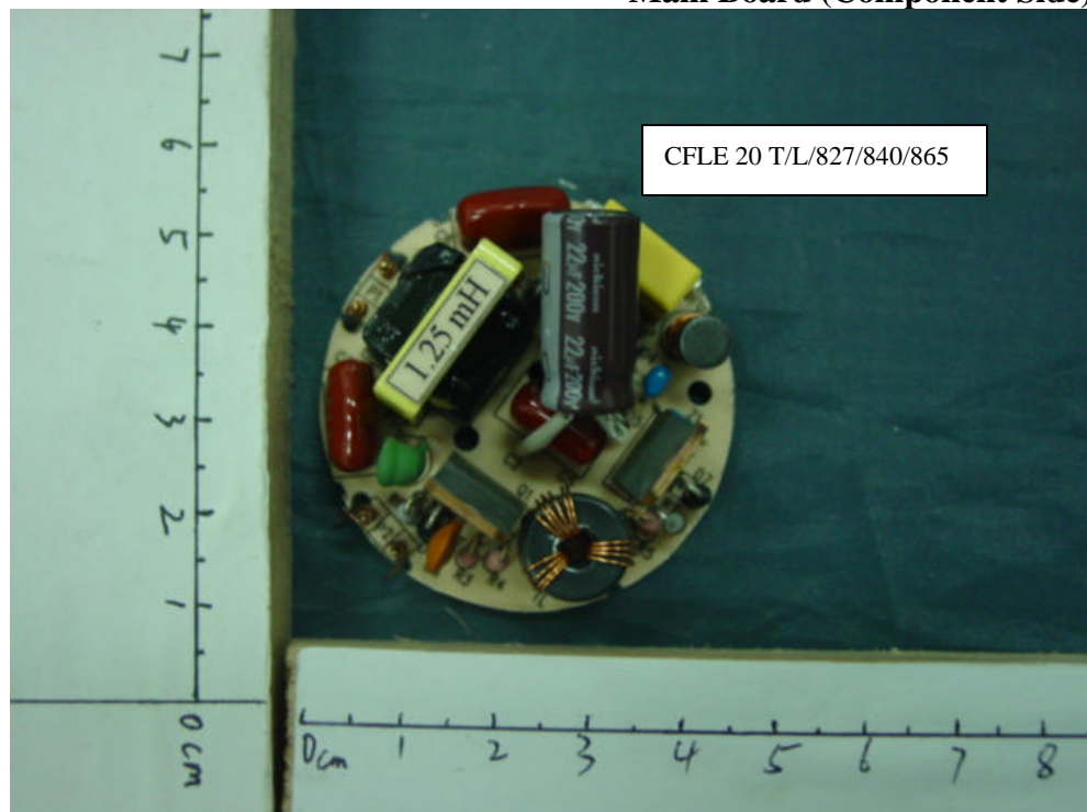
FIGURE 13 Energy Saving Lamp Main Board (Soldered Side)
