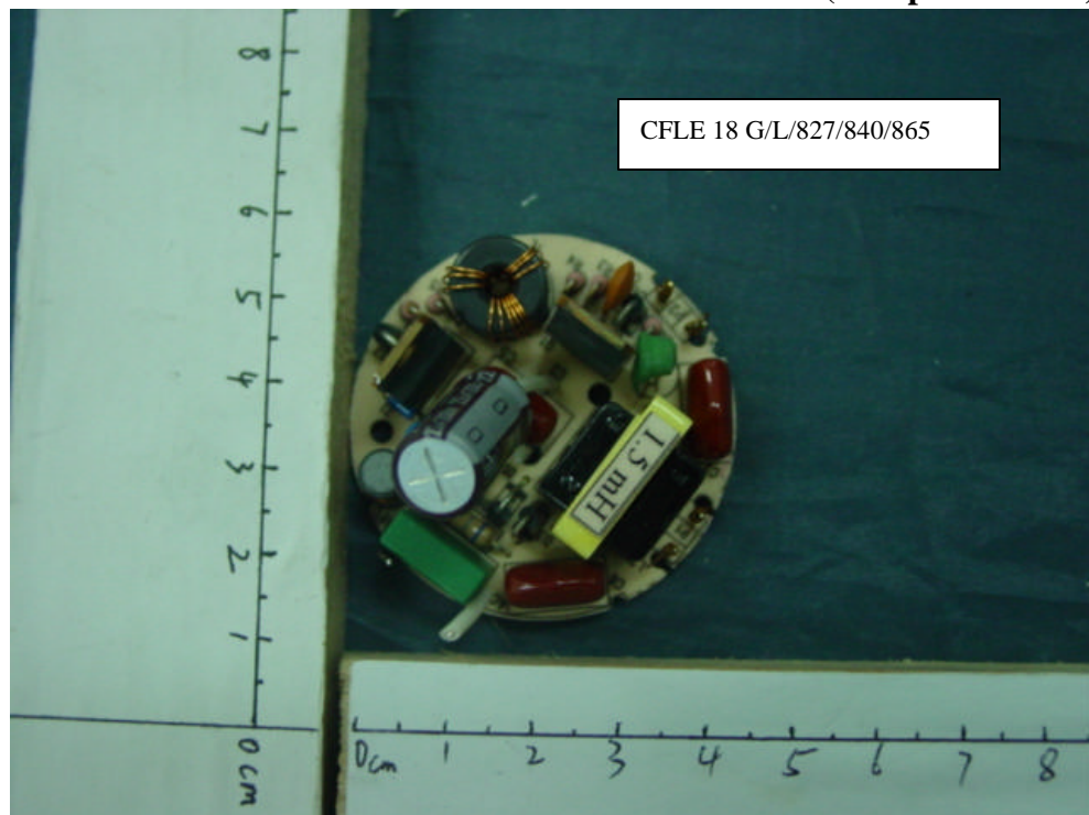
FIGURE 31 Energy Saving Lamp Main Board (Soldered Side)
