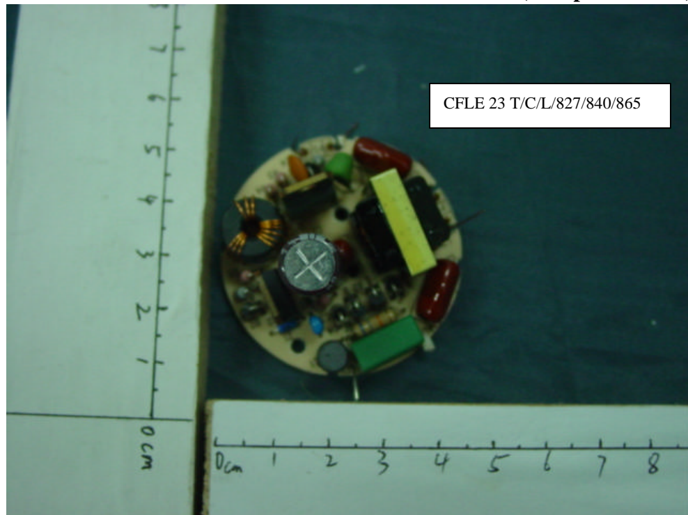
FIGURE 27 Energy Saving Lamp Main Board (Soldered Side)
