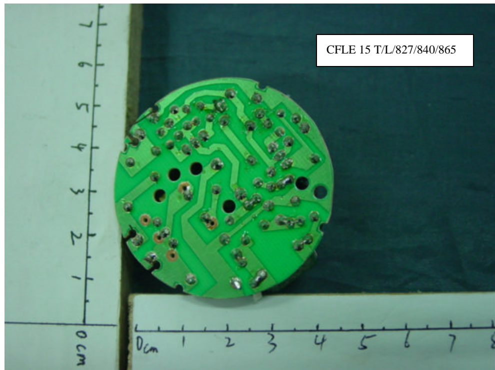
FIGURE 10 Energy Saving Lamp Main Board (Component Side)
