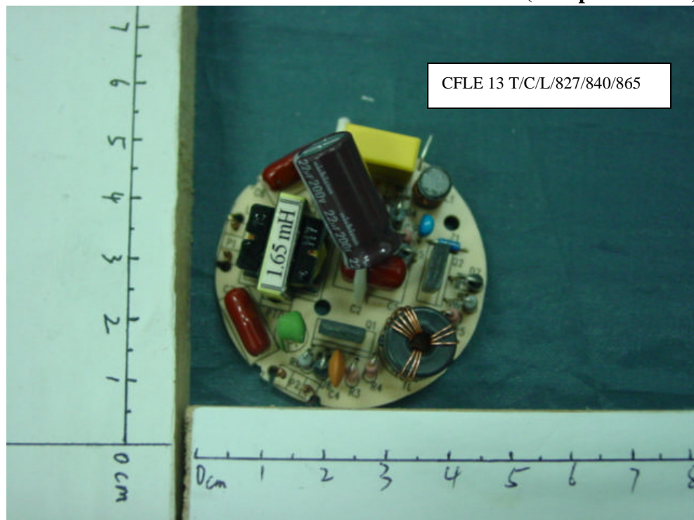
FIGURE 19 Energy Saving Lamp Main Board (Soldered Side)
