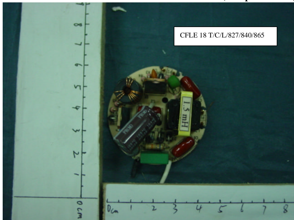
FIGURE 23 Energy Saving Lamp Main Board (Soldered Side)
