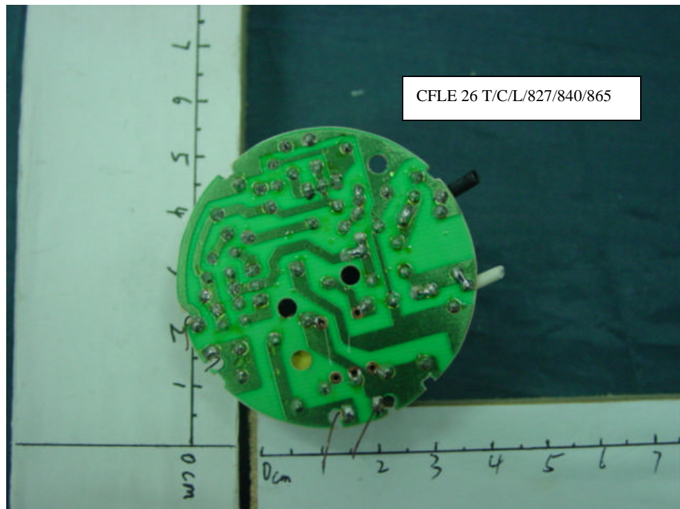
FIGURE 30 Energy Saving Lamp Main Board (Component Side)
