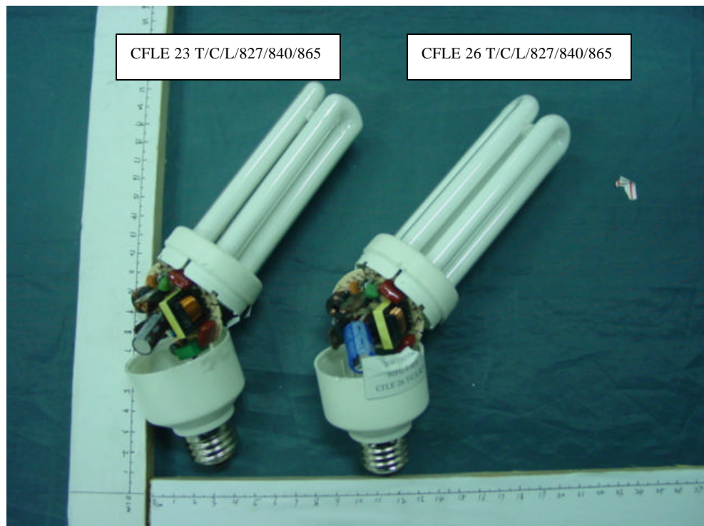
FIGURE 4 Energy Saving Lamp Cover Removed
