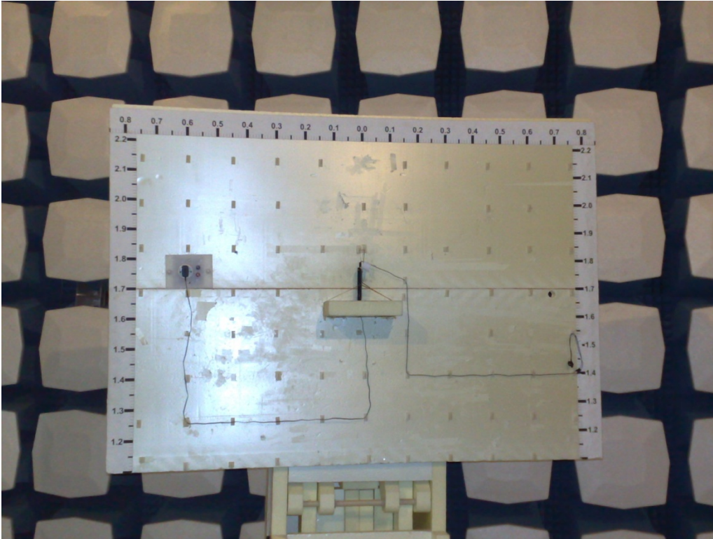
Picture 1. FCC Part 15C Radiated emissions
