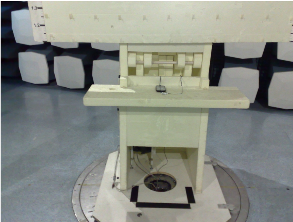
Picture 2. FCC Part 15B Radiated emissions
