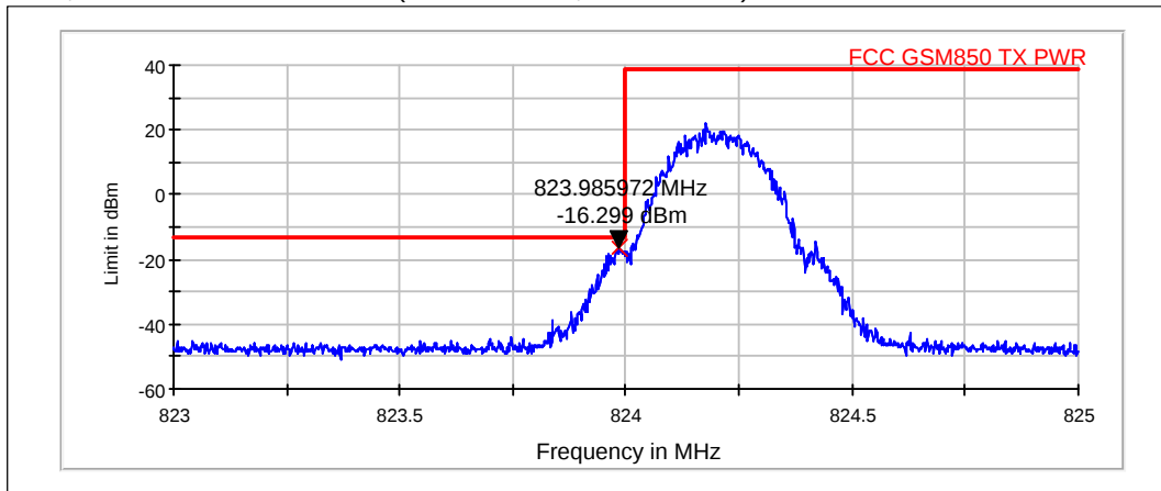
GSM, channel 128 / 824.2 MHz (Peak detector, RBW: 3 kHz)
