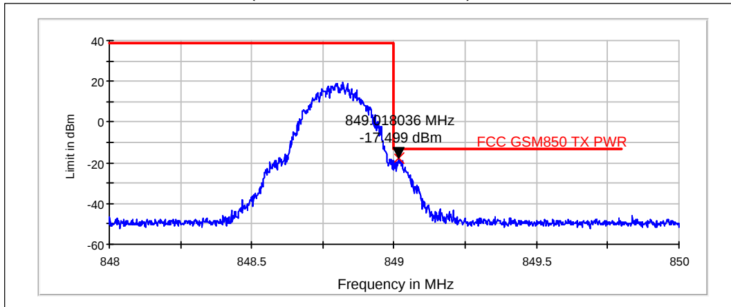
GSM, channel 251 / 848.8 MHz (Peak detector, RBW: 3 kHz)
