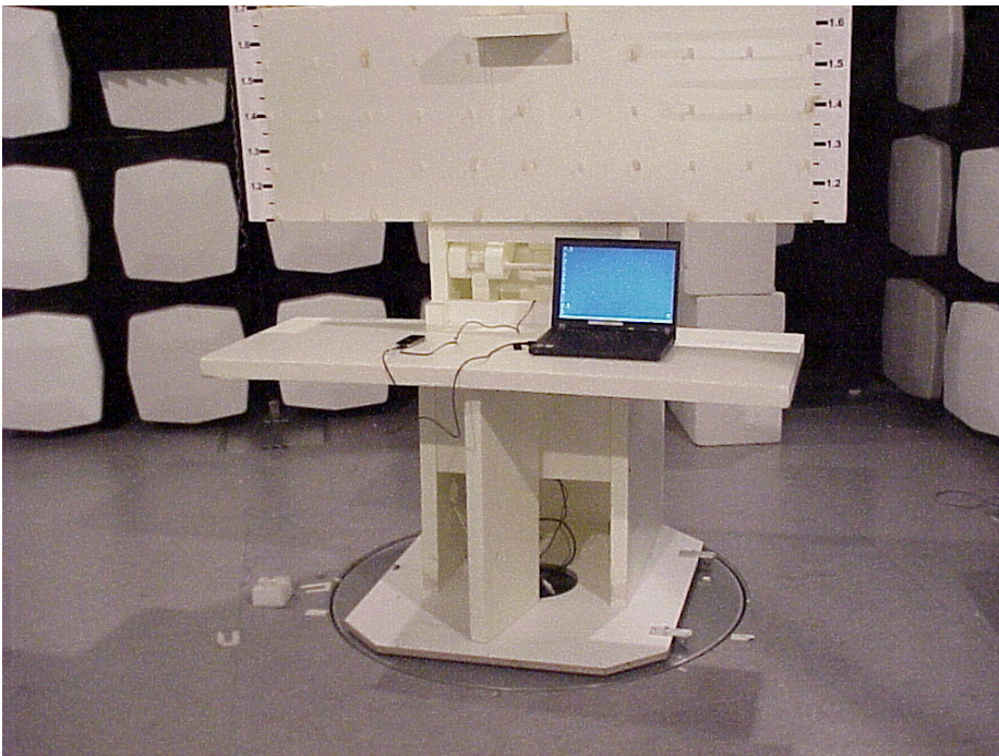
Picture 2 Radiated emission 15B
