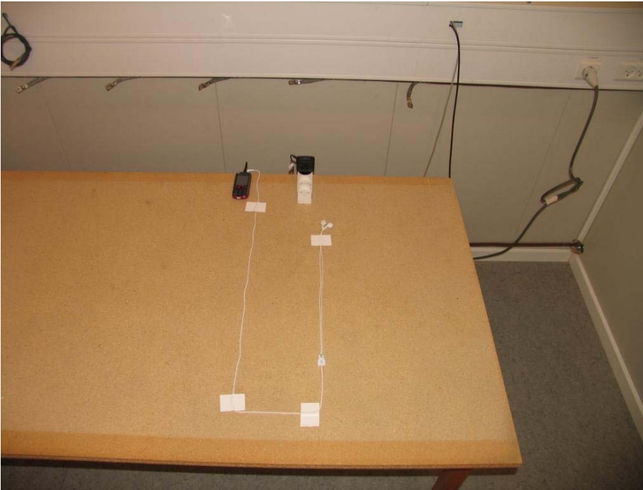
Picture 3 AC powerline conducted emission measurement 15C
