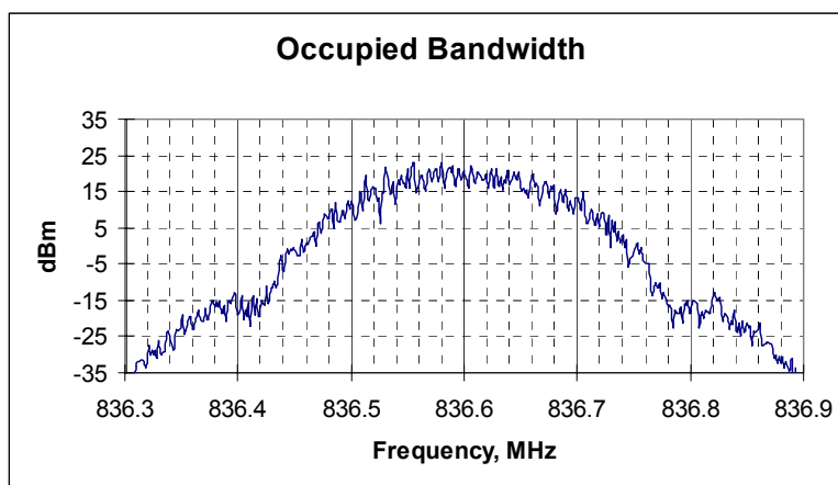
Picture 4. 99% occupied bandwidth, channel 190 3KHz Bw and VBw
