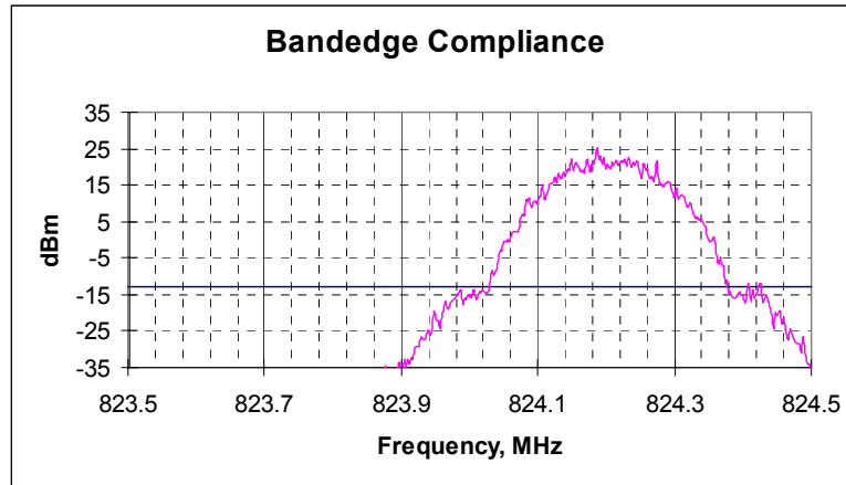
Picture 5. Lower bandedge, channel 128 RBw 3KHz, VBw 3KHz
