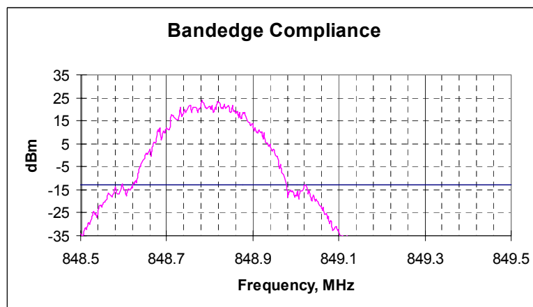
Picture 6. Upper bandedge, channel 251 RBw 3KHz VBw 3KHz
