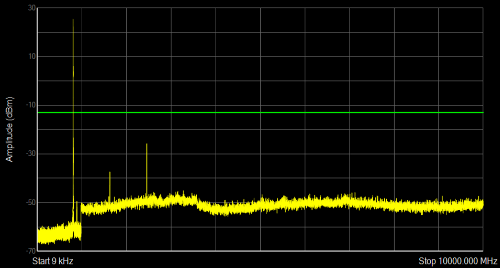
Band5 16QAM BW=1.4MHz Channel=20407 RB Size=1 Position=#0
