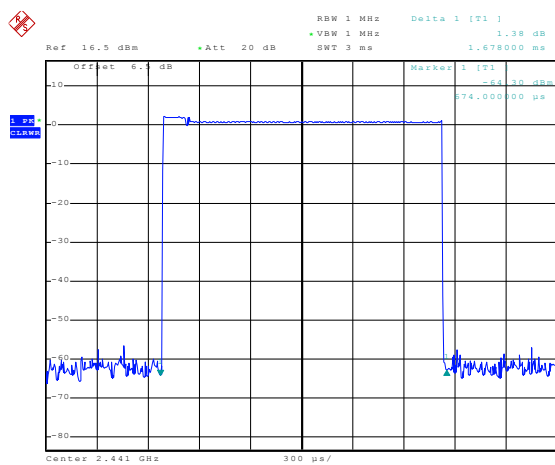
2-DH3
