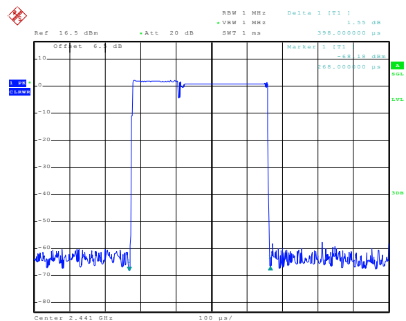
3-DH1
