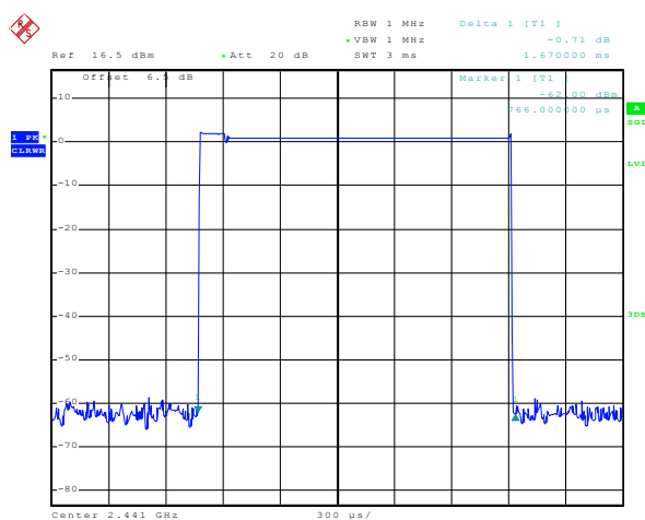
3-DH3
