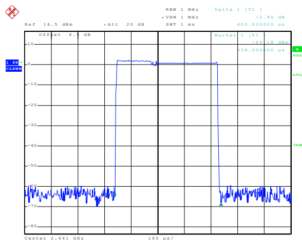
2-DH1
