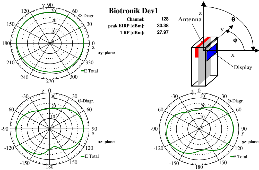
Figure 3: Polar diagrams GSM850 Channel: 128
