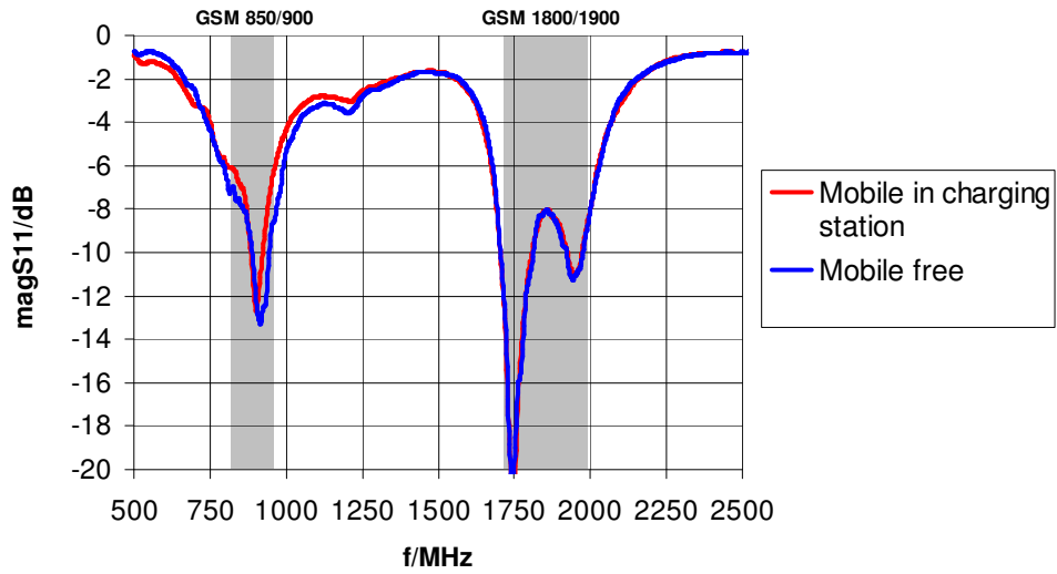
Fig 1: Return loss
