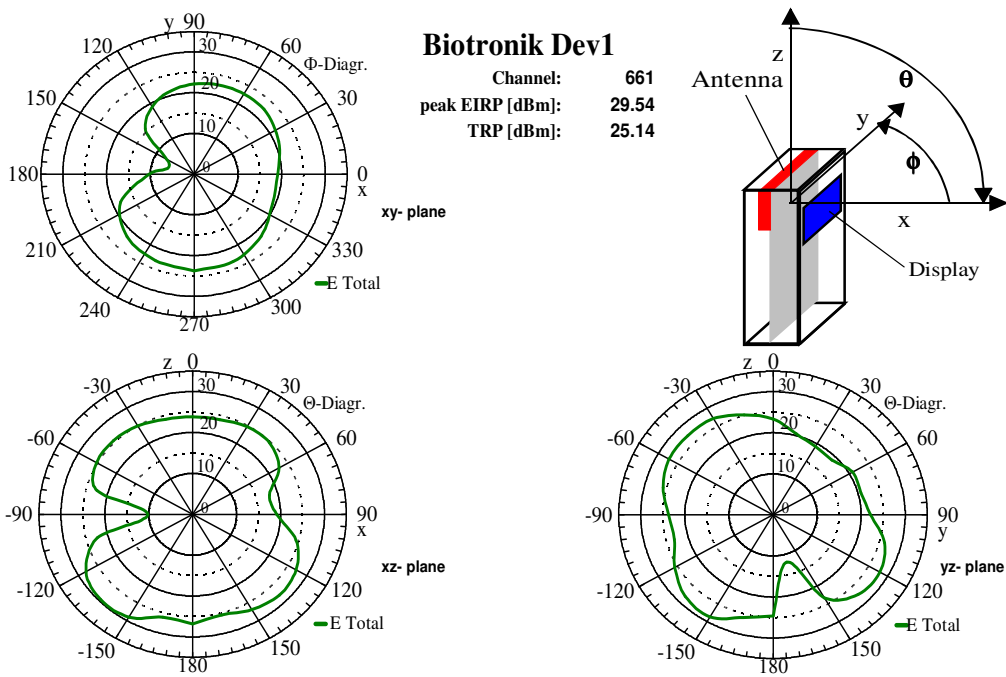
Figure 4: Polar diagrams GSM1900 Channel: 661
