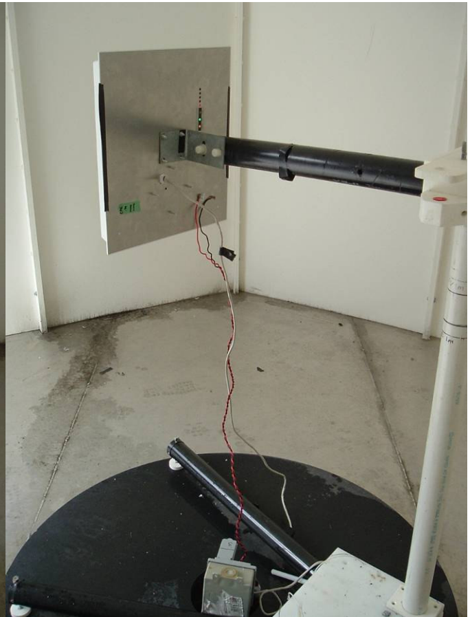
TR-6019 Radiated Emissions
