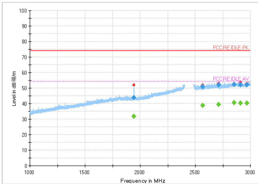
Fig.22 Radiated emission: Ch39, 1GHz~3GHz
