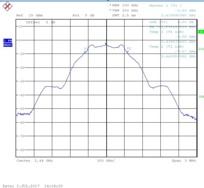
Fig.8 6dB Bandwidth: Ch19
