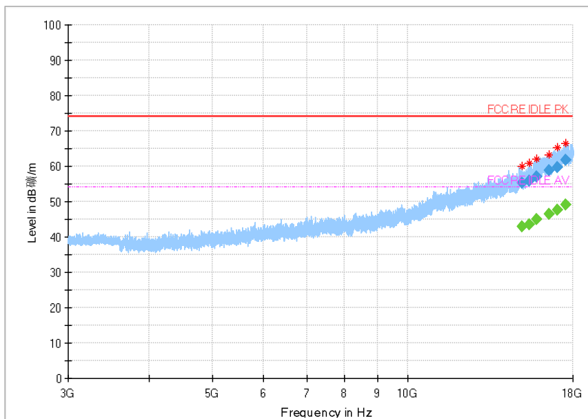
Fig.23 Radiated emission: Ch39, 3GHz~18GHz
