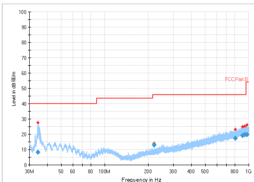
Fig.21 Radiated emission: Ch39, 30MHz~1GHz
