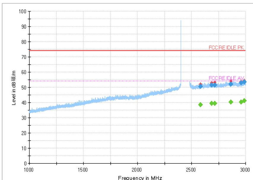
Fig.19 Radiated emission: Ch0, 1GHz~3GHz
