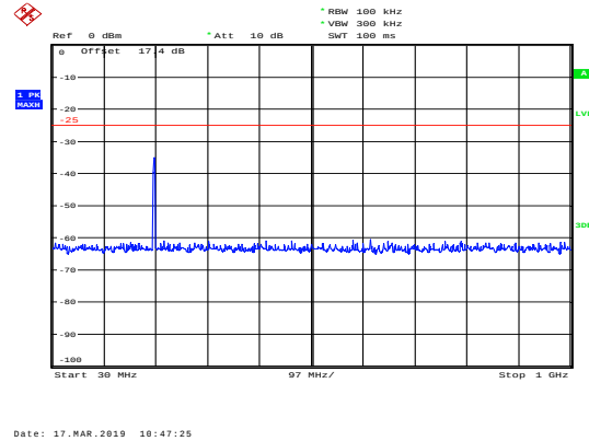
LTE Band 7 5MHz CH-Middle 30MHz~1GHz
