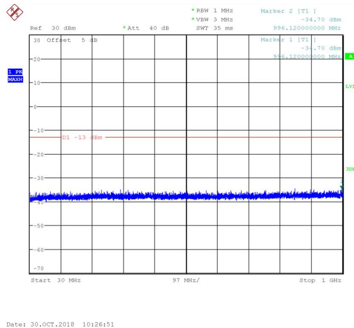
Fig.65 Channel 9538: 30MHz~1GHz
