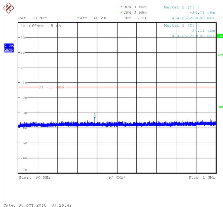
Fig.49 Channel 128: 30MHz~1GHz
