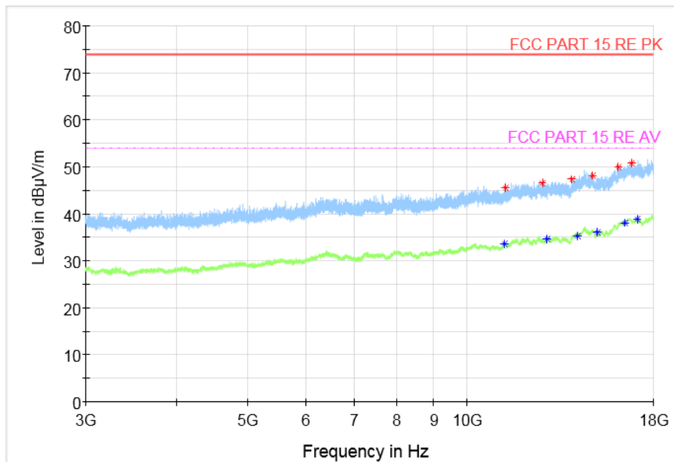
Fig.25 Radiated Spurious Emission (GFSK, Ch39, 3 GHz ~18 GHz)
