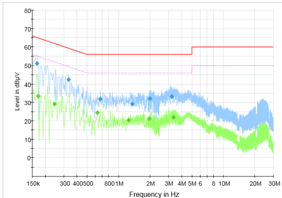
Fig.31 AC Power line Conducted Emission (Traffic)
