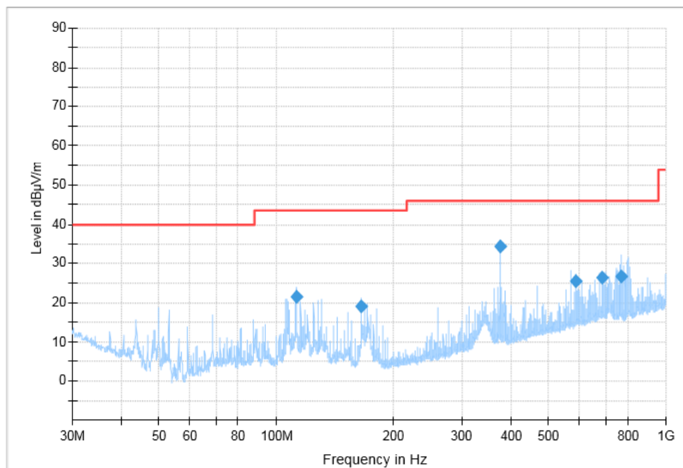
Fig.29 Radiated Spurious Emission (All Channels, 30 MHz-1 GHz)
