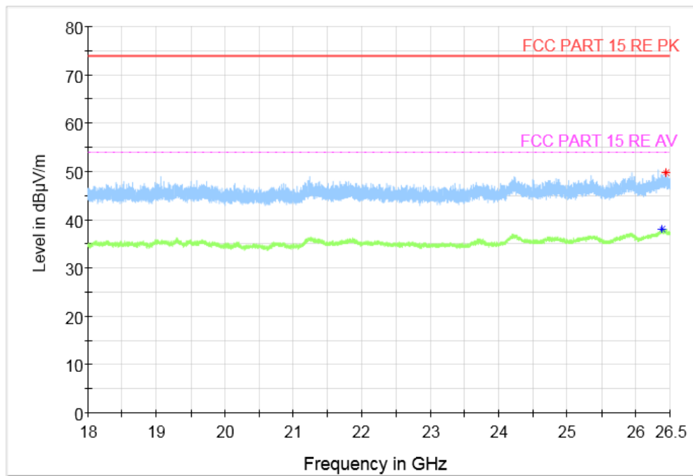
Fig.30 Radiated Spurious Emission (All Channels, 18 GHz-26.5 GHz)
