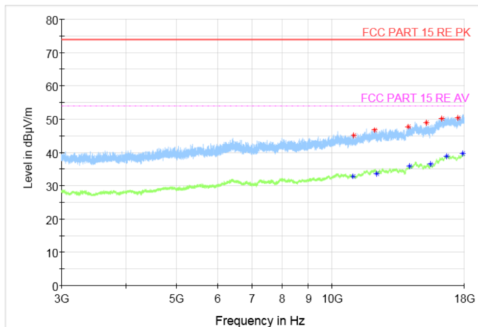
Fig.21 Radiated Spurious Emission (GFSK, Ch0, 3 GHz ~18 GHz)
