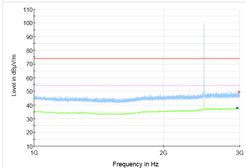
Fig.24 Radiated Spurious Emission (GFSK, Ch39, 1 GHz ~3 GHz)
