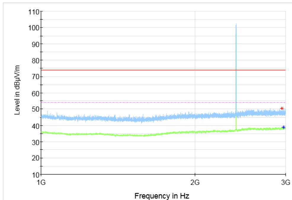
Fig.20 Radiated Spurious Emission (GFSK, Ch0, 1 GHz ~3 GHz)
