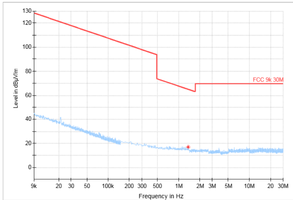
Fig.28 Radiated Spurious Emission (All Channels, 9 kHz-30 MHz)
