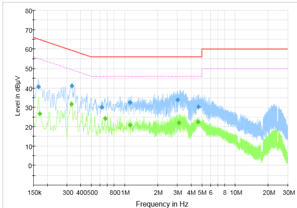
Fig.32 AC Power line Conducted Emission (Idle)
