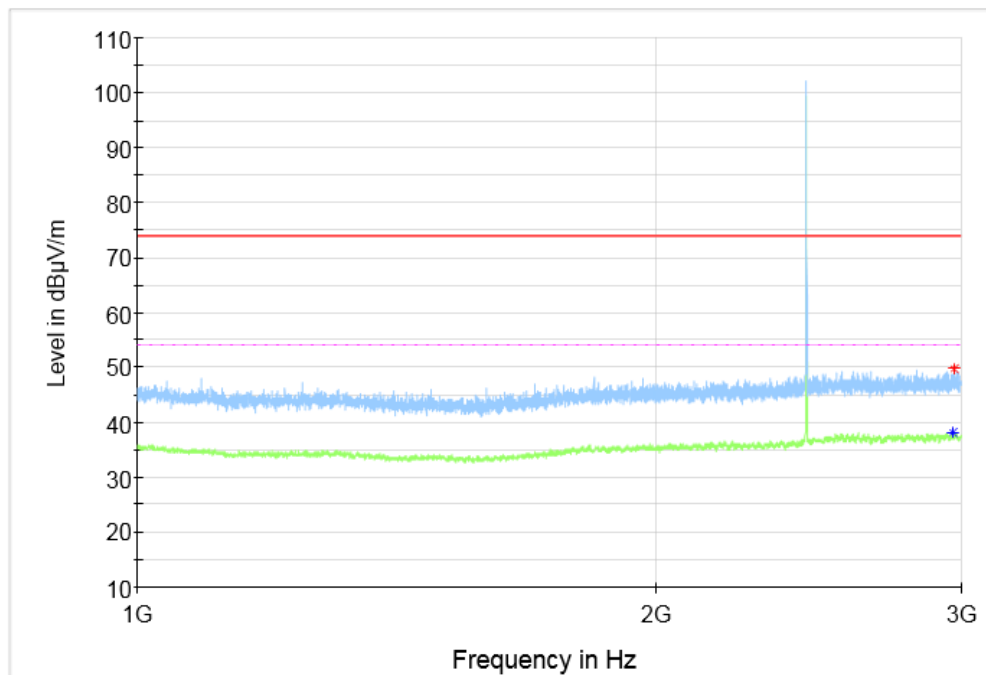
Fig.22 Radiated Spurious Emission (GFSK, Ch19, 1 GHz ~3 GHz)
