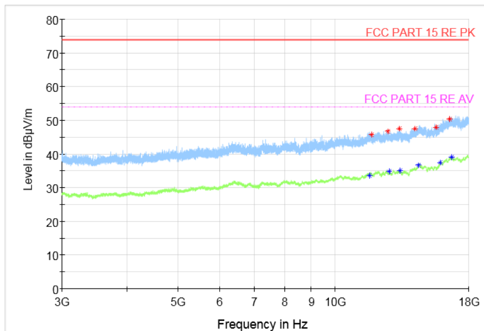
Fig.23 Radiated Spurious Emission (GFSK, Ch19, 3 GHz ~18 GHz)
