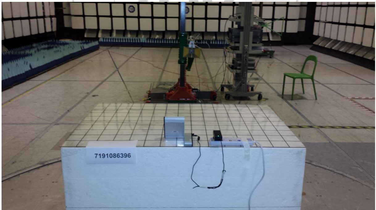
Protection of Aeronautical Radio Navigation Satellite Service Test Setup (Rear View)
