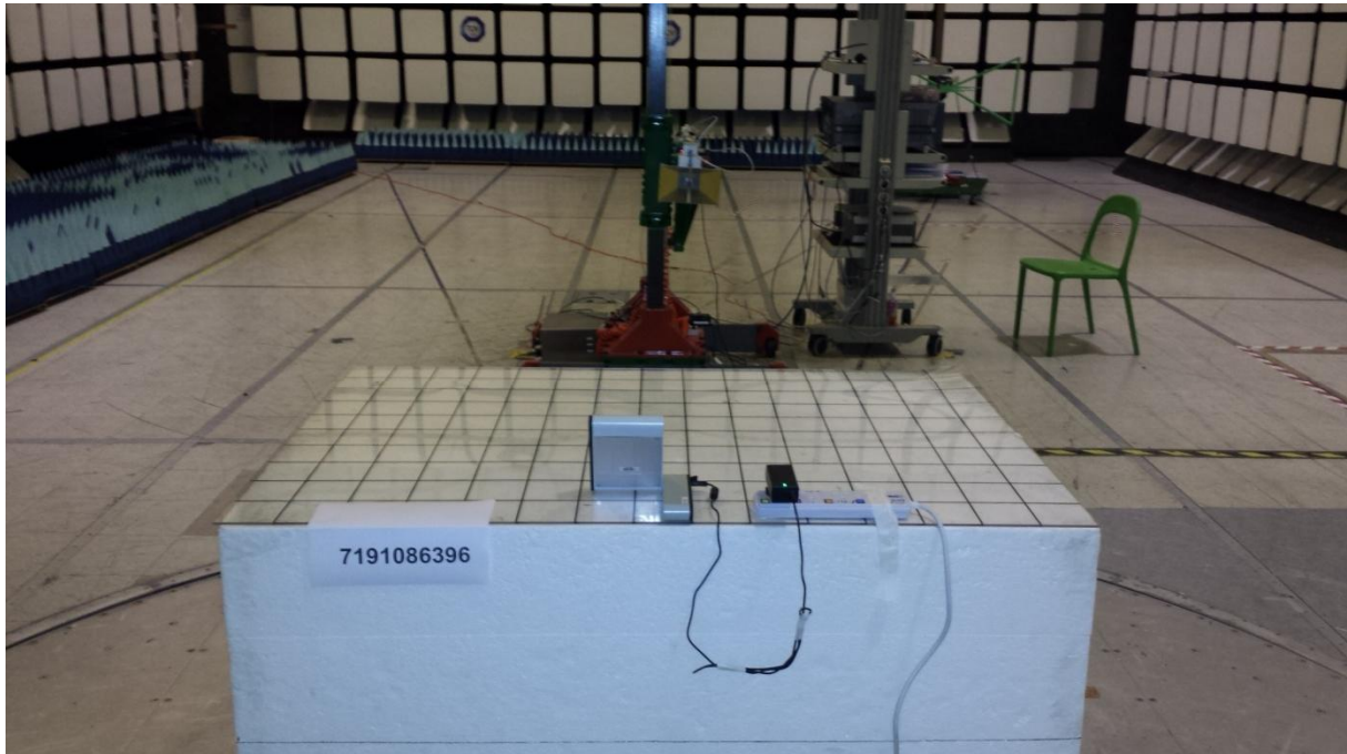
Radiated Spurious Emissions Test Setup (Front View)
