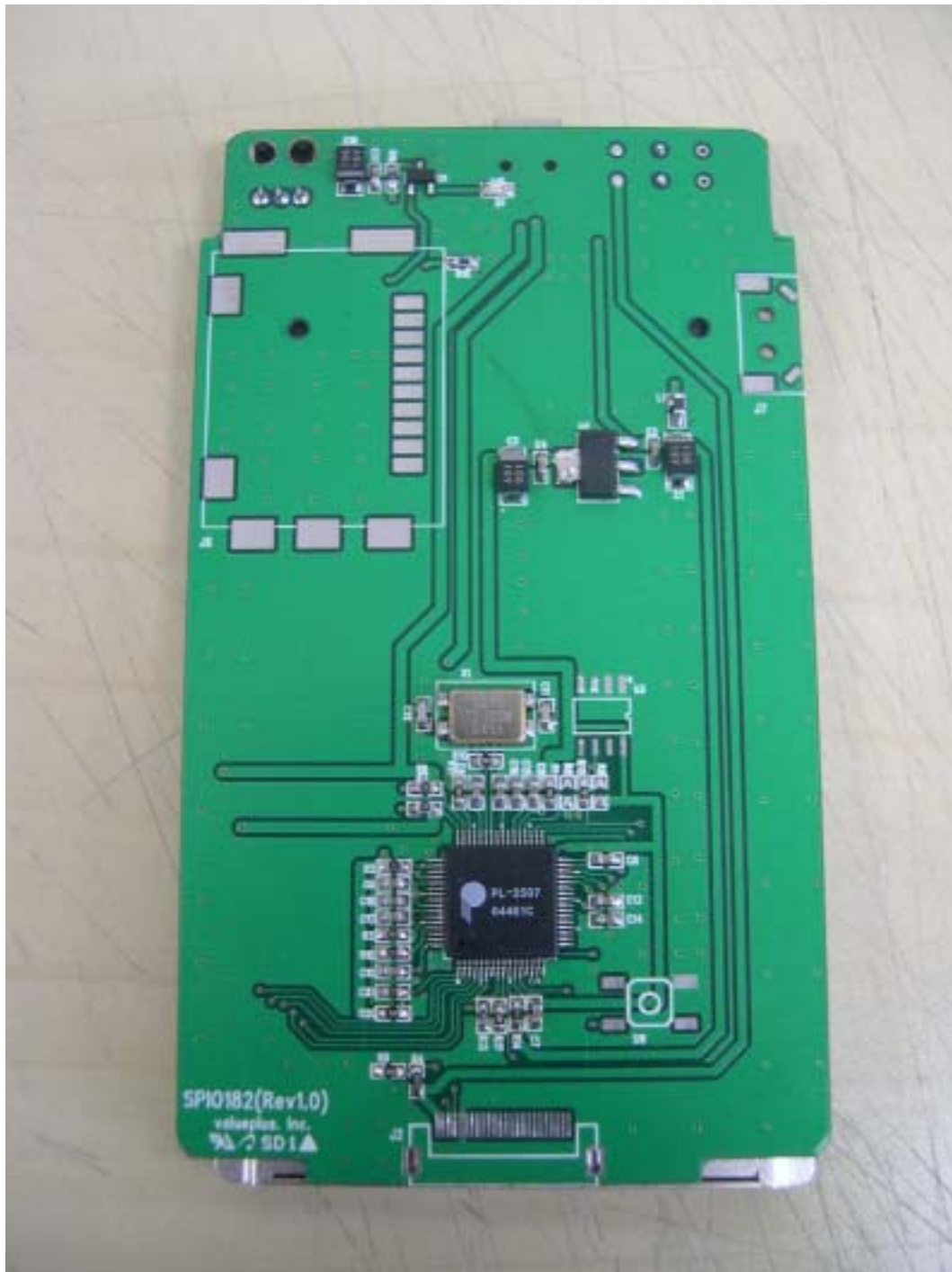
<REAR VIEW OF MAIN BOARD>
