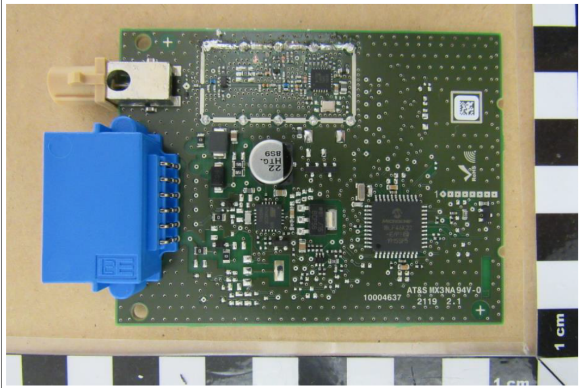
PCB Top View without Shielding
