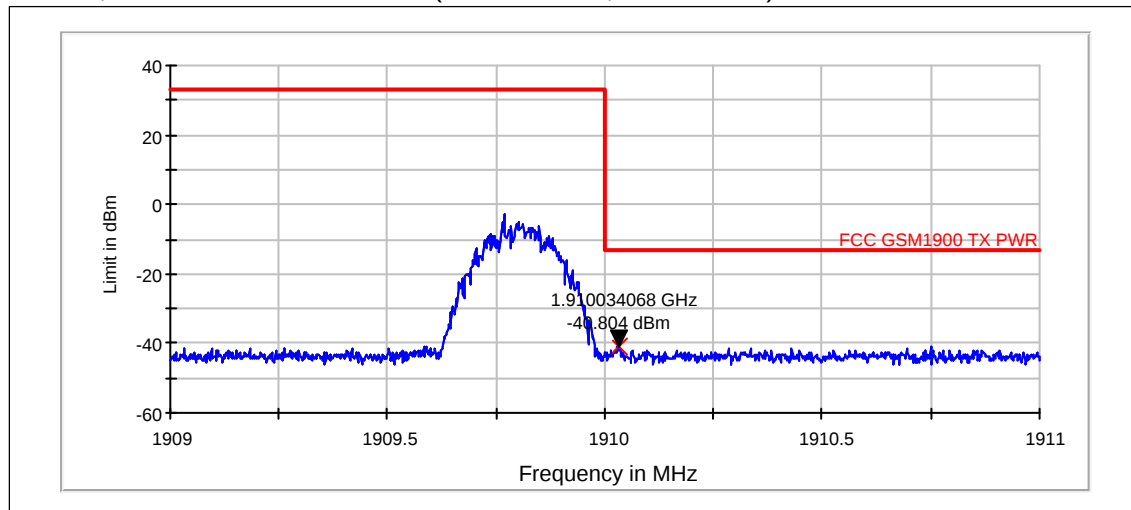
EGPRS, channel 810 / 1909.8 MHz (Peak detector, RBW: 3 kHz)
