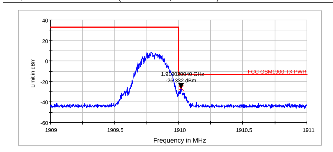
GSM, channel 810 / 1909.8 MHz (Peak detector, RBW: 3 kHz)
