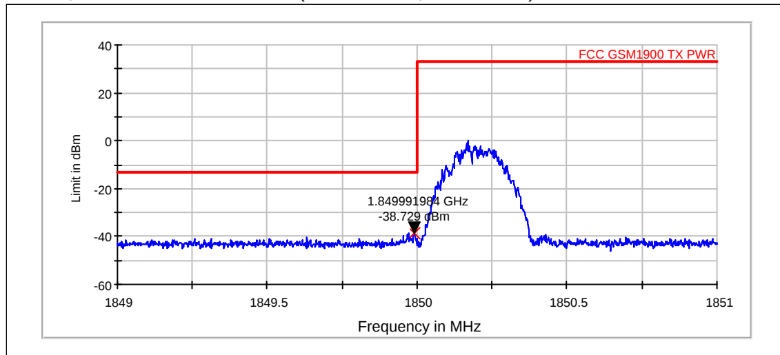
EGPRS, channel 512 / 1850.2 MHz (Peak detector, RBW: 3 kHz)
