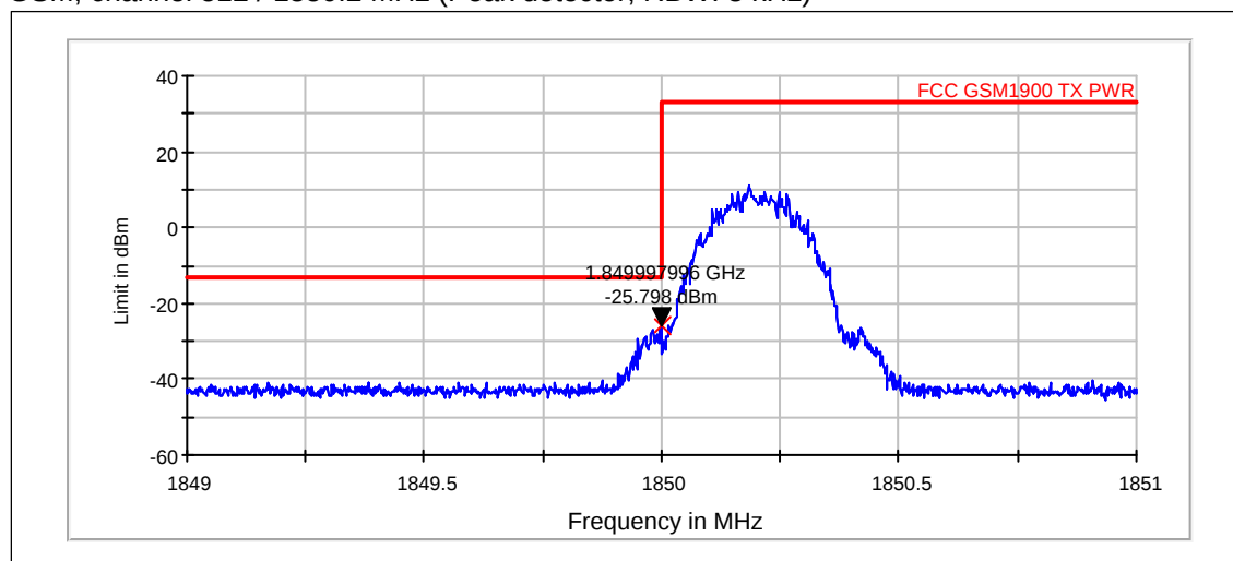
GSM, channel 512 / 1850.2 MHz (Peak detector, RBW: 3 kHz)
