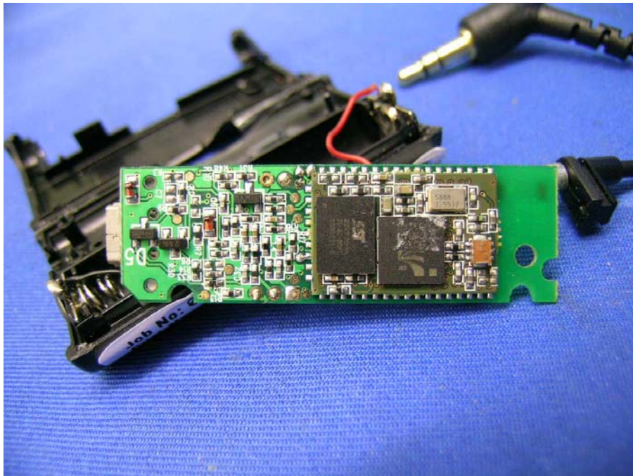
Dongle Main PCB comp side
