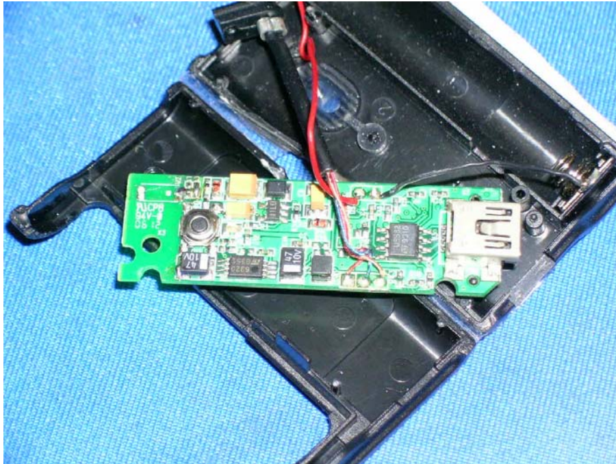
Dongle Main PCB solder side
