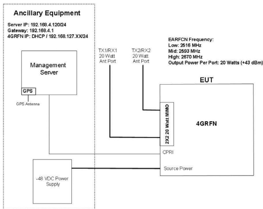
Figure 5-1. Test Setup
