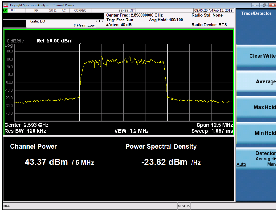
Plot 7-53. Maximum Conducted Power (Band 41 - 5.0MHz 16-QAM – Mid Channel)
