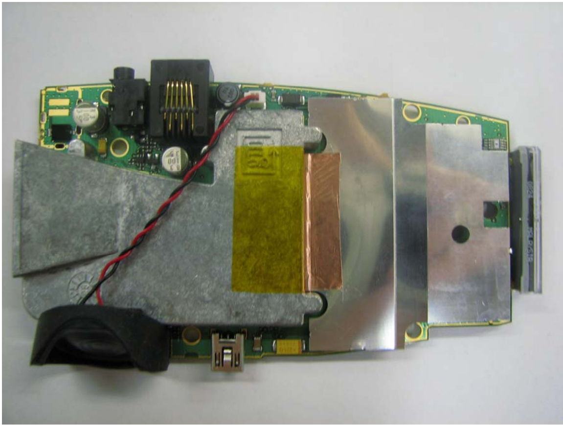
New board with shield over main circuit
