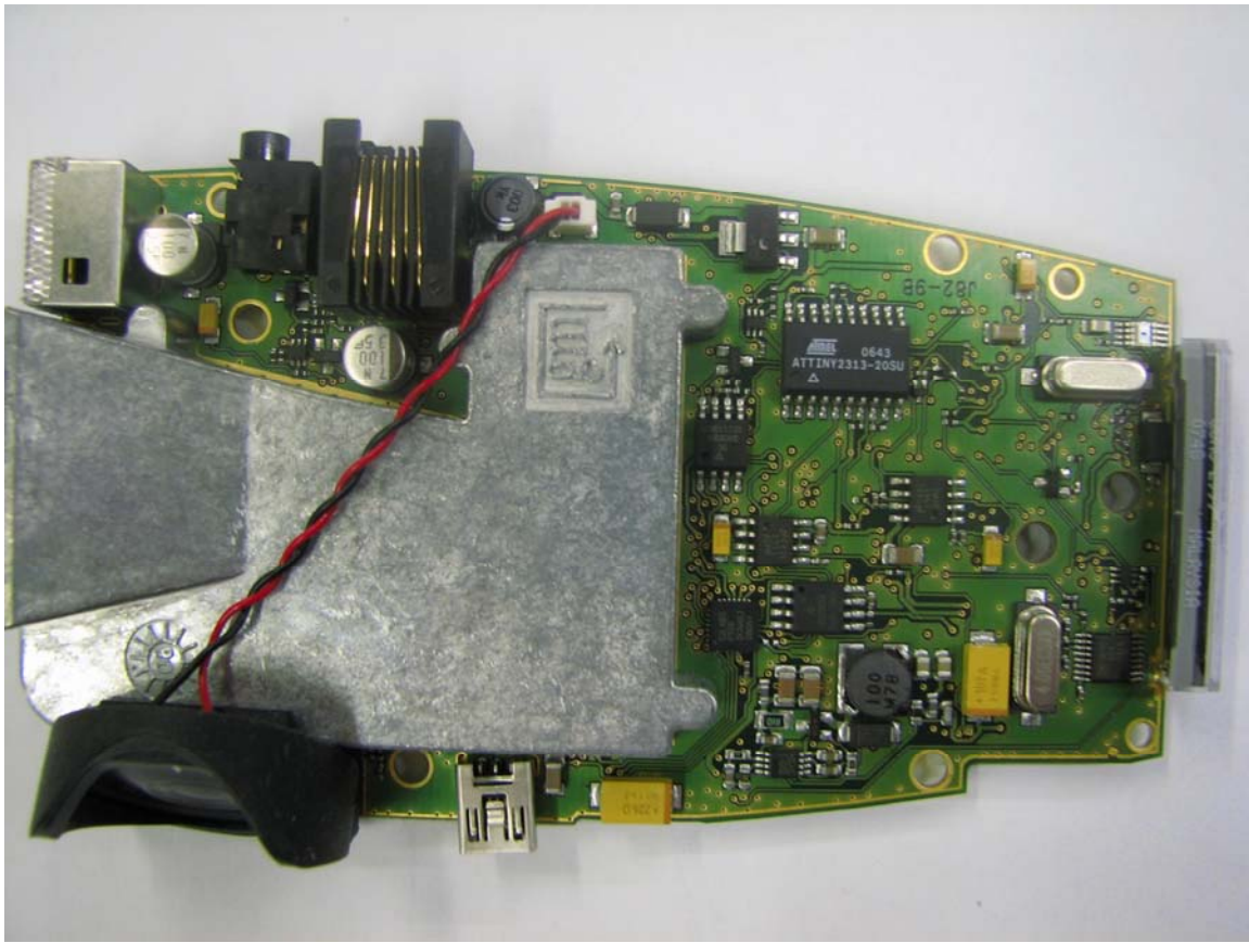
Current Board (old GPS layout)
