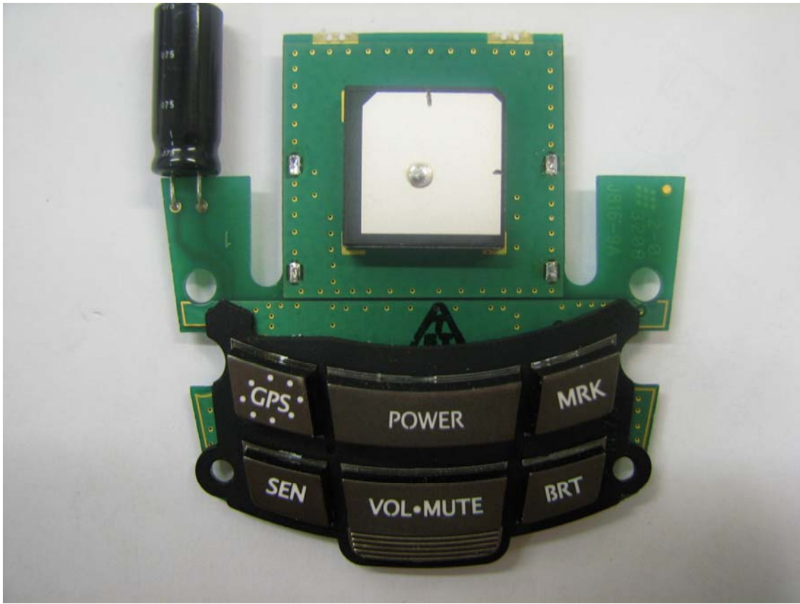
New GPS layout board
