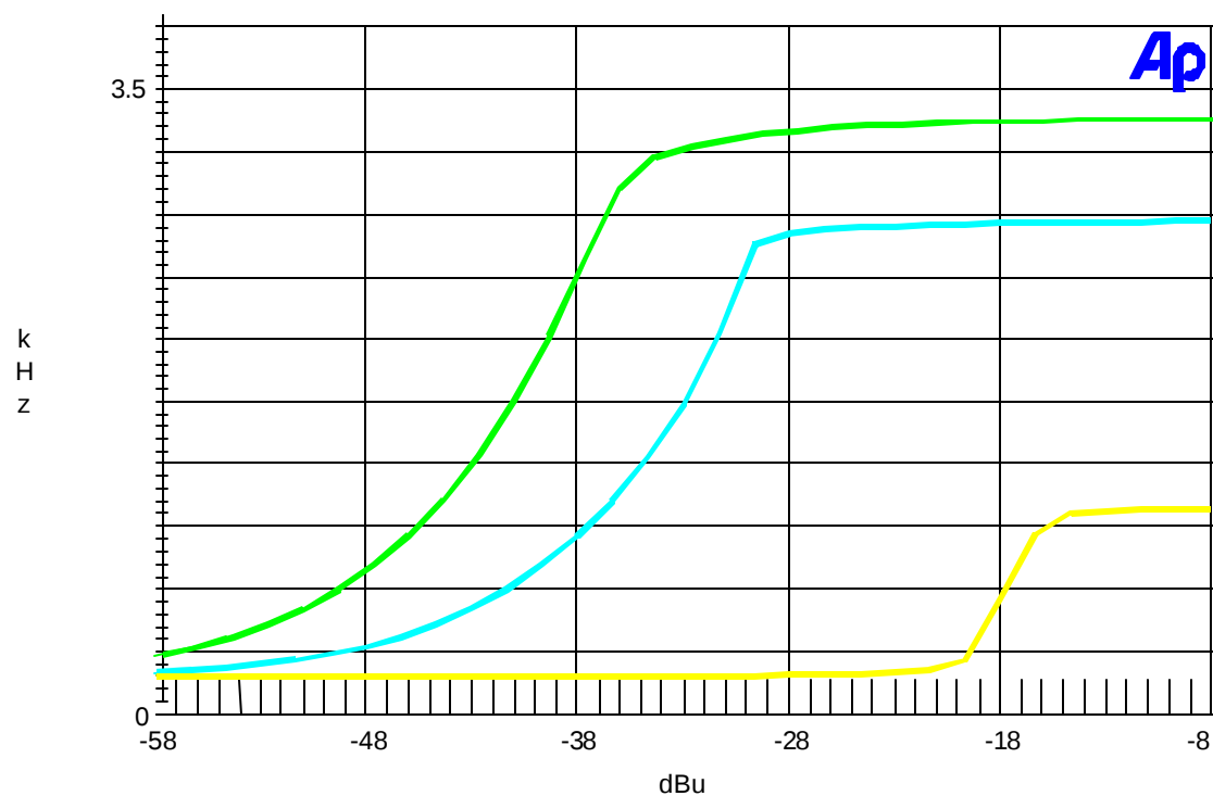
Modulation Limiting Plot: 2.5KHz, 1KHz, 300Hz
