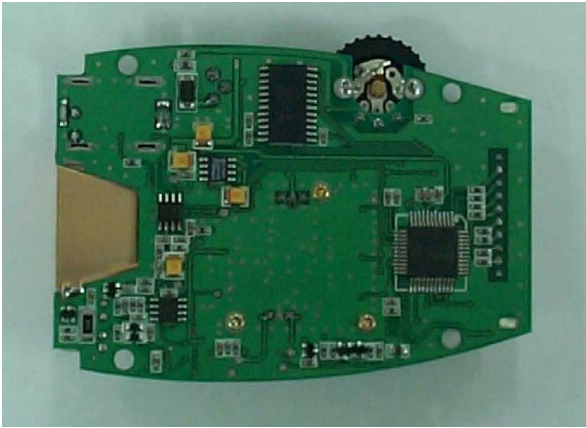
Internal Bottom
