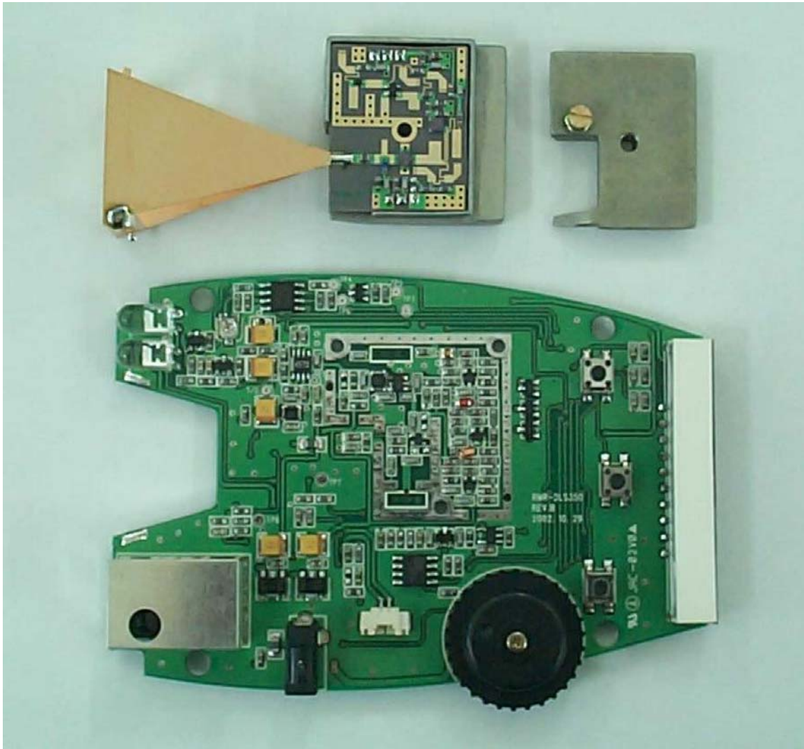
Internal PWBs
