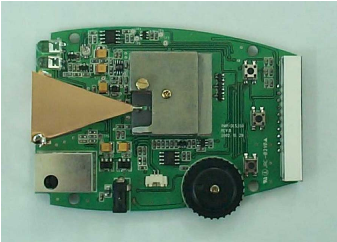
Internal Assembly
