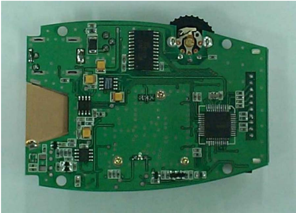
Internal Bottom
