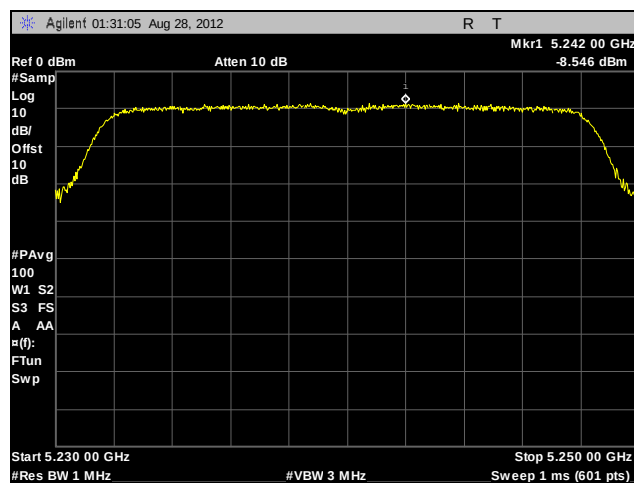
Plot 198. Peak Power Spectral Density, 802.11a, High Channel, Port C, Panel Antenna
