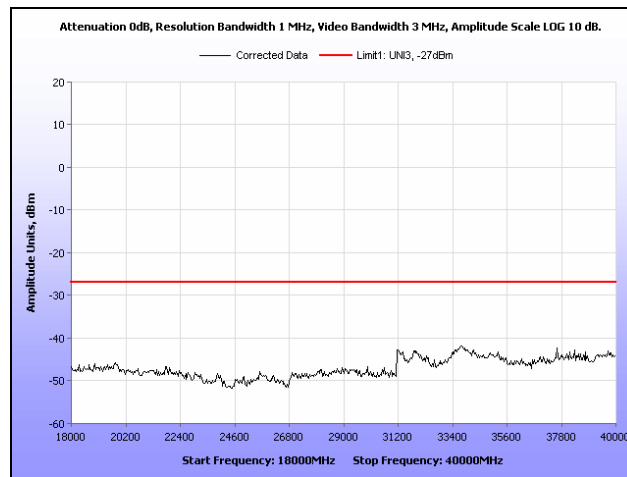
Plot 397. Radiated Spurious Emissions, 802.11n 40 MHz, Low Channel, 18 GHz – 40 GHz, 8.25 dBi Omni Antenna
