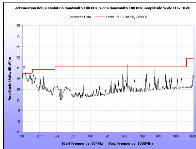
Plot 541. Restricted Band, 802.11n 40 MHz, Low Channel, Low Gain Omni Antenna, 30 MHz – 1 GHz
