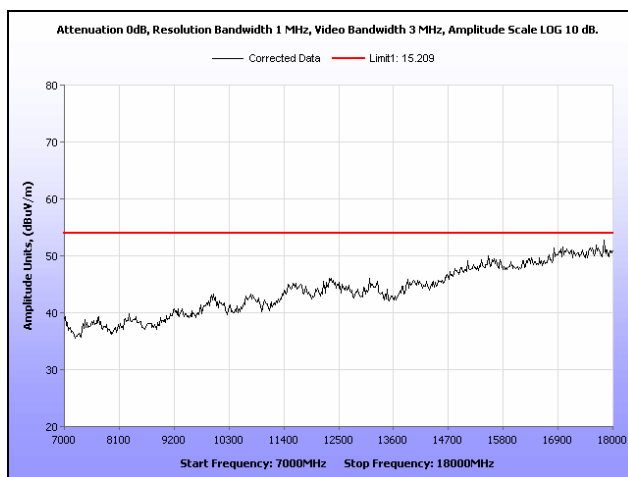
Plot 474. Restricted Band, 802.11a, Mid Channel, Omni Antenna, 7 GHz – 18 GHz
