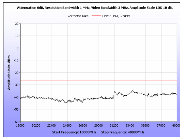
Plot 361. Radiated Spurious Emissions, 802.11n 40 MHz, Low Channel, 18 GHz – 40 GHz, 10.7 dBi Panel Antenna
