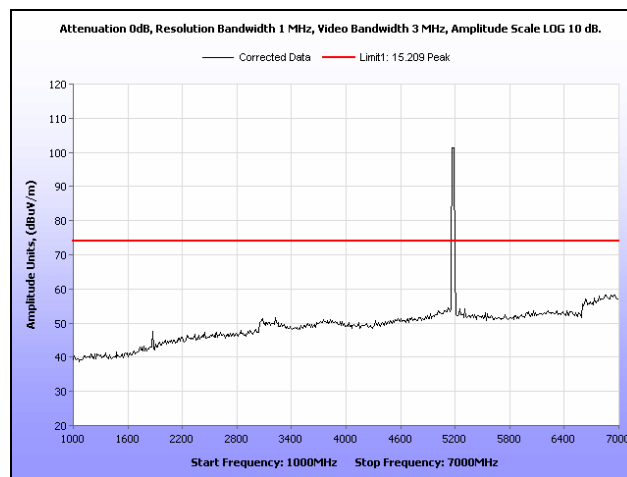
Plot 468. Restricted Band, 802.11a, Low Channel, Omni Antenna, 1 GHz – 7 GHz, Peak
