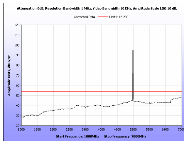
Plot 482. Restricted Band, 802.11n 20 MHz, Low Channel, Omni Antenna, 1 GHz – 7 GHz, Average
