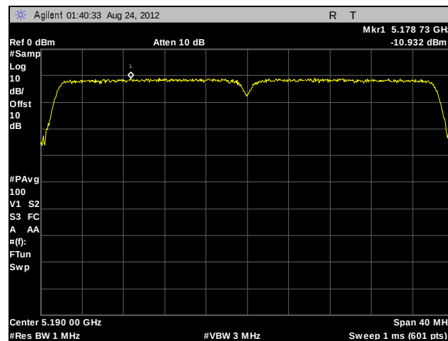
Plot 181. Peak Power Spectral Density, 802.11n 40 MHz, Low Channel, Port A, Omni Antenna
