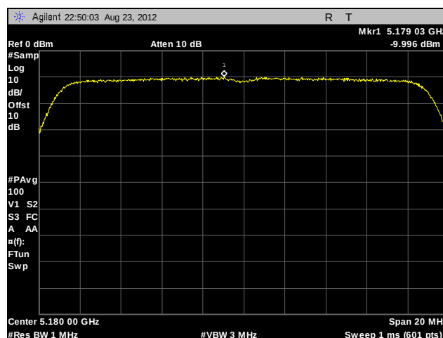
Plot 174. Peak Power Spectral Density, 802.11n 20 MHz, Low Channel, Port C, Omni Antenna
