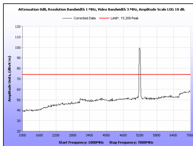
Plot 588. Restricted Band, 802.11n 40 MHz, Low Channel, Panel Antenna, 1 GHz – 7 GHz, Peak
