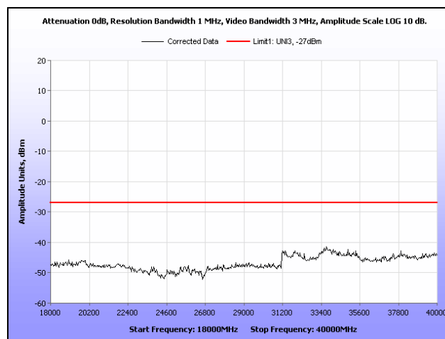
Plot 321. Radiated Spurious Emissions, 802.11n 20 MHz, High Channel, 18 GHz – 40 GHz, 10 dBi Omni Antenna
