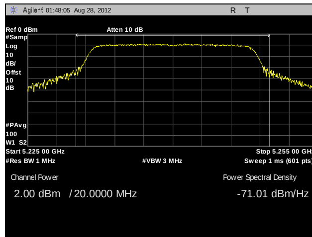
Plot 88. RF Power Output, 802.11a, High Channel, Port A, Panel Antenna
