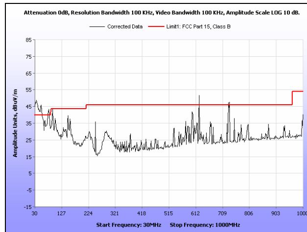
Plot 586. Restricted Band, 802.11n 40 MHz, Low Channel, Panel Antenna, 30 MHz – 1 GHz
