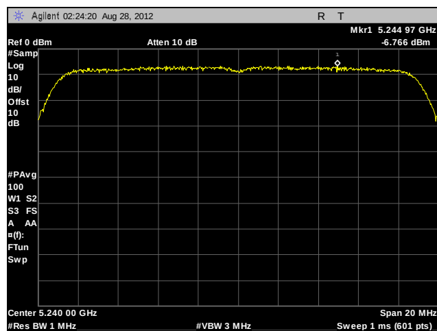
Plot 234. Peak Power Spectral Density, 802.11n 20 MHz, High Channel, Port C, Lower Gain Omni Antenna
