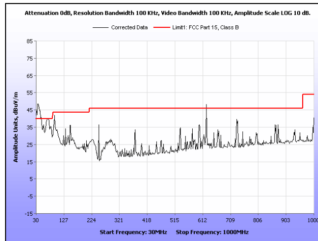
Plot 466. Restricted Band, 802.11a, Low Channel, Omni Antenna, 30 MHz – 1 GHz
