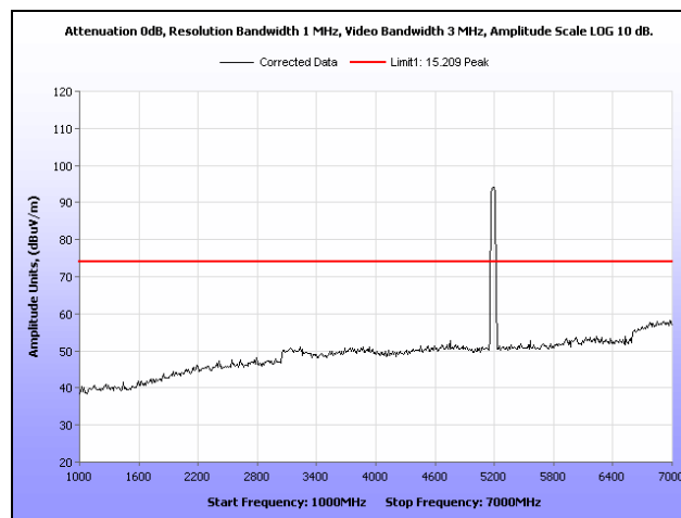
Plot 543. Restricted Band, 802.11n 40 MHz, Low Channel, Low Gain Omni Antenna, 1 GHz – 7 GHz, Peak
