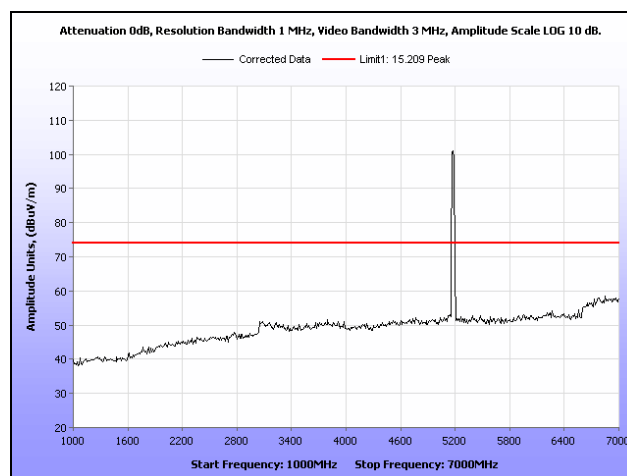
Plot 573. Restricted Band, 802.11n 20 MHz, Low Channel, Panel Antenna, 1 GHz – 7 GHz, Peak
