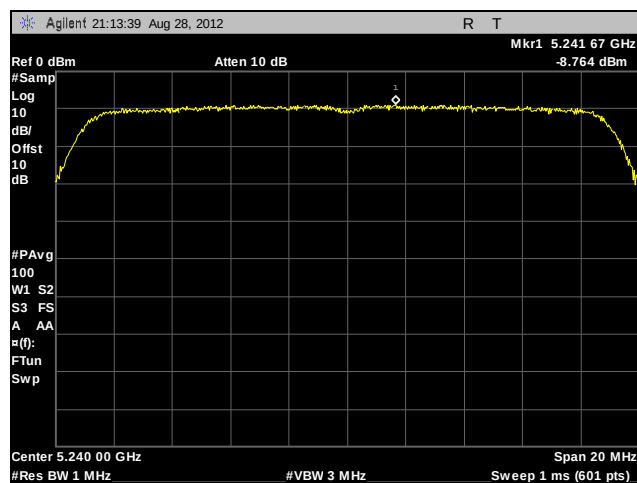
Plot 261. Peak Power Spectral Density, 802.11n 20 MHz, High Channel, Port C, Patch Antenna
