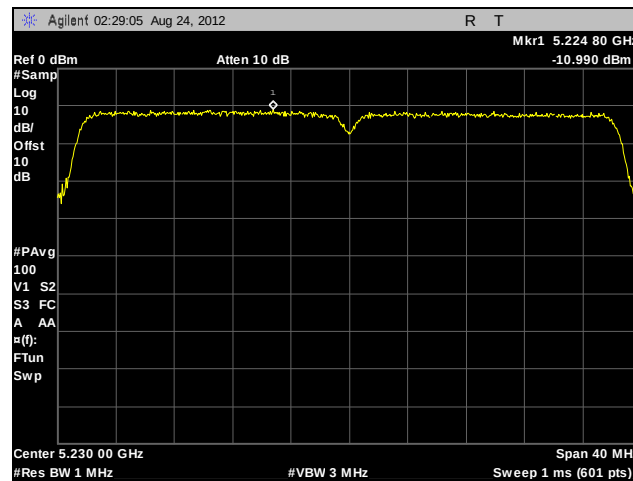
Plot 268. Peak Power Spectral Density, 802.11n 40 MHz, High Channel, Port A, Patch Antenna
