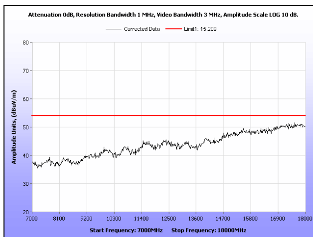
Plot 639. Restricted Band, 802.11n 40 MHz, Mid Channel, Patch Antenna, 7 GHz – 18 GHz
