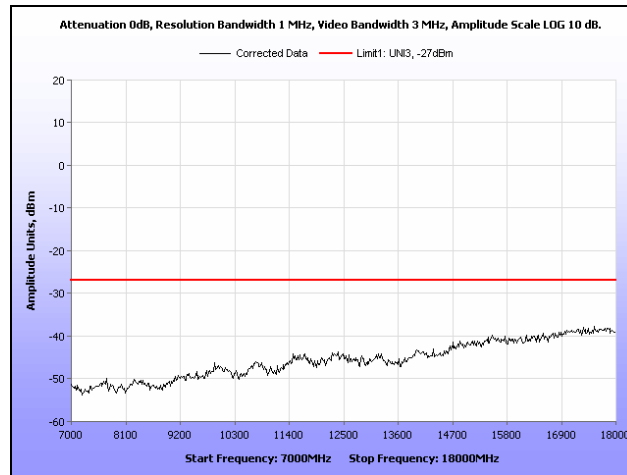
Plot 436. Radiated Spurious Emissions, 802.11n 40 MHz, Mid Channel, 7 GHz – 18 GHz, 10.1 dBi Patch Antenna
