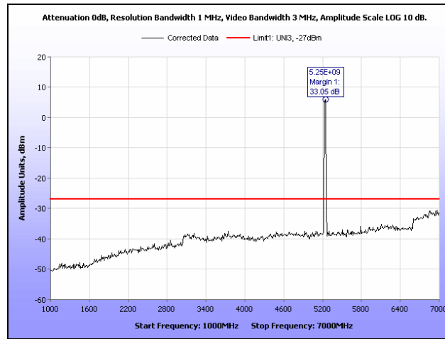
Plot 379. Radiated Spurious Emissions, 802.11a, High Channel, 1 GHz – 7 GHz, 8.25 dBi Omni Antenna
