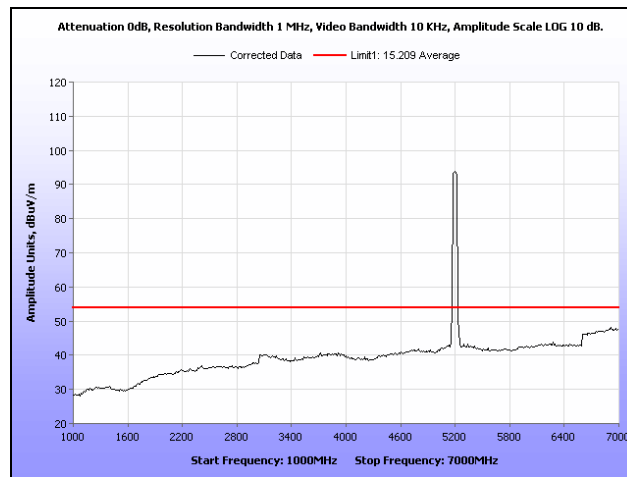
Plot 547. Restricted Band, 802.11n 40 MHz, Mid Channel, Low Gain Omni Antenna, 1 GHz – 7 GHz, Average
