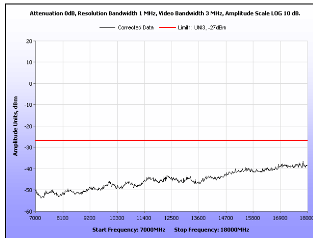
Plot 304. Radiated Spurious Emissions, 802.11a, Mid Channel, 7 GHz – 18 GHz, 10 dBi Omni Antenna
