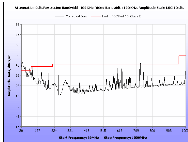
Plot 571. Restricted Band, 802.11n 20 MHz, Low Channel, Panel Antenna, 30 MHz – 1 GHz
