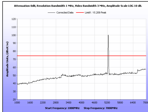
Plot 583. Restricted Band, 802.11n 20 MHz, High Channel, Panel Antenna, 1 GHz – 7 GHz, Peak
