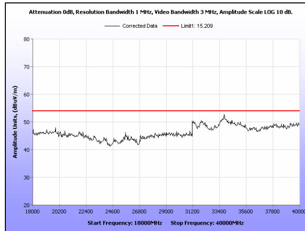
Plot 565. Restricted Band, 802.11a, Mid Channel, Panel Antenna, 18 GHz – 40 GHz
