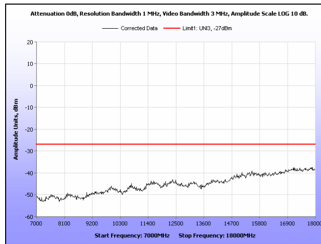
Plot 424. Radiated Spurious Emissions, 802.11n 20 MHz, Mid Channel, 7 GHz – 18 GHz, 10.1 dBi Patch Antenna
