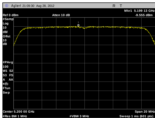
Plot 258. Peak Power Spectral Density, 802.11n 20 MHz, Mid Channel, Port C, Patch Antenna
