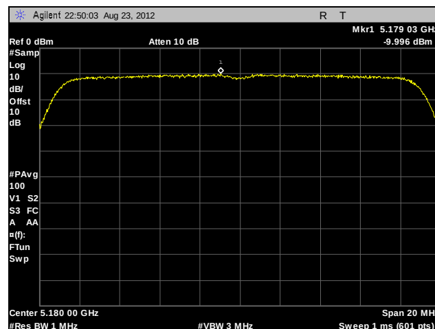
Plot 255. Peak Power Spectral Density, 802.11n 20 MHz, Low Channel, Port C, Patch Antenna
