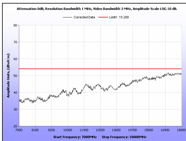
Plot 579. Restricted Band, 802.11n 20 MHz, Mid Channel, Panel Antenna, 7 GHz – 18 GHz
