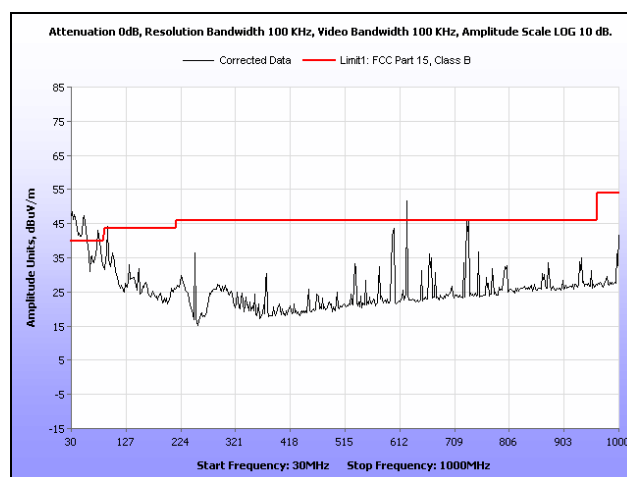
Plot 438. Radiated Spurious Emissions, 802.11n 40 MHz, High Channel, 30 MHz – 1 GHz, 10.1 dBi Patch Antenna
