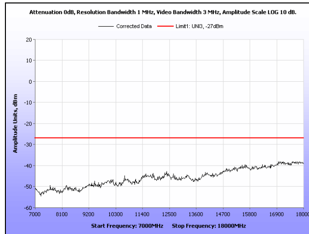
Plot 388. Radiated Spurious Emissions, 802.11n 20 MHz, Mid Channel, 7 GHz – 18 GHz, 8.25 dBi Omni Antenna
