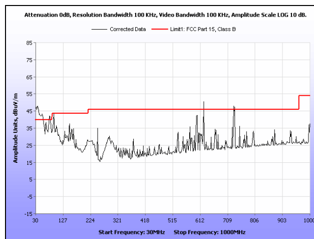
Plot 561. Restricted Band, 802.11a, Mid Channel, Panel Antenna, 30 MHz – 1 GHz
