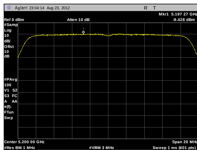
Plot 177. Peak Power Spectral Density, 802.11n 20 MHz, Mid Channel, Port C, Omni Antenna
