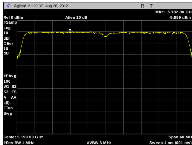
Plot 262. Peak Power Spectral Density, 802.11n 40 MHz, Low Channel, Port A, Patch Antenna
