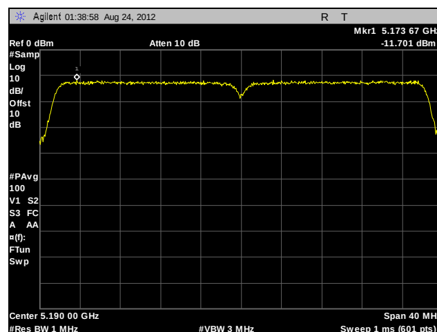
Plot 183. Peak Power Spectral Density, 802.11n 40 MHz, Low Channel, Port C, Omni Antenna
