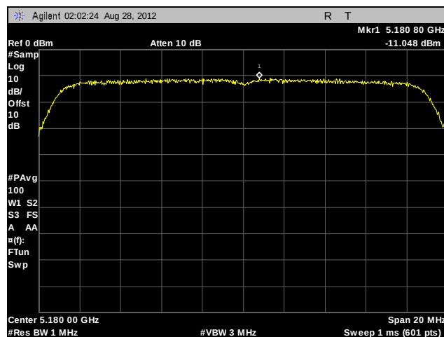
Plot 227. Peak Power Spectral Density, 802.11n 20 MHz, Low Channel, Port B, Lower Gain Omni Antenna
