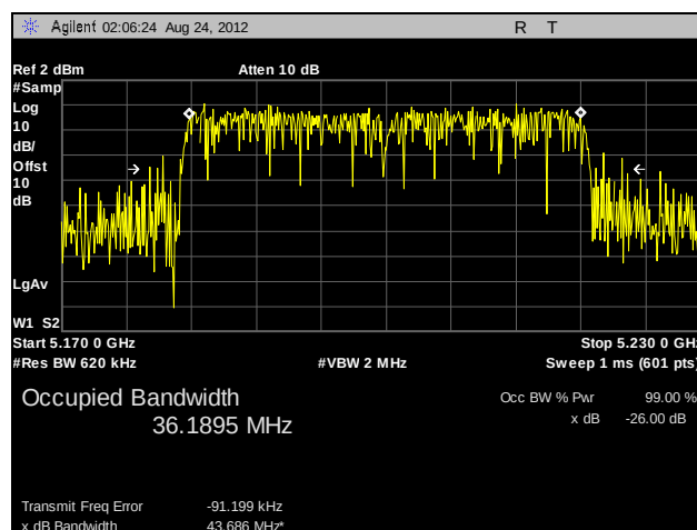
Plot 51. 99% Occupied Bandwidth, 802.11n 40 MHz, Mid Channel, Port C
