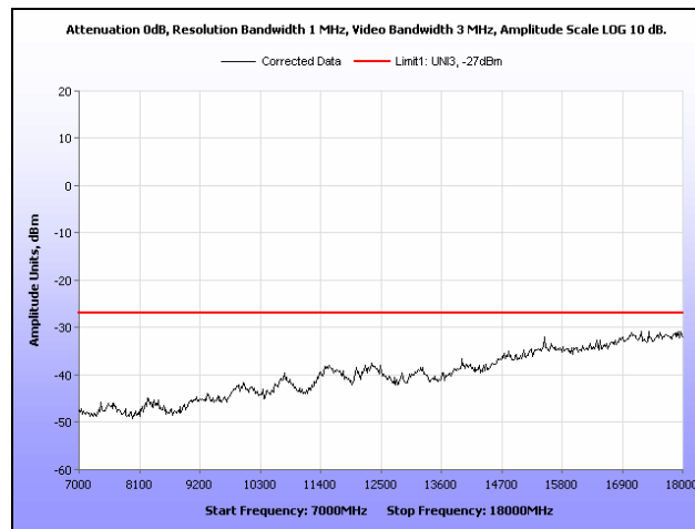
Plot 340. Radiated Spurious Emissions, 802.11a, Mid Channel, 7 GHz – 18 GHz, 10.7 dBi Panel Antenna
