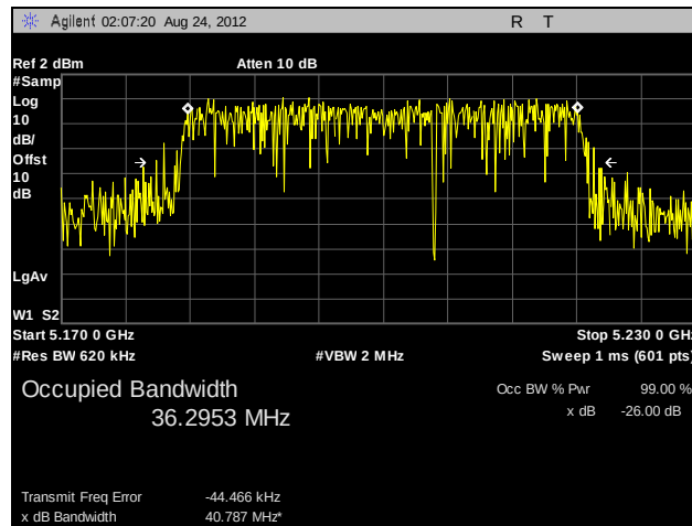
Plot 49. 99% Occupied Bandwidth, 802.11n 40 MHz, Mid Channel, Port A
