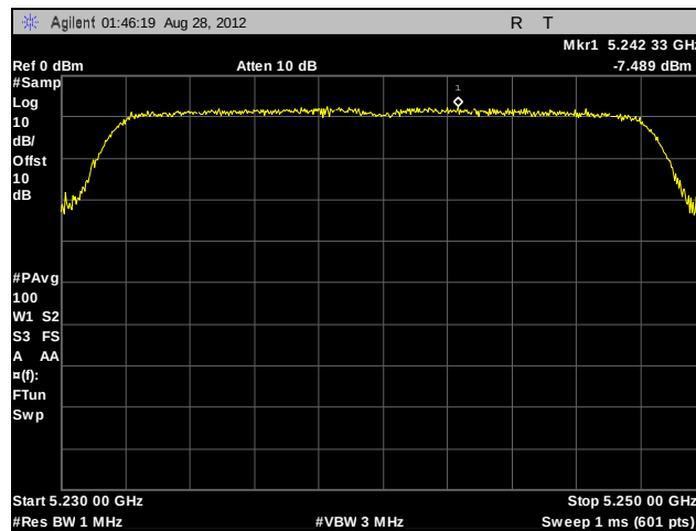
Plot 223. Peak Power Spectral Density, 802.11a, High Channel, Port A, Lower Gain Omni Antenna
