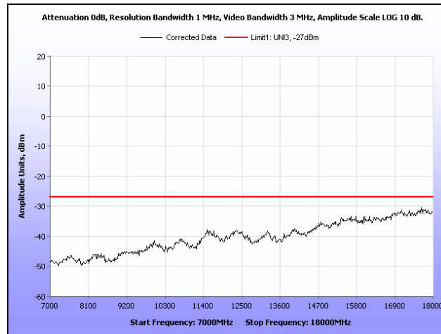
Plot 364. Radiated Spurious Emissions, 802.11n 40 MHz, Mid Channel, 7 GHz – 18 GHz, 10.7 dBi Panel Antenna
