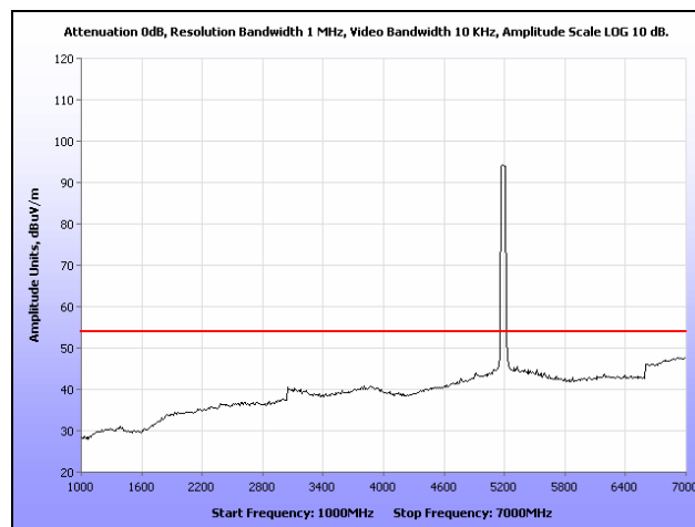
Plot 587. Restricted Band, 802.11n 40 MHz, Low Channel, Panel Antenna, 1 GHz – 7 GHz, Average
