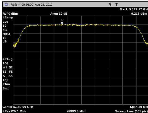
Plot 190. Peak Power Spectral Density, 802.11a, Low Channel, Port A, Panel Antenna
