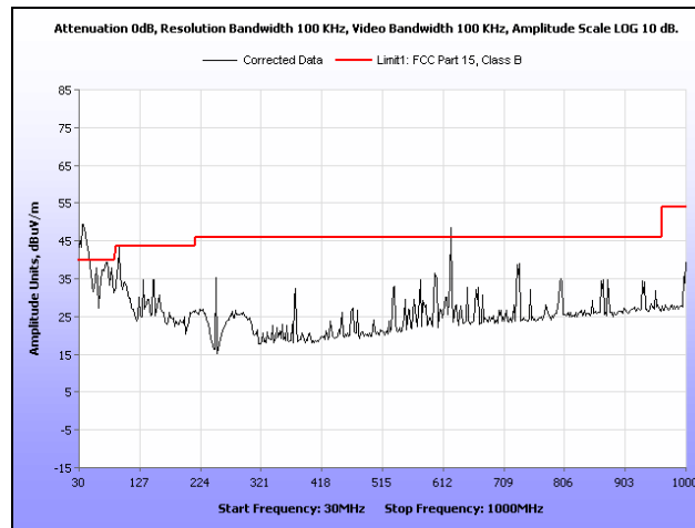
Plot 481. Restricted Band, 802.11n 20 MHz, Low Channel, Omni Antenna, 30 MHz – 1 GHz
