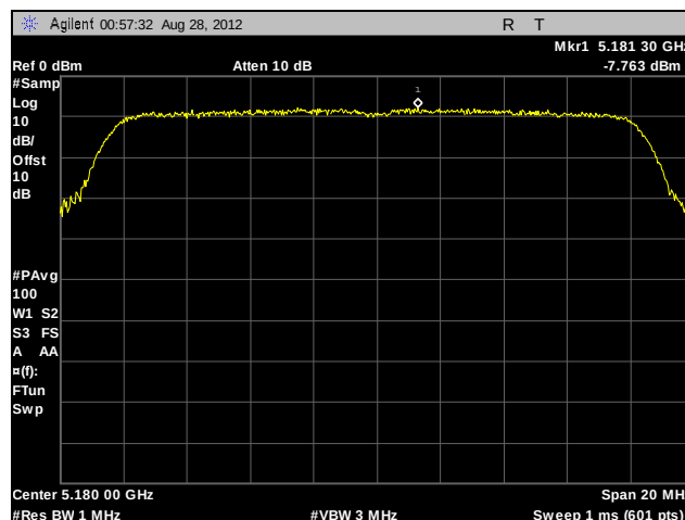
Plot 192. Peak Power Spectral Density, 802.11a, Low Channel, Port C, Panel Antenna
