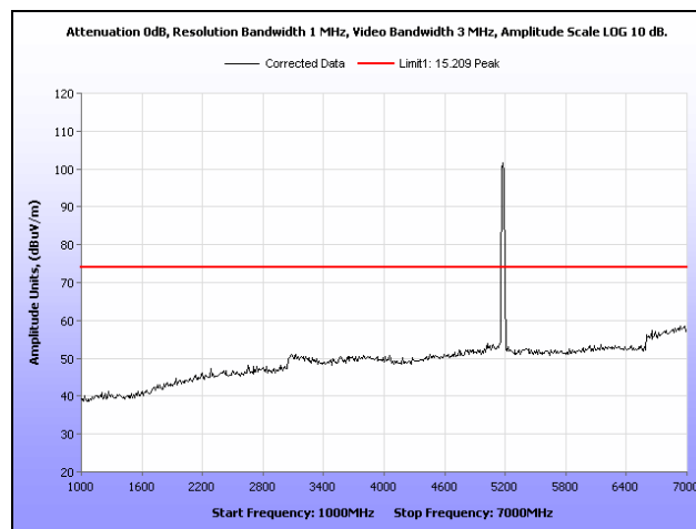
Plot 483. Restricted Band, 802.11n 20 MHz, Low Channel, Omni Antenna, 1 GHz – 7 GHz, Peak
