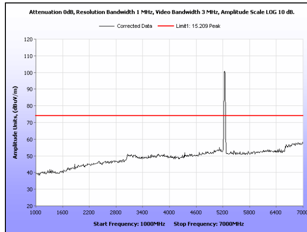
Plot 478. Restricted Band, 802.11a, High Channel, Omni Antenna, 1 GHz – 7 GHz, Peak
