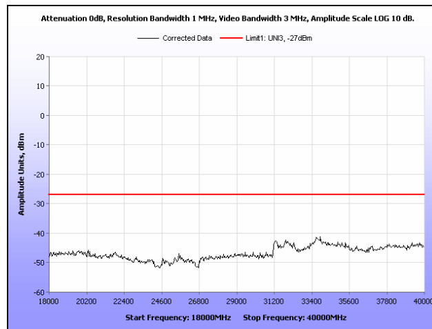
Plot 313. Radiated Spurious Emissions, 802.11n 20 MHz, Low Channel, 18 GHz – 40 GHz, 10 dBi Omni Antenna
