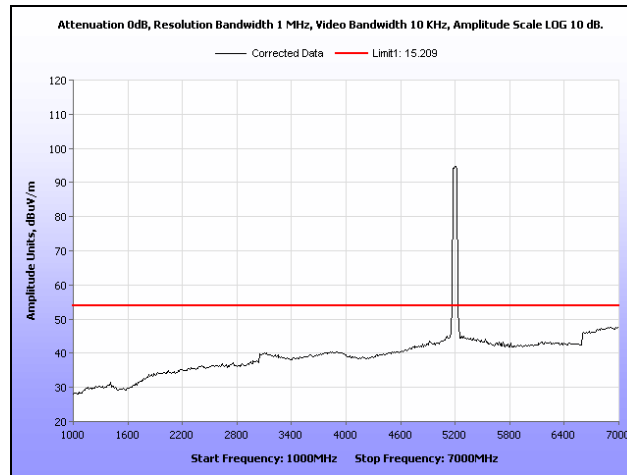
Plot 592. Restricted Band, 802.11n 40 MHz, Mid Channel, Panel Antenna, 1 GHz – 7 GHz, Average
