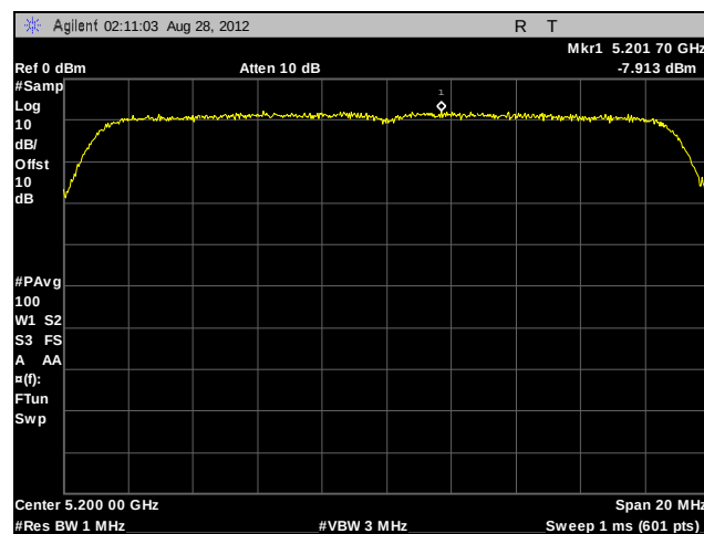
Plot 204. Peak Power Spectral Density, 802.11n 20 MHz, Mid Channel, Port C, Panel Antenna
