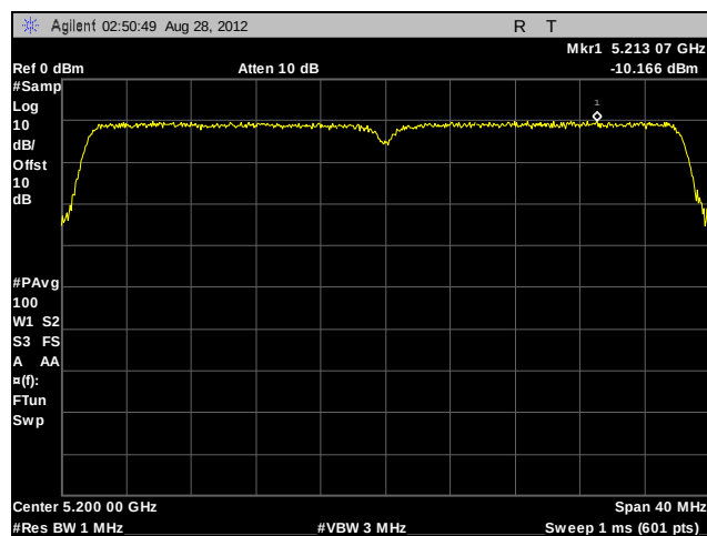
Plot 213. Peak Power Spectral Density, 802.11n 40 MHz, Mid Channel, Port C, Panel Antenna
