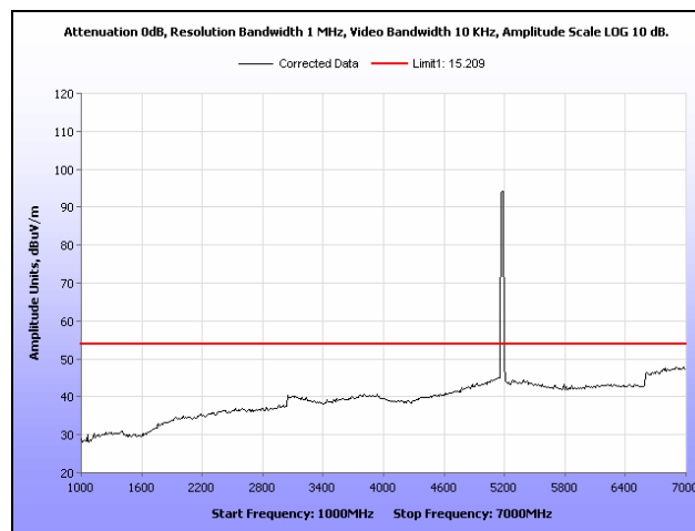
Plot 467. Restricted Band, 802.11a, Low Channel, Omni Antenna, 1 GHz – 7 GHz, Average
