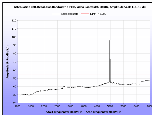
Plot 572. Restricted Band, 802.11n 20 MHz, Low Channel, Panel Antenna, 1 GHz – 7 GHz, Average
