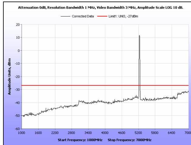
Plot 307. Radiated Spurious Emissions, 802.11a, High Channel, 1 GHz – 7 GHz, 10 dBi Omni Antenna
