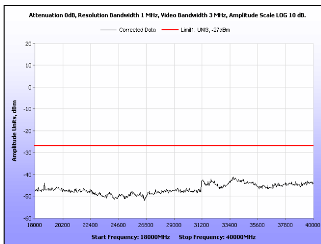
Plot 417. Radiated Spurious Emissions, 802.11a, High Channel, 18 GHz – 40 GHz, 10.1 dBi Patch Antenna
