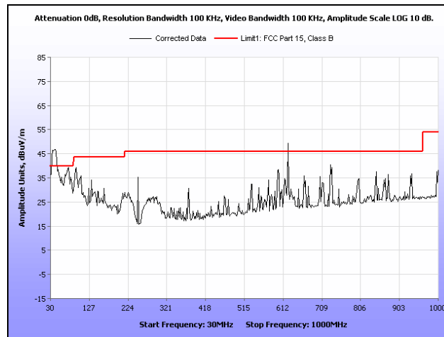
Plot 526. Restricted Band, 802.11n 20 MHz, Low Channel, Low Gain Omni Antenna, 30 MHz – 1 GHz
