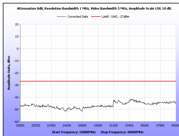
Plot 429. Radiated Spurious Emissions, 802.11n 20 MHz, High Channel, 18 GHz – 40 GHz, 10.1 dBi Patch Antenna
