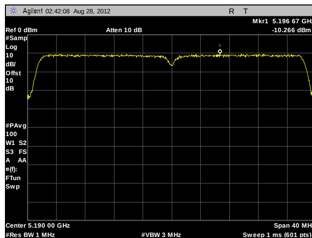
Plot 210. Peak Power Spectral Density, 802.11n 40 MHz, Low Channel, Port C, Panel Antenna
