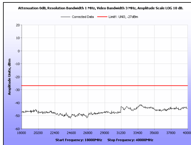
Plot 433. Radiated Spurious Emissions, 802.11n 40 MHz, Low Channel, 18 GHz – 40 GHz, 10.1 dBi Patch Antenna
