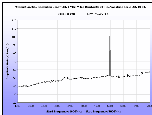
Plot 603. Restricted Band, 802.11a, Low Channel, Patch Antenna, 1 GHz – 7 GHz, Peak
