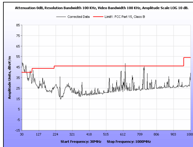
Plot 601. Restricted Band, 802.11a, Low Channel, Patch Antenna, 30 MHz – 1 GHz
