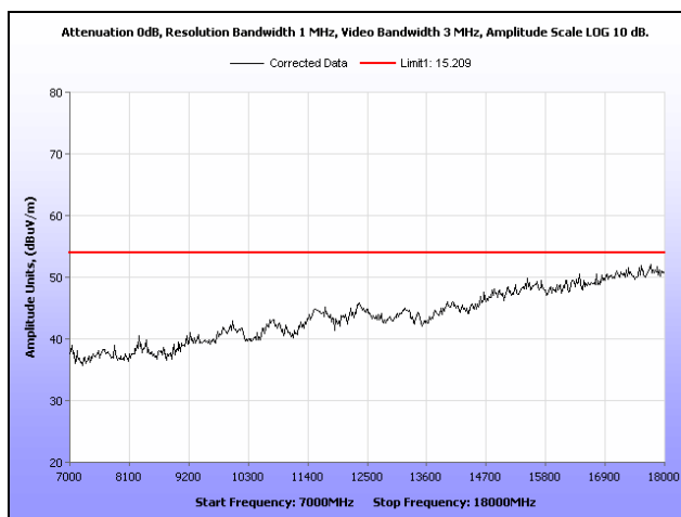
Plot 609. Restricted Band, 802.11a, Mid Channel, Patch Antenna, 7 GHz – 18 GHz
