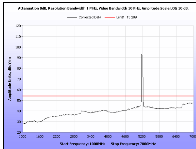
Plot 502. Restricted Band, 802.11n 40 MHz, Mid Channel, Omni Antenna, 1 GHz – 7 GHz, Average
