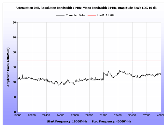
Plot 615. Restricted Band, 802.11a, High Channel, Patch Antenna, 18 GHz – 40 GHz
