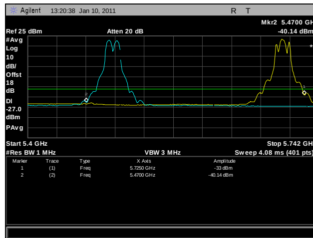
Plot 297. Frequency Stability, 0°C for 5470 MHz - 5725 MHz at 102 VAC
