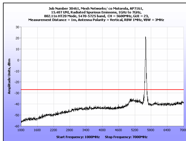
Plot 198. Radiated Spurious Emissions, 1 GHz – 7 GHz, 802.11n HT20, 5600 MHz
