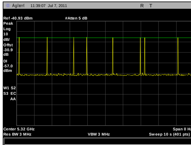
Plot 337. Bin 5 Radar Calibration for 5 dBi
