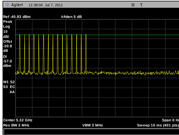
Plot 336. Bin 4 Radar Calibration for 5 dBi
