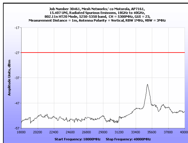
Plot 188. Radiated Spurious Emissions, 18 GHz – 40 GHz, 802.11n HT20, 5300 MHz
