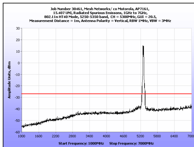
Plot 210. Radiated Spurious Emissions, 1 GHz – 7 GHz, 802.11n HT40, 5300 MHz
