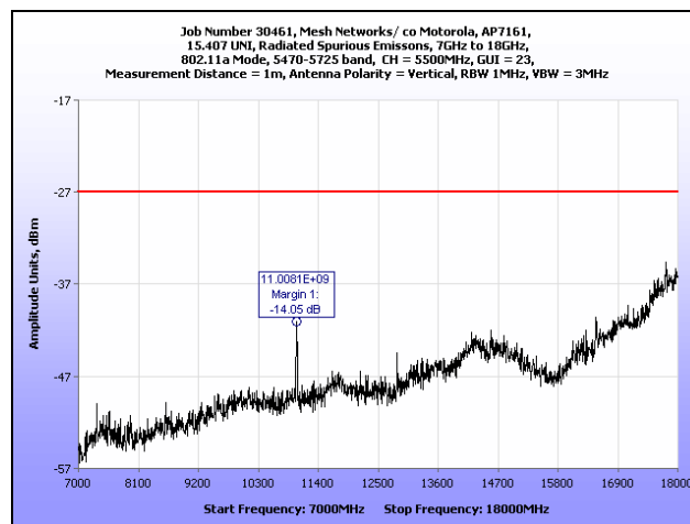
Plot 171. Radiated Spurious Emissions, 7 GHz – 18 GHz, 802.11a, 5500 MHz
