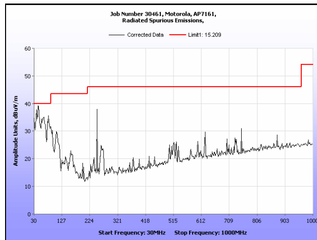
Plot 185. Radiated Spurious Emissions, 30 MHz – 1 GHz, 802.11n HT20, 5300 MHz
