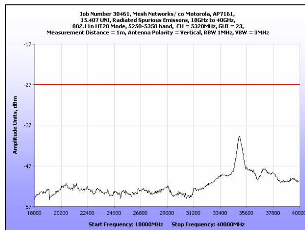
Plot 192. Radiated Spurious Emissions, 18 GHz – 40 GHz, 802.11n HT20, 5320 MHz
