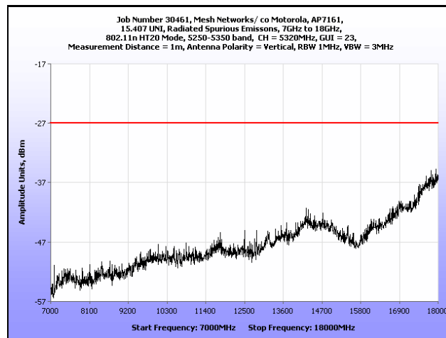
Plot 191. Radiated Spurious Emissions, 7 GHz – 18 GHz, 802.11n HT20, 5320 MHz
