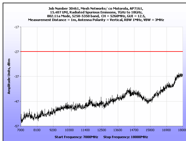
Plot 159. Radiated Spurious Emissions, 7 GHz – 18 GHz, 802.11a, 5260 MHz
