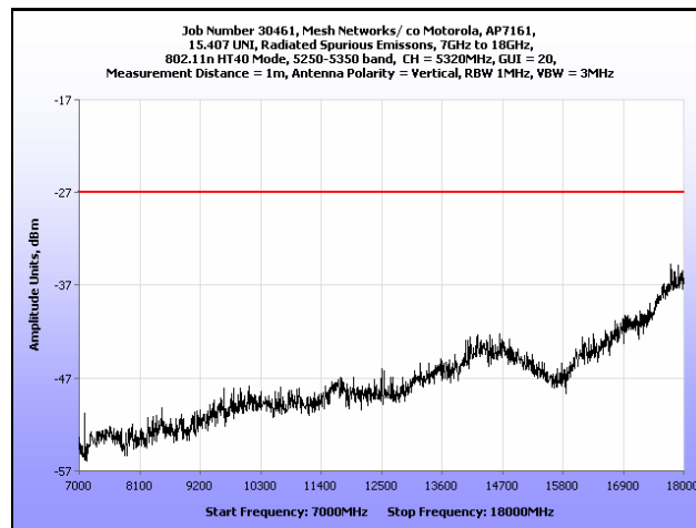
Plot 215. Radiated Spurious Emissions, 7 GHz – 18 GHz, 802.11n HT40, 5320 MHz
