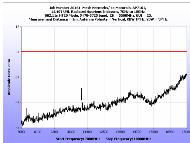
Plot 195. Radiated Spurious Emissions, 7 GHz – 18 GHz, 802.11n HT20, 5500 MHz
