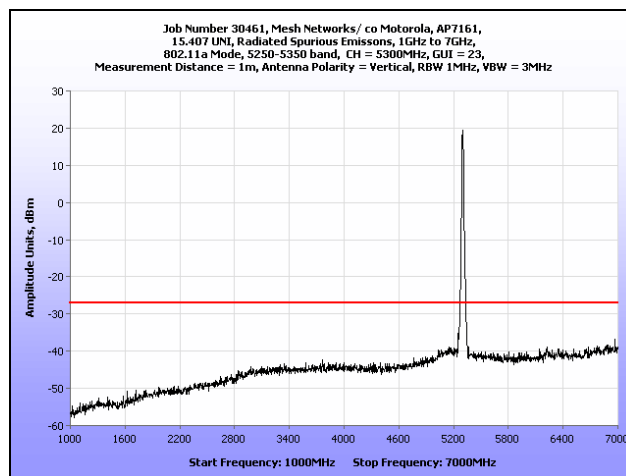
Plot 162. Radiated Spurious Emissions, 1 GHz – 7 GHz, 802.11a, 5300 MHz
