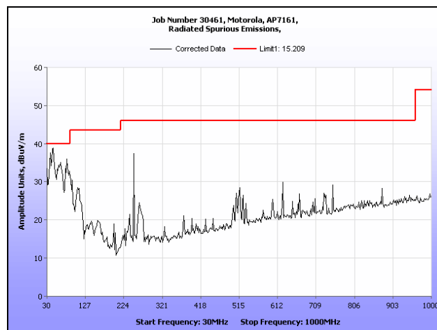
Plot 213. Radiated Spurious Emissions, 30 MHz – 1 GHz, 802.11n HT40, 5320 MHz
