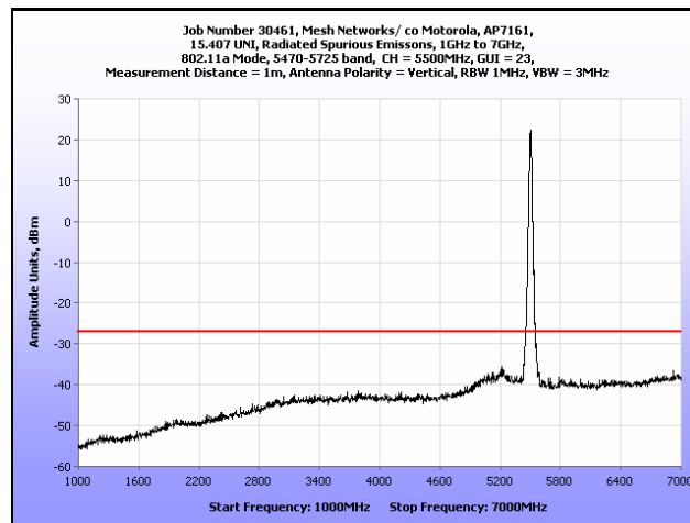
Plot 170. Radiated Spurious Emissions, 1 GHz – 7 GHz, 802.11a, 5500 MHz
