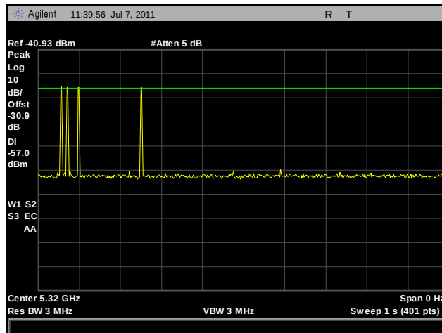
Plot 338. Bin 6 Radar Calibration for 5 dBi
