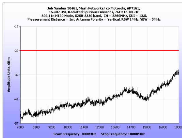
Plot 183. Radiated Spurious Emissions, 7 GHz – 18 GHz, 802.11n HT20, 5260 MHz
