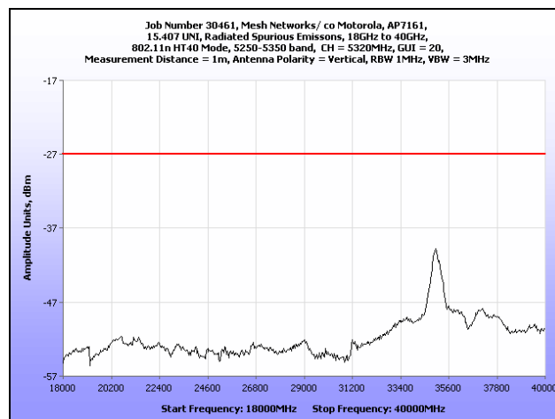
Plot 216. Radiated Spurious Emissions, 18 GHz – 40 GHz, 802.11n HT40, 5320 MHz
