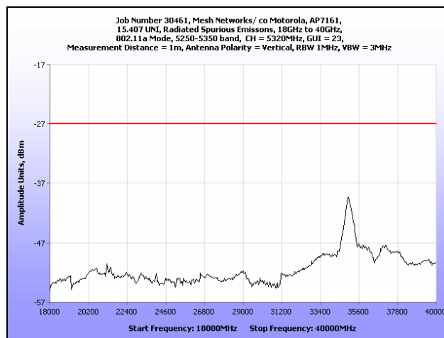
Plot 168. Radiated Spurious Emissions, 18 GHz – 40 GHz, 802.11a, 5320 MHz
