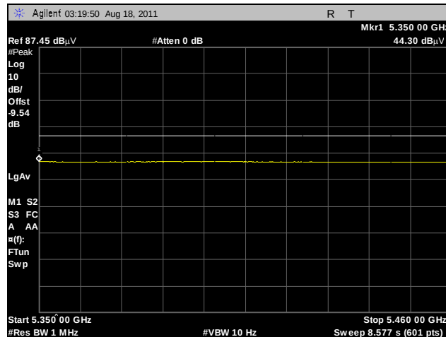
Plot 236. Radiated Restricted Band, 802.11n HT20, 5320 MHz, Average
