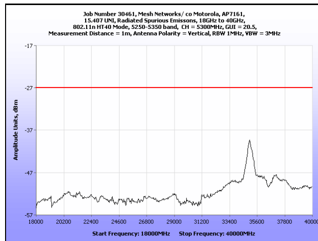
Plot 212. Radiated Spurious Emissions, 18 GHz – 40 GHz, 802.11n HT40, 5300 MHz
