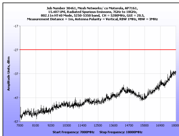
Plot 207. Radiated Spurious Emissions, 7 GHz – 18 GHz, 802.11n HT40, 5280 MHz
