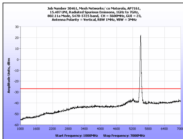
Plot 174. Radiated Spurious Emissions, 1 GHz – 7 GHz, 802.11a, 5600 MHz
