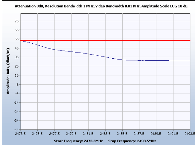
Restricted Band High Edge, Channel 11, 20 dBm, Average
