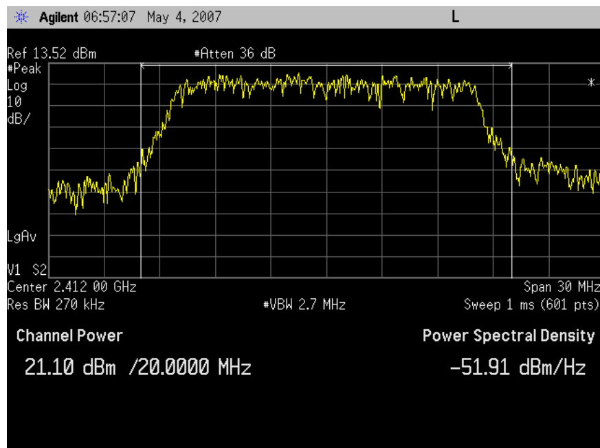
Peak Output Power, 802.11g, Channel 1
