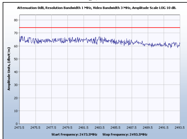
Restricted Band High Edge, Channel 6, 25 dBm, Peak
