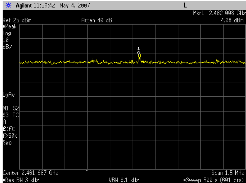
Peak Power Spectral Density, 802.11b, Channel 11
