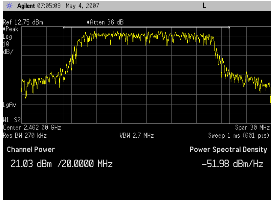
Peak Output Power, 802.11g, Channel 11
