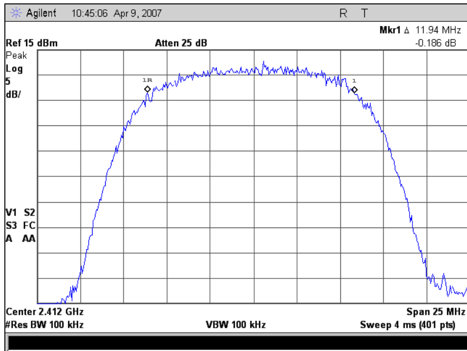
6 dB Occupied Bandwidth, 802.11b, Channel 1
