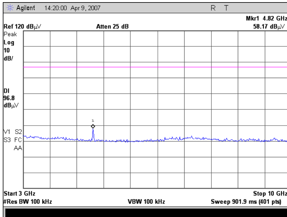
RF Conducted Spurious Emissions, 802.11b, Channel 1, 3-10 GHz
