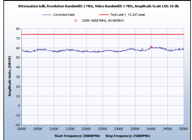
SpuriousRadiated Emissions, Channel 6, 20-25 GHz, Peak
