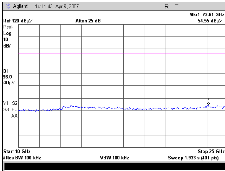
RF Conducted Spurious Emissions, 802.11g, Channel 1, 10-25 GHz
