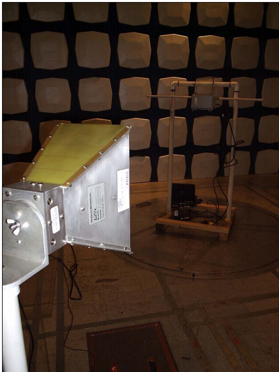
Photograph 3. Spurious Radiated Emissions, Test Setup
