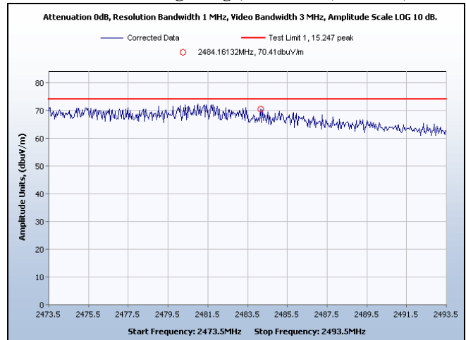
Restricted Band High Edge, Channel 7, 25 dBm, Peak
