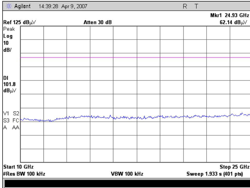
RF Conducted Spurious Emissions, 802.11b, Channel 11, 10-25 GHz
