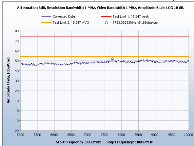
SpuriousRadiated Emissions, Channel 1, 5-10 GHz
