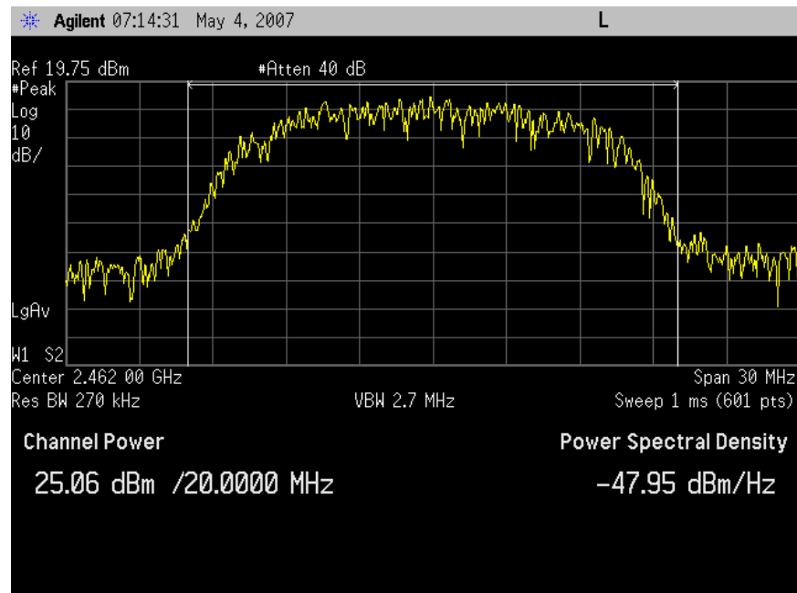
Peak Output Power, 802.11b, Channel 11
