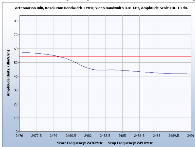
Restricted Band High Edge, Channel 11, 25 dBm, Average
