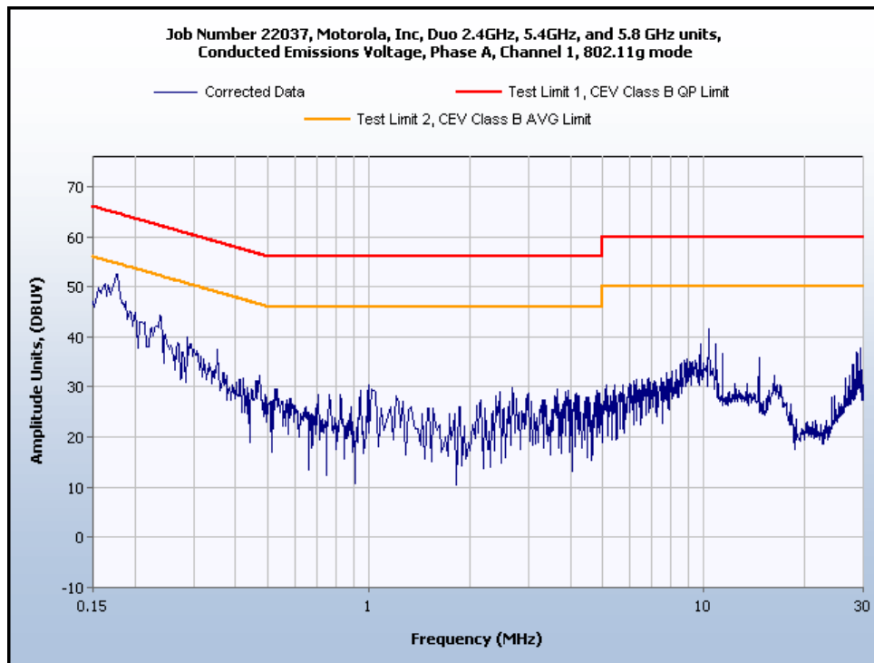
Channel 1 Phase Line Plot
