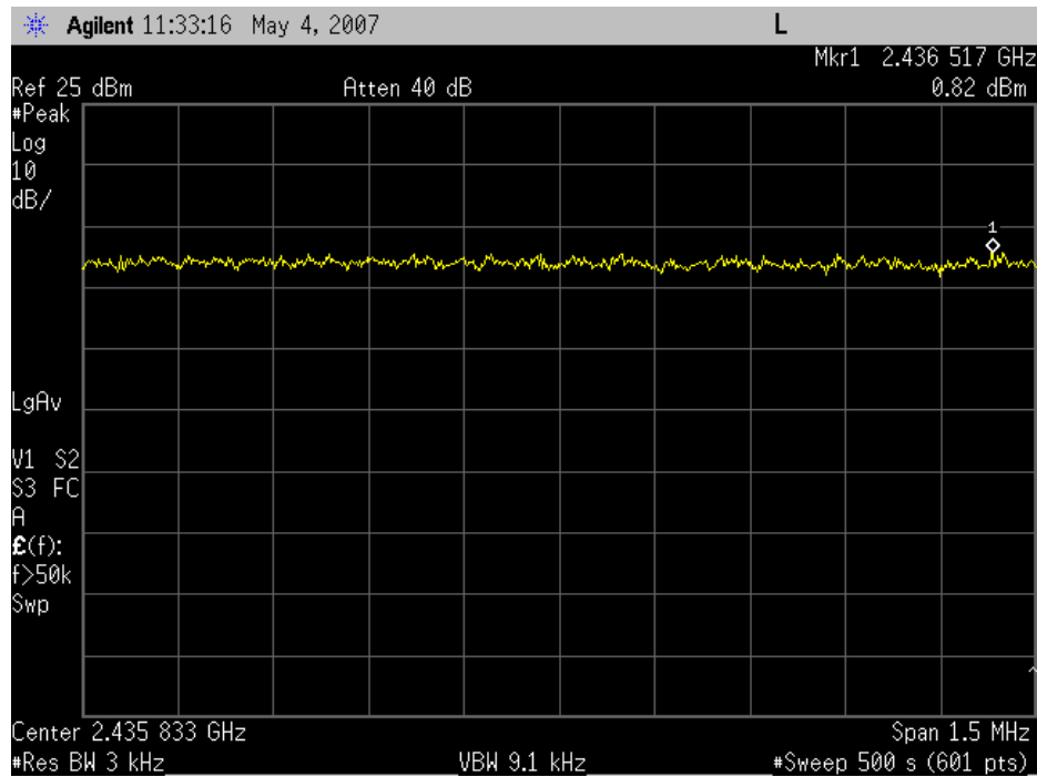
Peak Power Spectral Density, 802.11b, Channel 6
