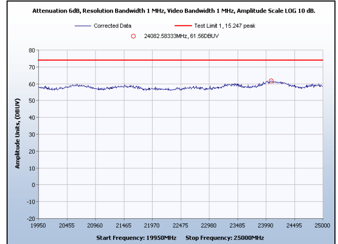
SpuriousRadiated Emissions, Channel 1, 20-25 GHz, Peak
