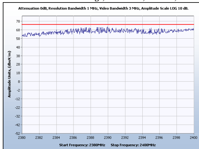
Restricted Band Low Edge, Channel 5, 25 dBm, Peak
