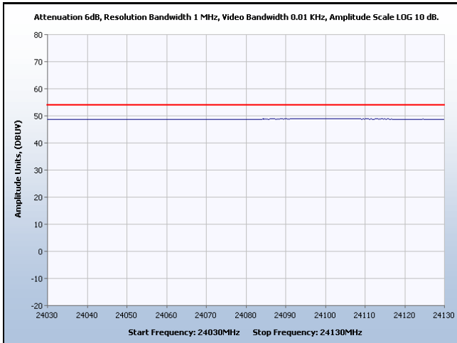
SpuriousRadiated Emissions, Channel 1, 20-25 GHz, Average
