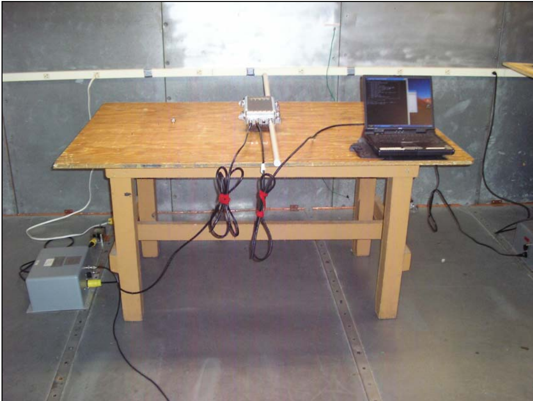
Photograph 1. Band Edge Test Setup
