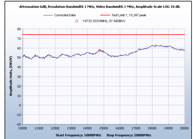
SpuriousRadiated Emissions, Channel 11, 10-20 GHz, Peak
