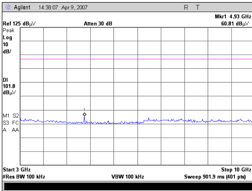
RF Conducted Spurious Emissions, 802.11b, Channel 11, 3-10 GHz
