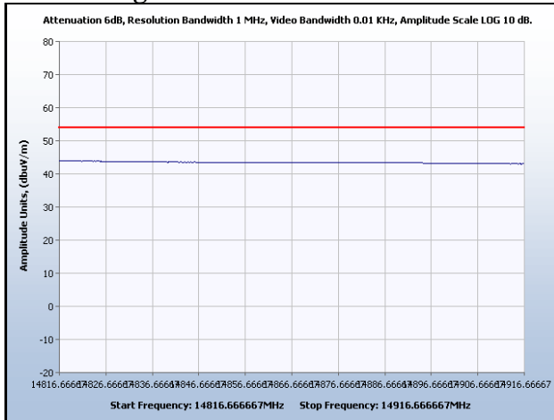
SpuriousRadiated Emissions, Channel 1, 10-20 GHz, Average
