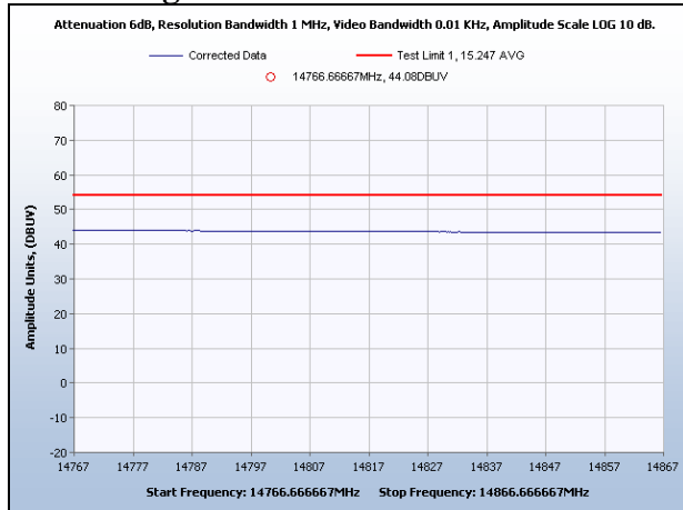
SpuriousRadiated Emissions, Channel 6, 10-20 GHz, Average
