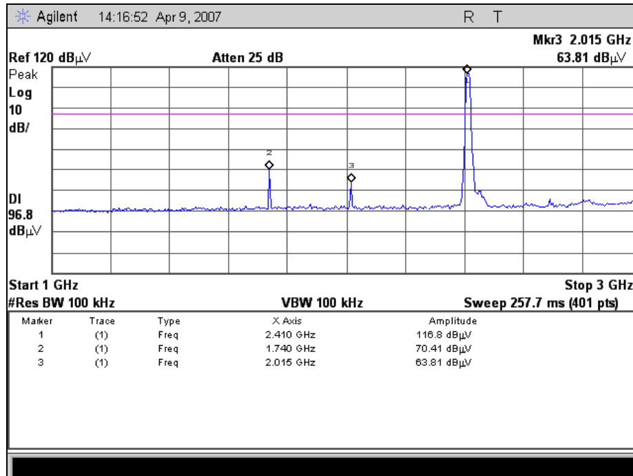
RF Conducted Spurious Emissions, 802.11b, Channel 1, 1-3 GHz
