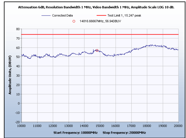
SpuriousRadiated Emissions, Channel 6, 10-20 GHz, Peak
