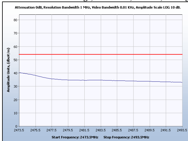
Restricted Band High Edge, Channel 6, 25 dBm, Average
