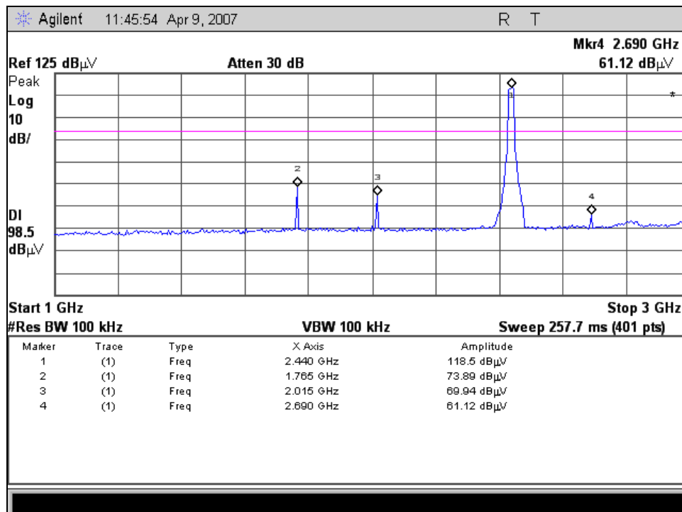
RF Conducted Spurious Emissions, 802.11g, Channel 6, 1-3 GHz
