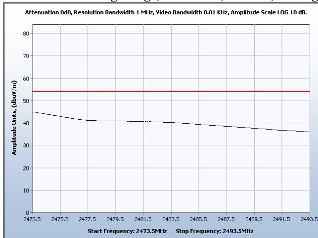
Restricted Band High Edge, Channel 7, 25 dBm, Average
