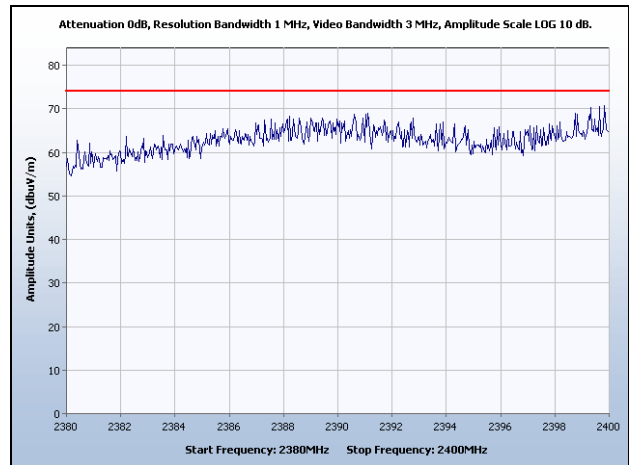
Restricted Band Low Edge, Channel 6, 25 dBm, Peak
