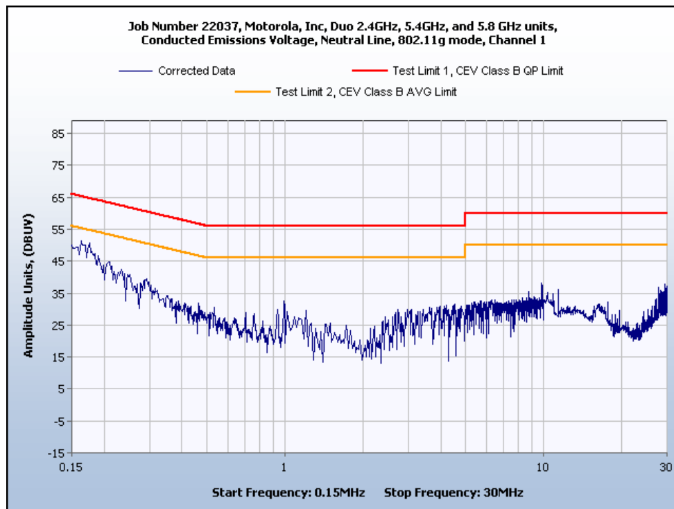
Channel 1 Neutral Line Plot
