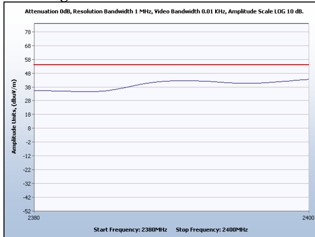
Restricted Band Low Edge, Channel 4, 23 dBm, Average
