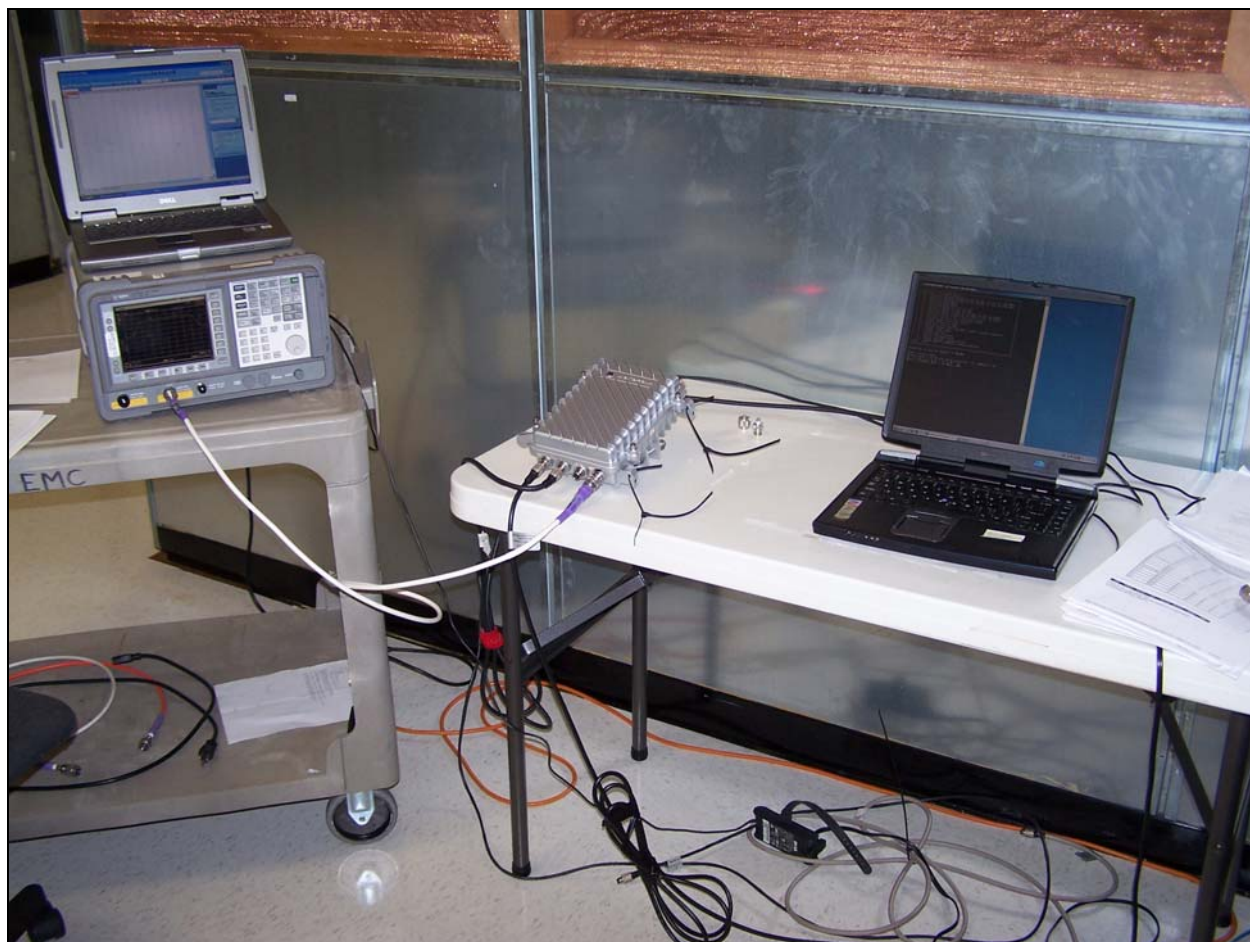
Photograph 6. Spurious Conducted Emissions, Test Setup
