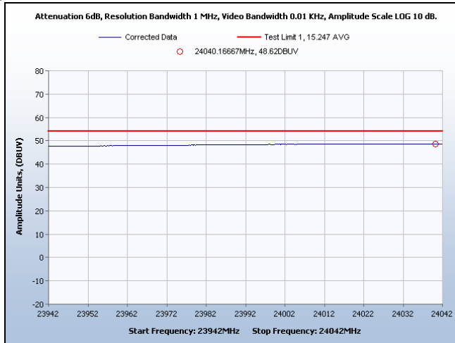
SpuriousRadiated Emissions, Channel 6, 20-25 GHz, Average
