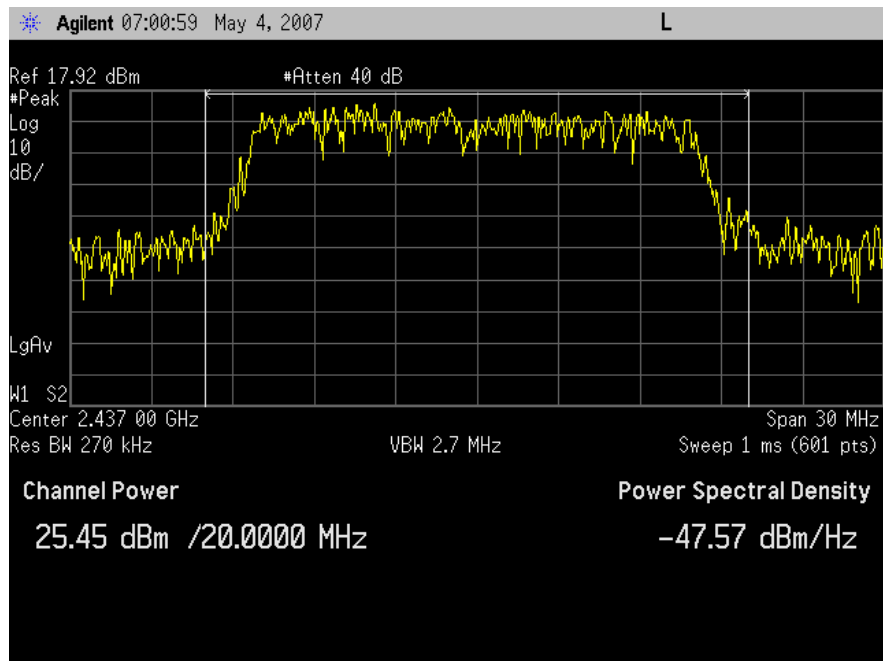
Peak Output Power, 802.11g, Channel 6
