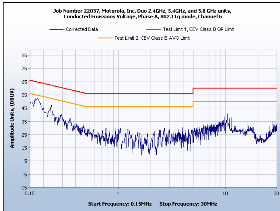
Channel 6 Phase Line Plot
