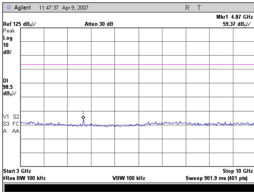
RF Conducted Spurious Emissions, 802.11g, Channel 6, 3-10 GHz
