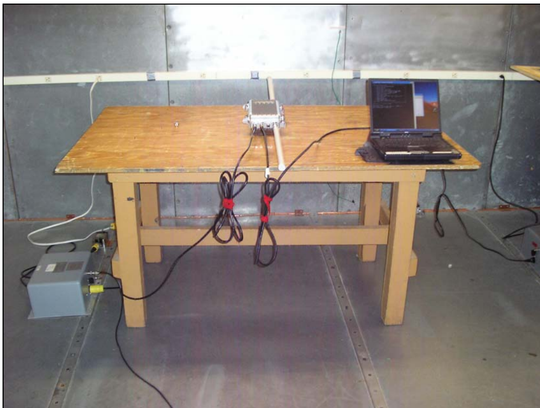
Photograph 2. Conducted Emission Test Setup
