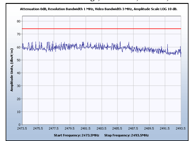
Restricted Band High Edge, Channel 5, 25 dBm, Peak
