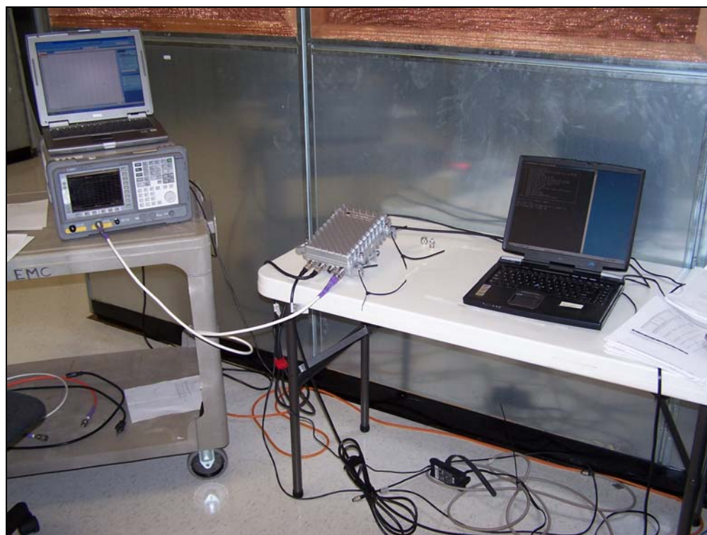
Photograph 4. 6 dB Bandwidth Test Setup
