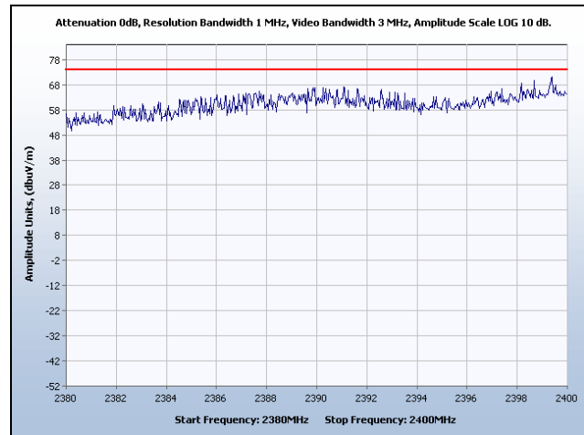
Restricted Band Low Edge, Channel 4, 23 dBm, Peak
