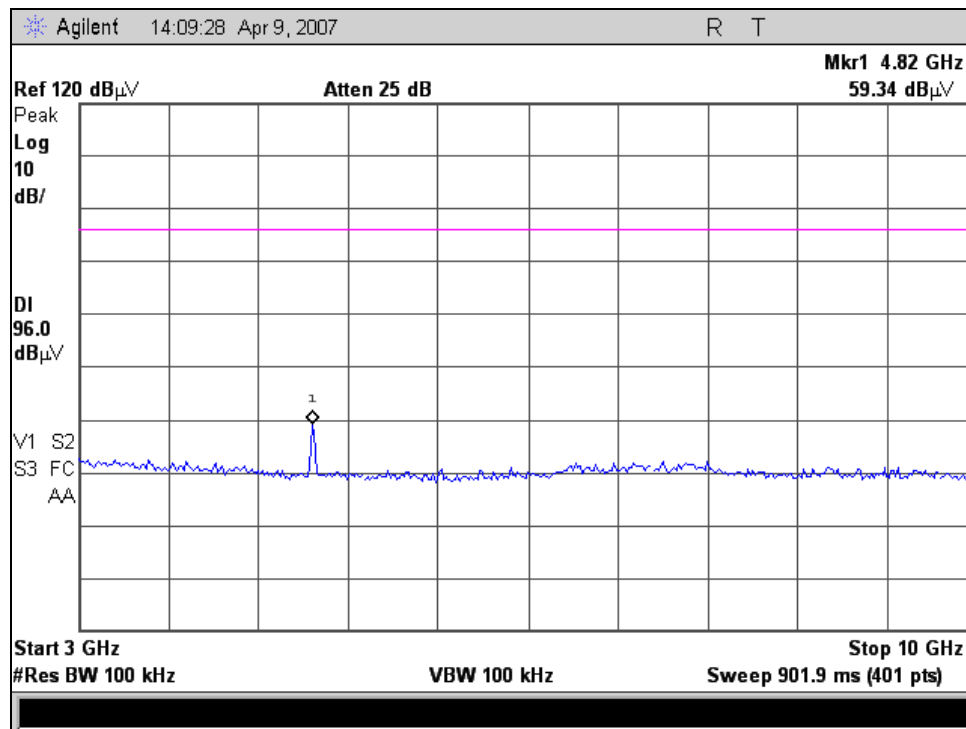
RF Conducted Spurious Emissions, 802.11g, Channel 1, 3-10 GHz
