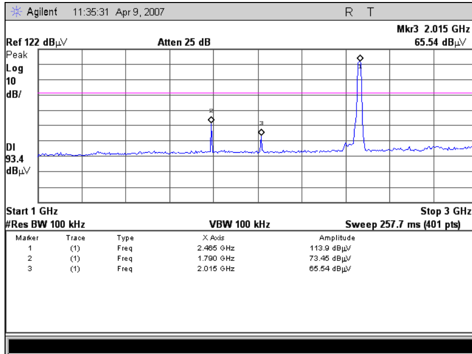
RF Conducted Spurious Emissions, 802.11g, Channel 11, 1-3 GHz
