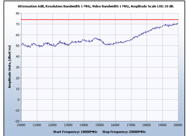
SpuriousRadiated Emissions, Channel 1, 10-20 GHz, Peak
