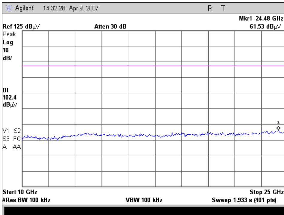
RF Conducted Spurious Emissions, 802.11b, Channel 6, 10-25 GHz
