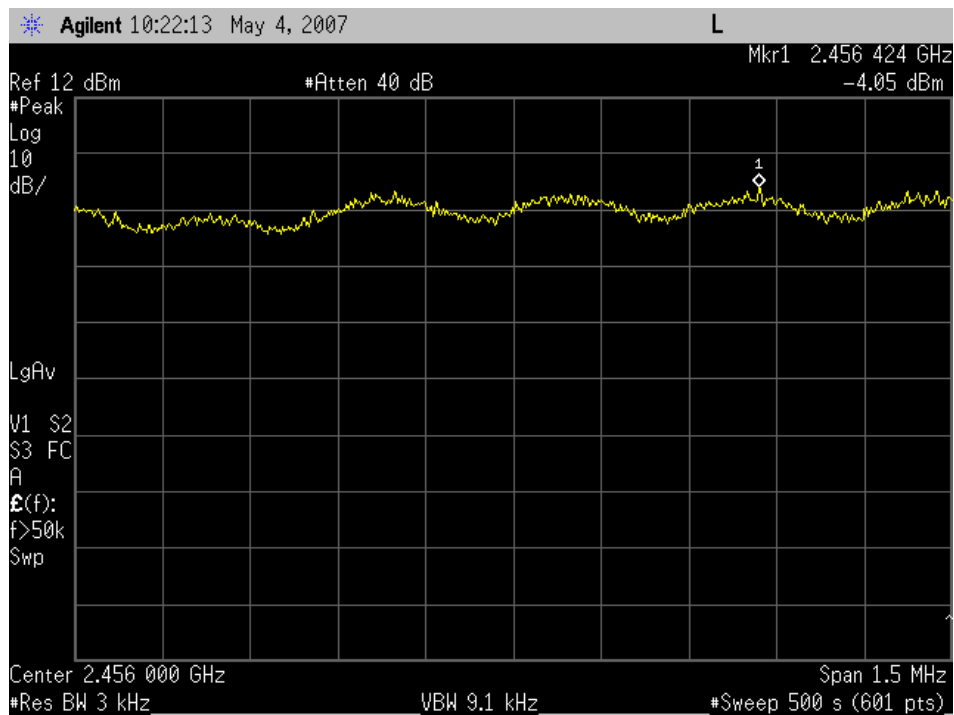
Peak Power Spectral Density, 802.11g, Channel 11
