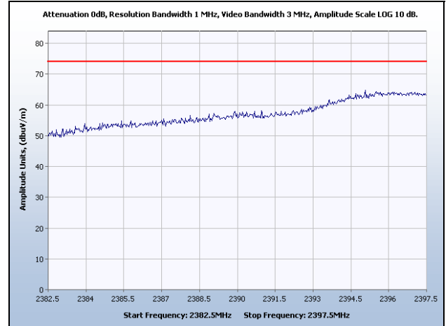
Restricted Band Low Edge, Channel 1, 27 dBm, Peak
