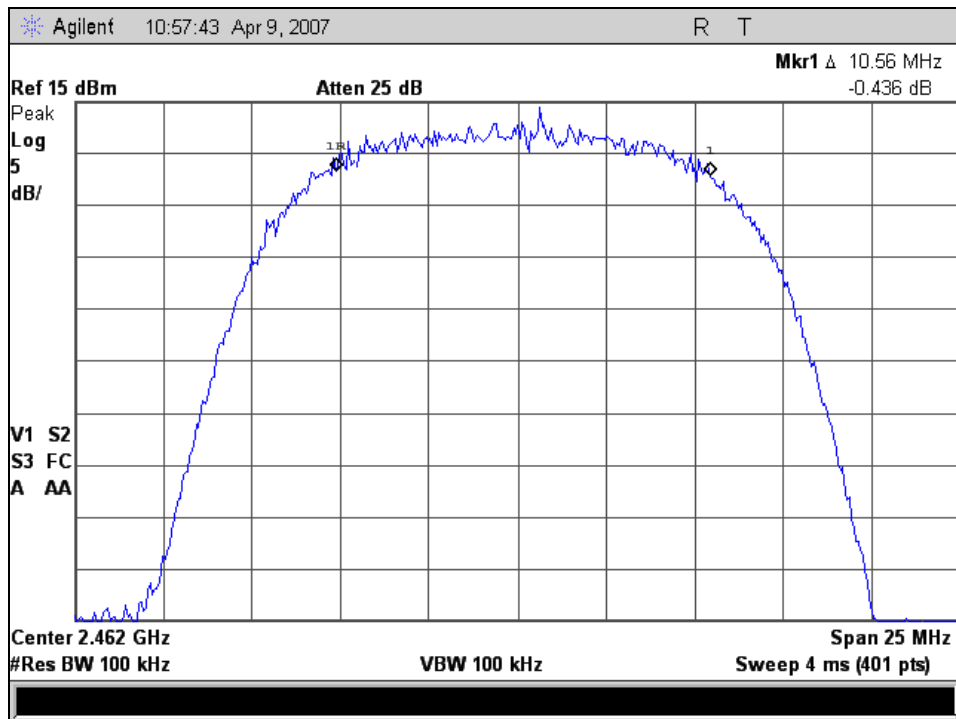
6 dB Occupied Bandwidth, 802.11b, Channel 11
