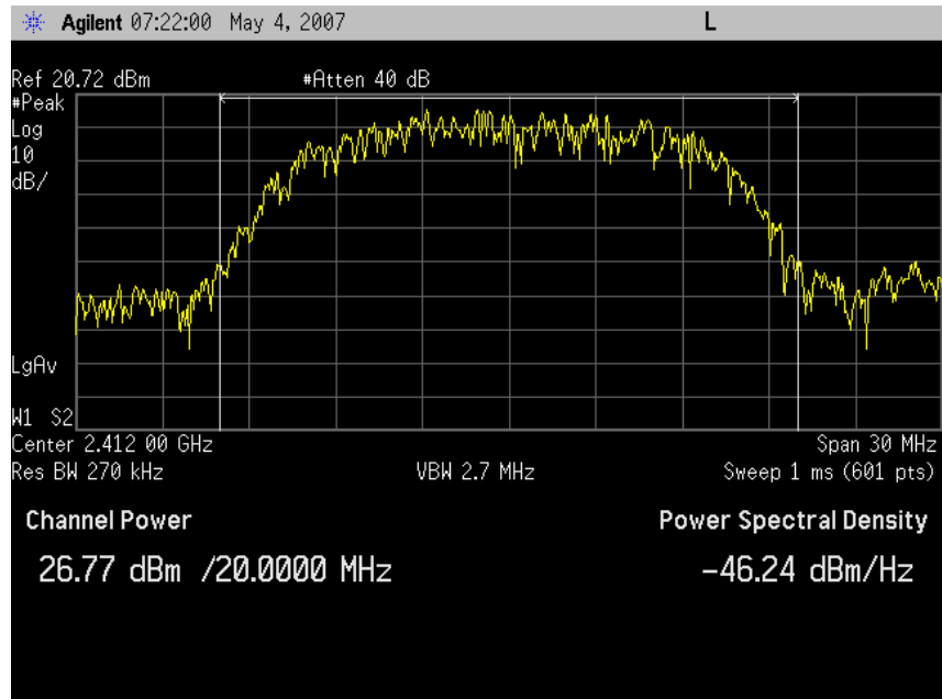
Peak Output Power, 802.11b, Channel 1
