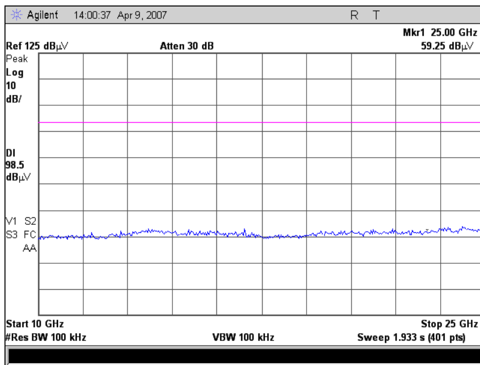
RF Conducted Spurious Emissions, 802.11g, Channel 6, 10-25 GHz
