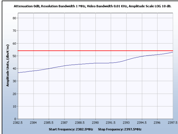
Restricted Band Low Edge, Channel 1, 27 dBm, Average
