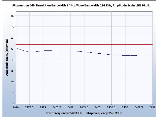
Restricted Band High Edge, Channel 10, 26 dBm, Average
