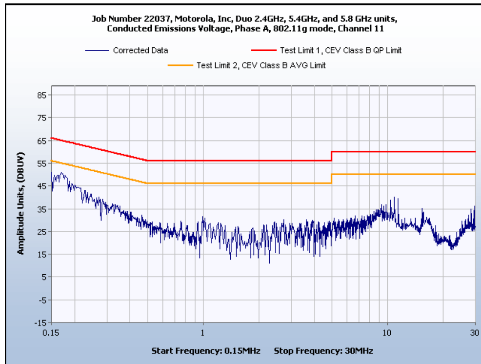
Channel 11 Phase Line Plot
