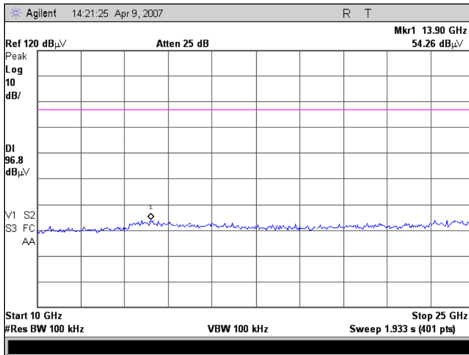
RF Conducted Spurious Emissions, 802.11b, Channel 1, 10-25 GHz
