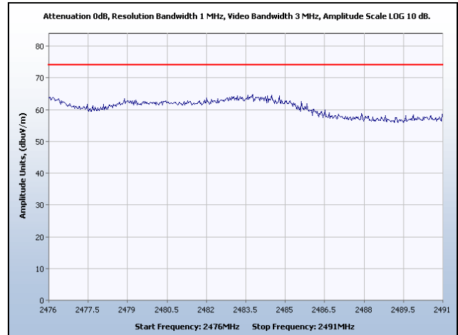
Restricted Band High Edge, Channel 10, 26 dBm, Peak
