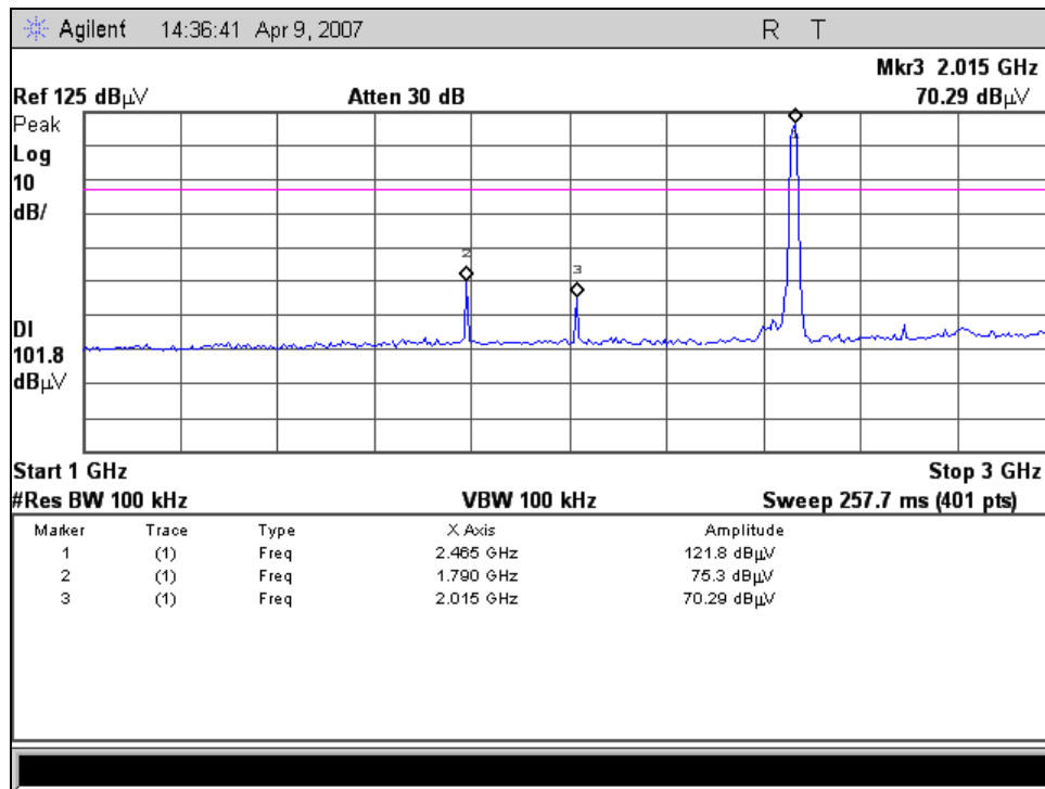
RF Conducted Spurious Emissions, 802.11b, Channel 11, 1-3 GHz
