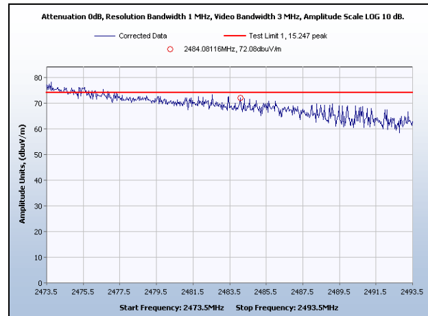
Restricted Band High Edge, Channel 10, 22 dBm, Peak
