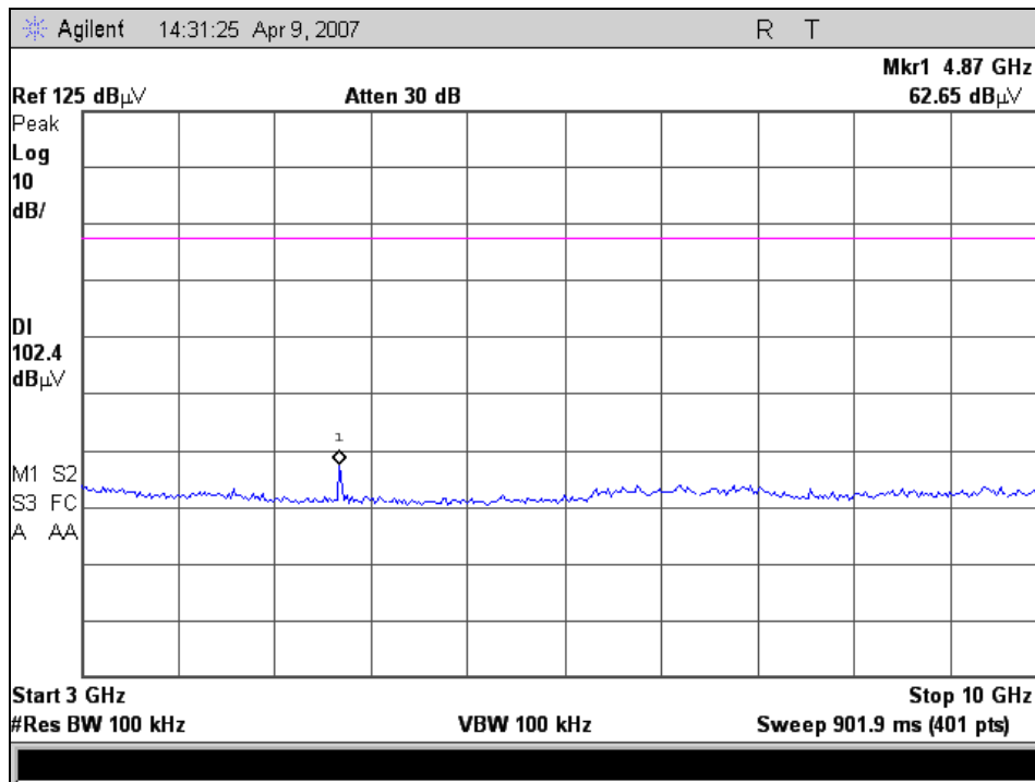
RF Conducted Spurious Emissions, 802.11b, Channel 6, 3-10 GHz
