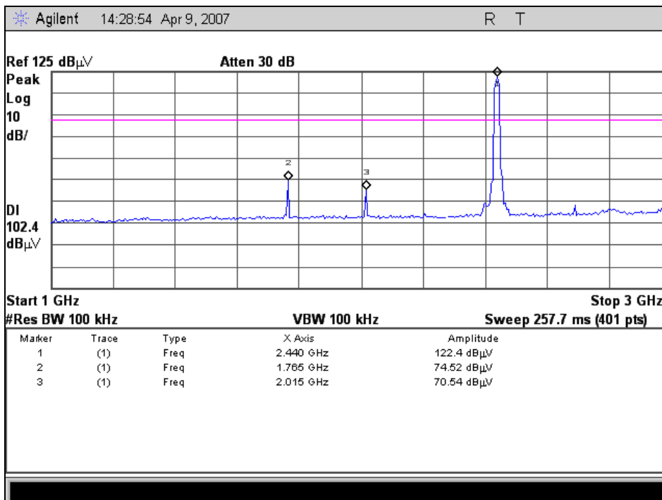
RF Conducted Spurious Emissions, 802.11b, Channel 6, 1-3 GHz
