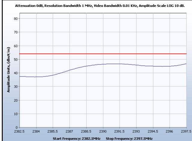
Restricted Band Low Edge, Channel 2, 27 dBm, Average
