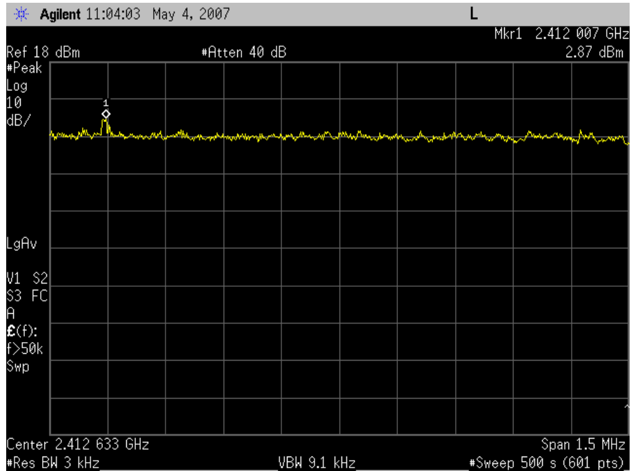
Peak Power Spectral Density, 802.11b, Channel 1
