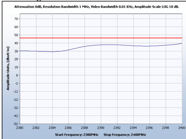
Restricted Band Low Edge, Channel 6, 25 dBm, Average
