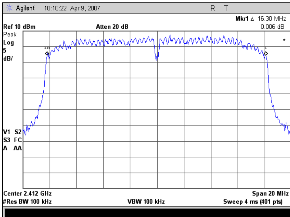
6 dB Occupied Bandwidth, 802.11g, Channel 1
