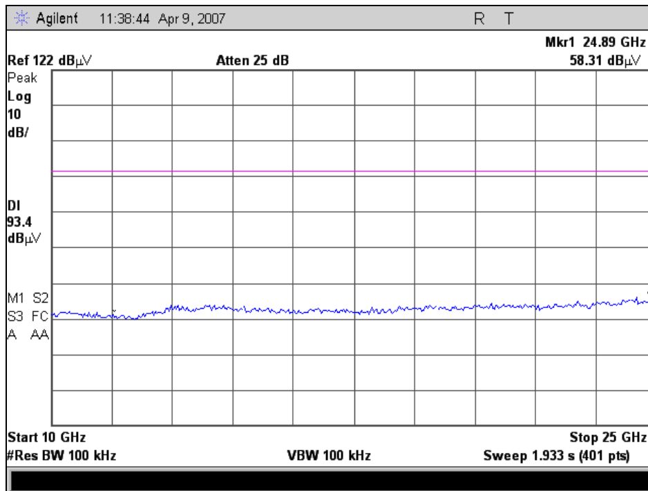
RF Conducted Spurious Emissions, 802.11g, Channel 11, 10-25 GHz
