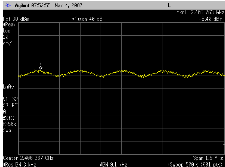
Peak Power Spectral Density, 802.11g, Channel 1
