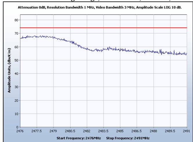
Restricted Band High Edge, Channel 11, 25 dBm, Peak
