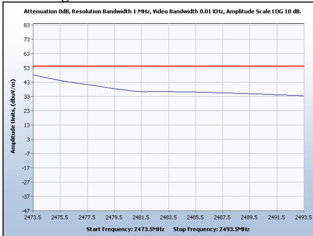
Restricted Band High Edge, Channel 10, 22 dBm, Average
