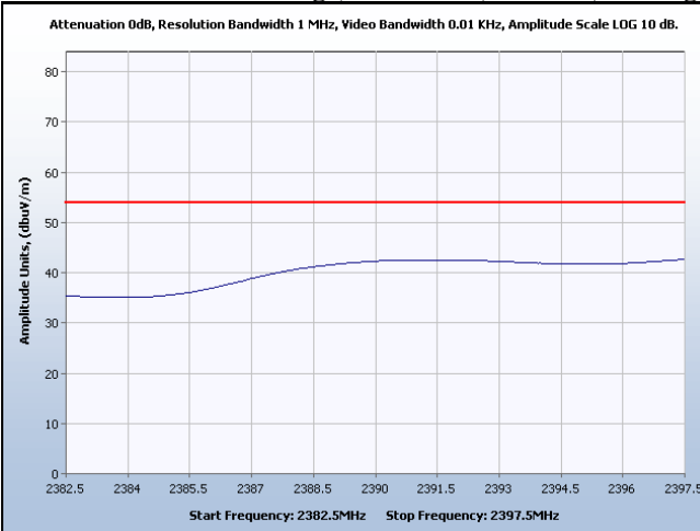
Restricted Band Low Edge, Channel 3, 27 dBm, Average
