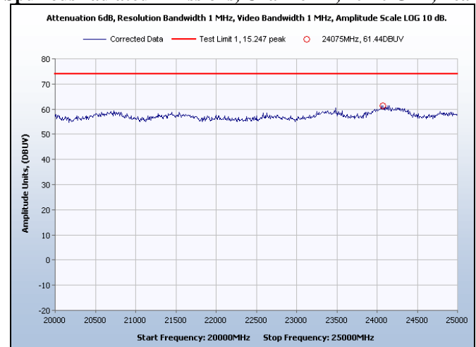
SpuriousRadiated Emissions, Channel 11, 20-25 GHz, Peak
