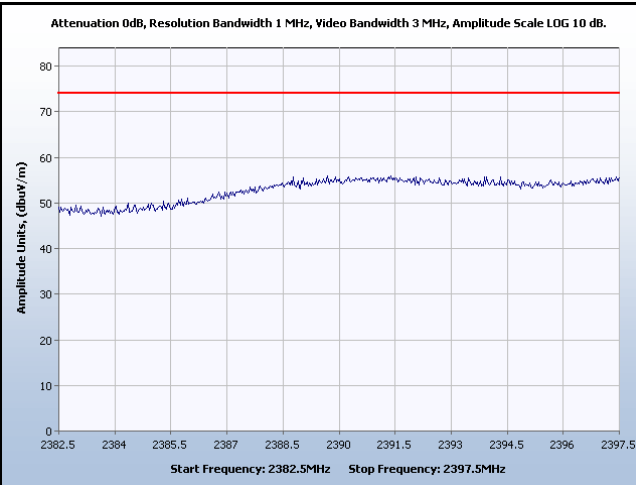
Restricted Band Low Edge, Channel 3, 27 dBm, Peak
