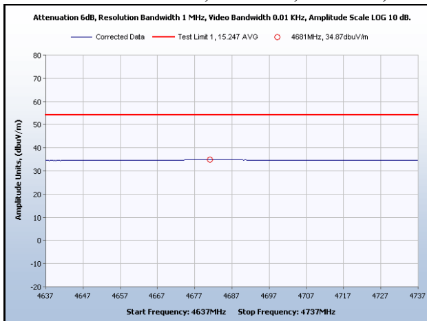
SpuriousRadiated Emissions, Channel 1, 2-5.5 GHz, Average
