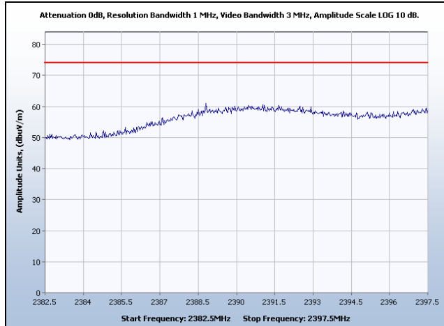
Restricted Band Low Edge, Channel 2, 27 dBm, Peak
