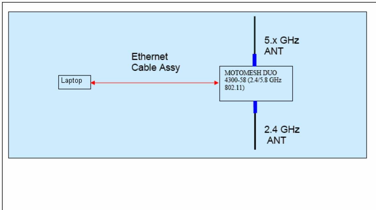
Figure 1. Block Diagram of Test Configuration (Radiated Emissions)
