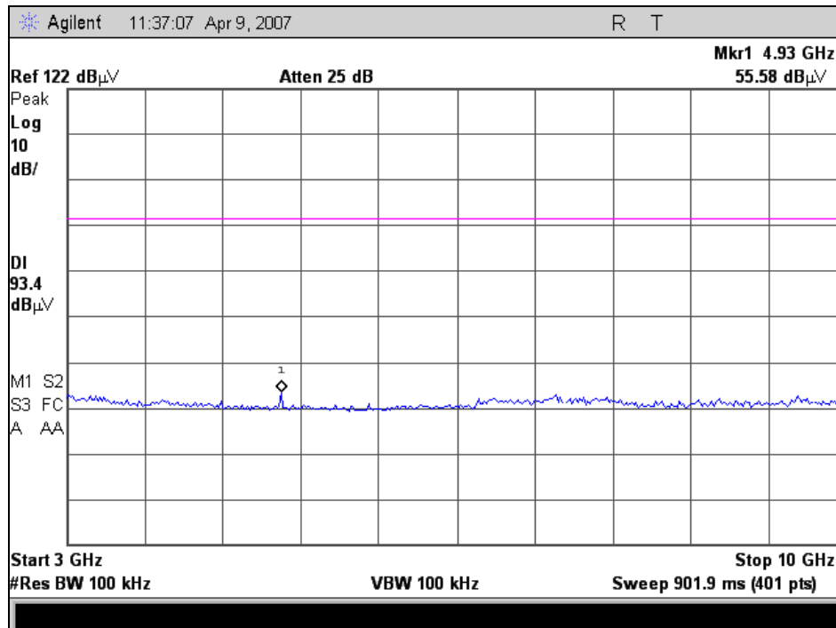
RF Conducted Spurious Emissions, 802.11g, Channel 11, 3-10 GHz
