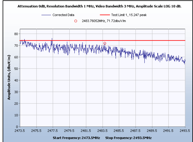
Restricted Band High Edge, Channel 11, 20 dBm, Peak
