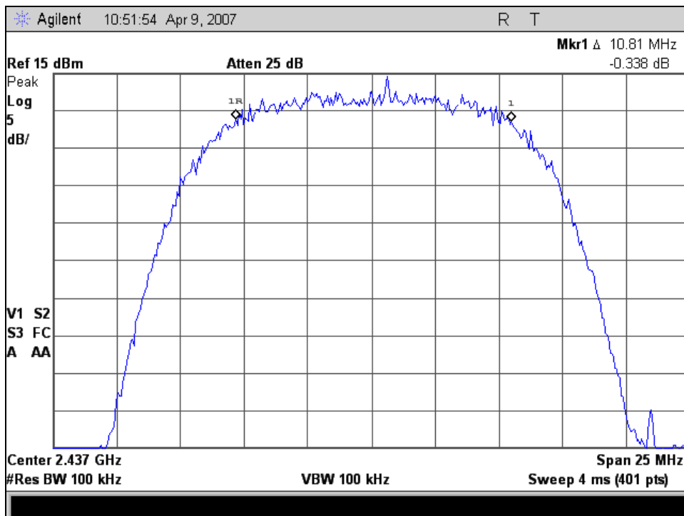
6 dB Occupied Bandwidth, 802.11b, Channel 6
