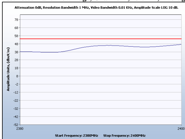
Restricted Band Low Edge, Channel 5, 25 dBm, Average
