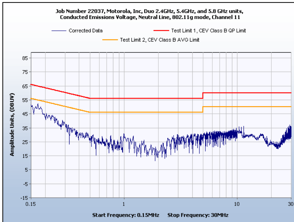
Channel 11 Neutral Line Plot
