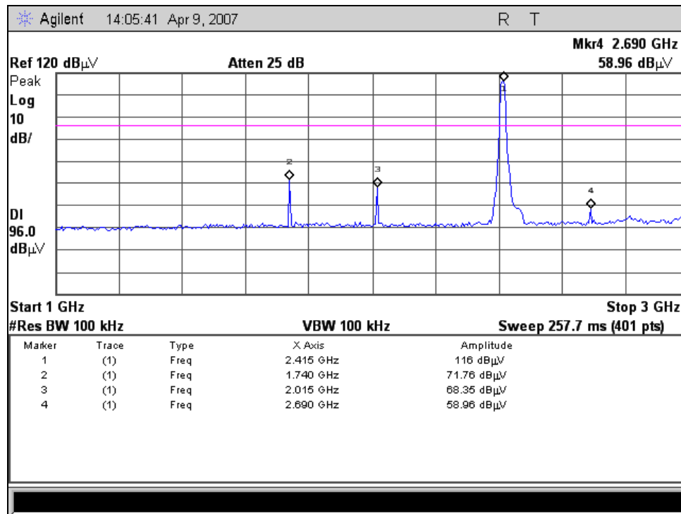
RF Conducted Spurious Emissions, 802.11g, Channel 1, 1-3 GHz
