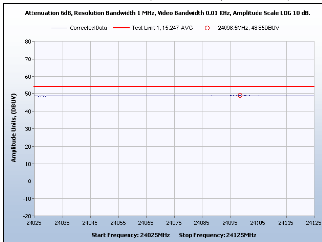
SpuriousRadiated Emissions, Channel 11, 20-25 GHz, Average
