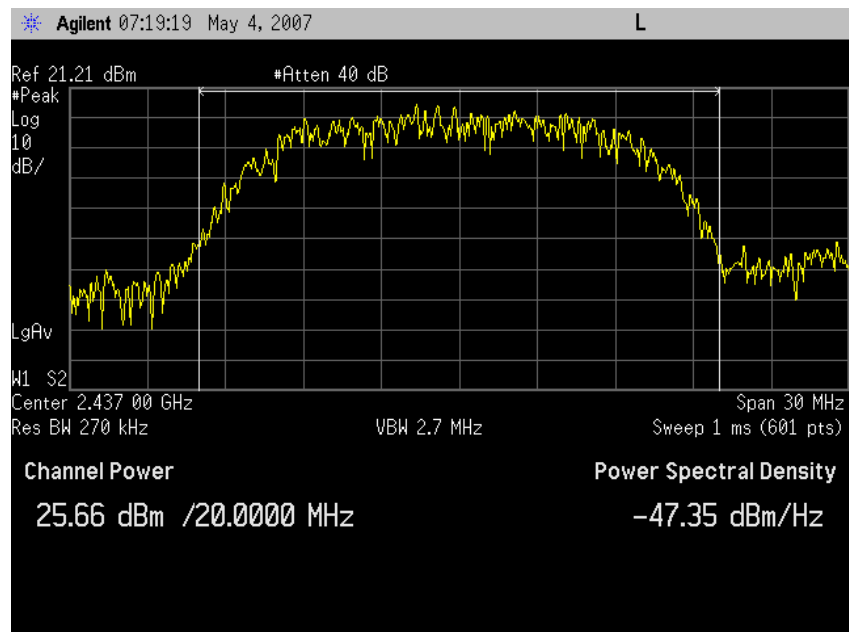
Peak Output Power,, 802.11b, Channel 6
