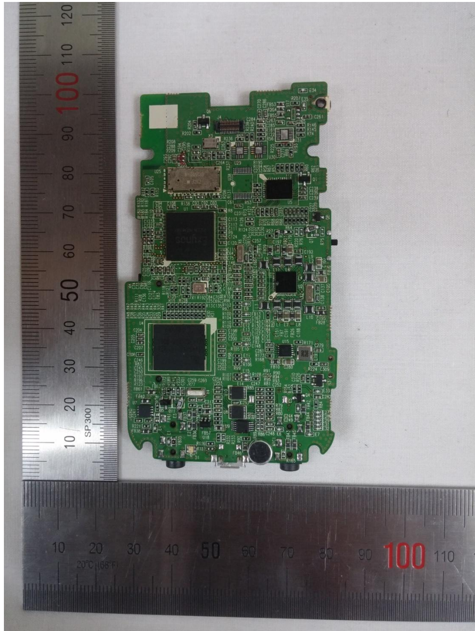
View of Main PCB (Bottom)
