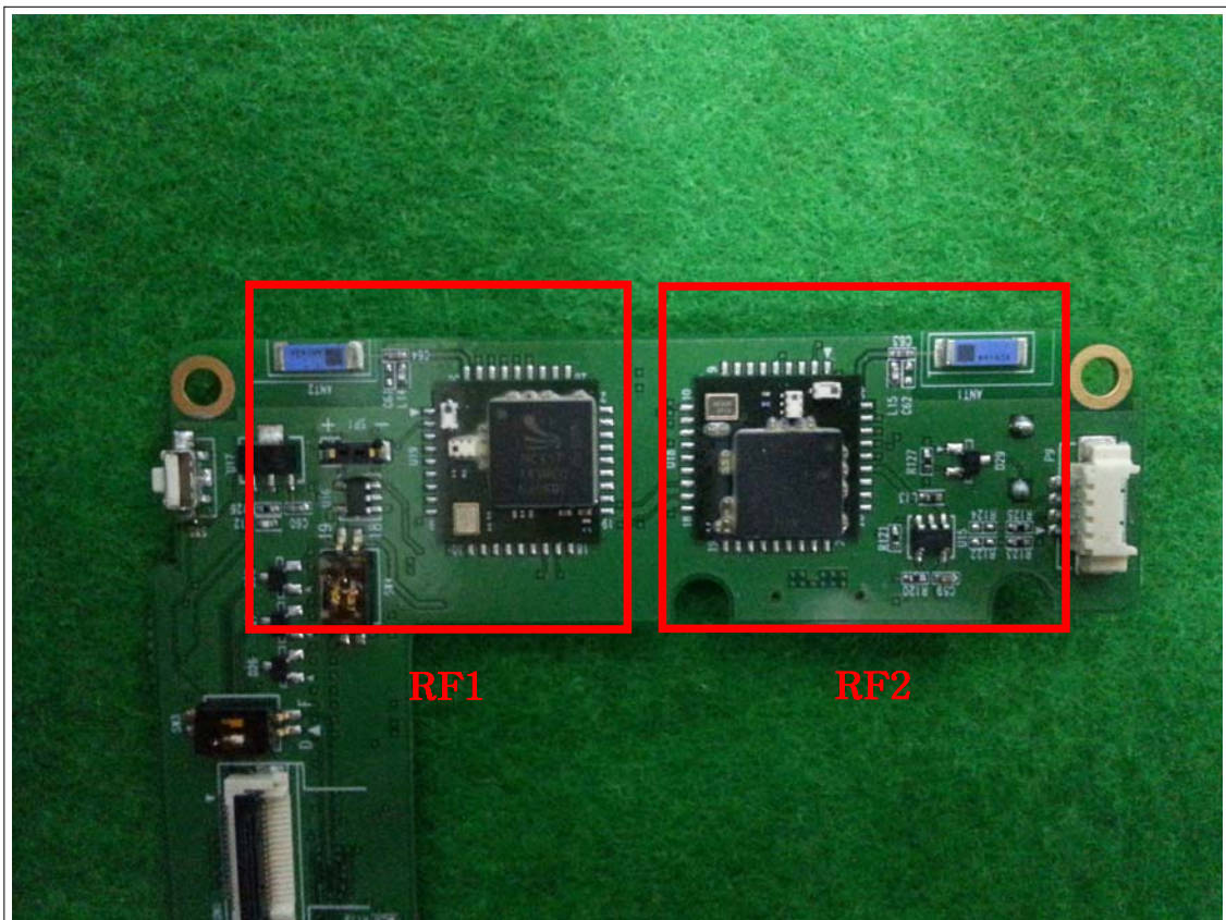
Chip Antenna and RF1/ RF2
