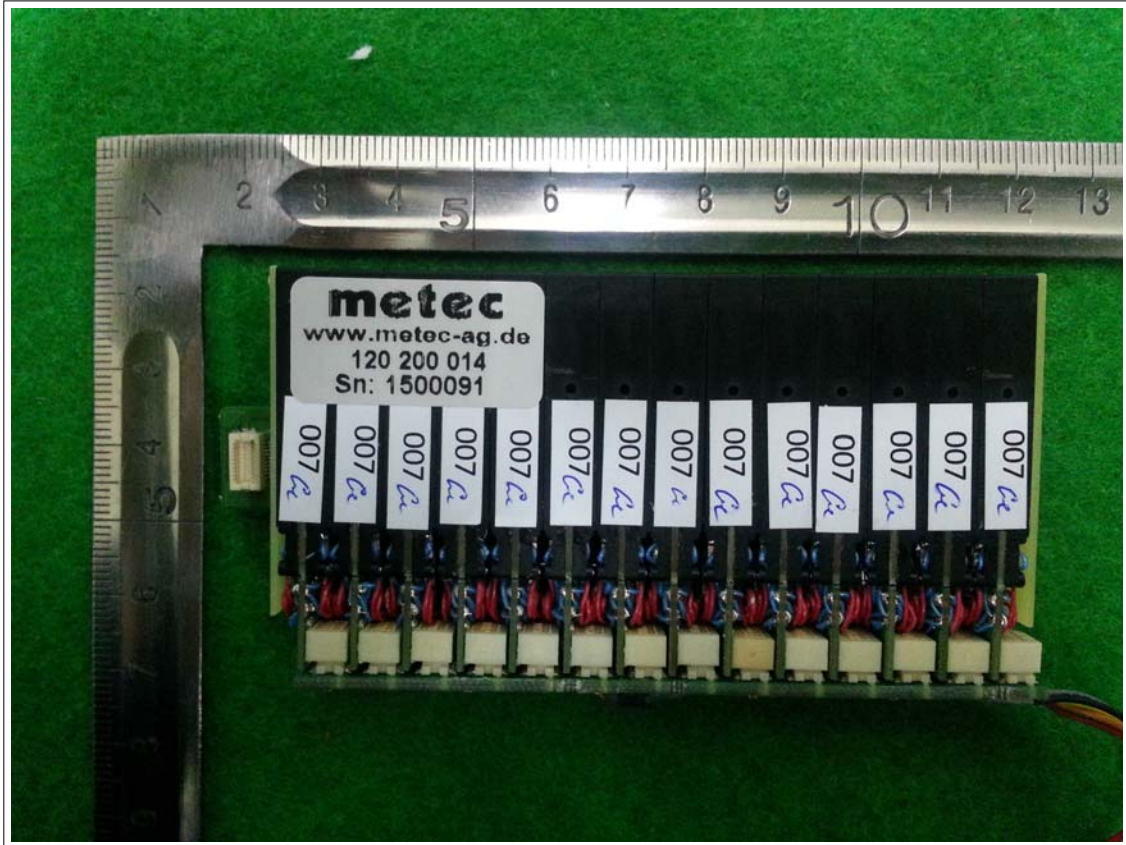
Side PCB 1(Top)
