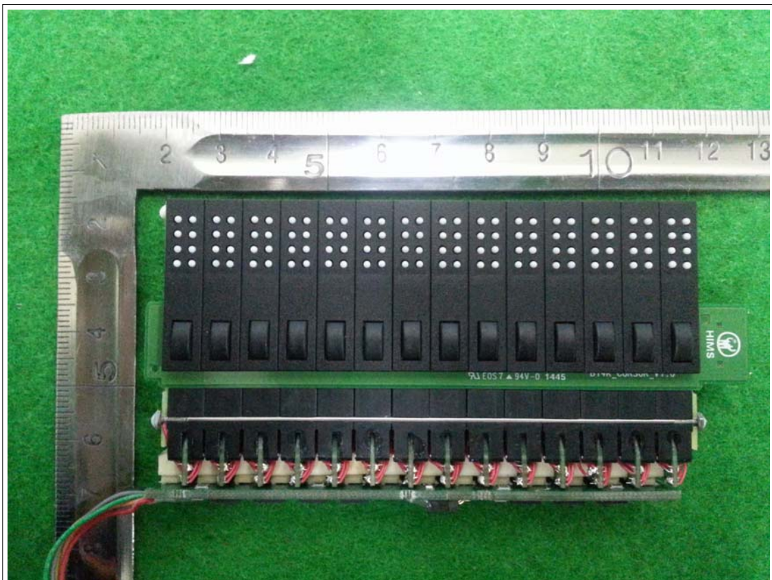
Side PCB 2(Bottom)
