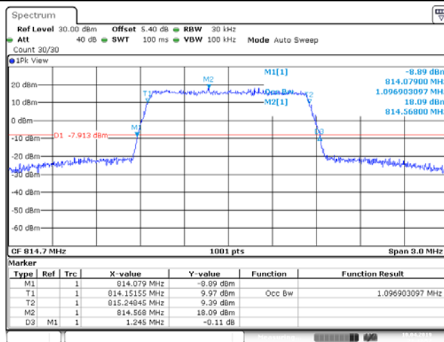
Band26_1.4MHz_QPSK_26697_6RB#0
