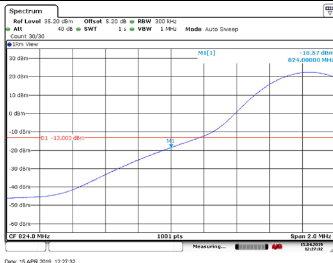
Band26_15MHz_16QAM_26865_50RB#0
