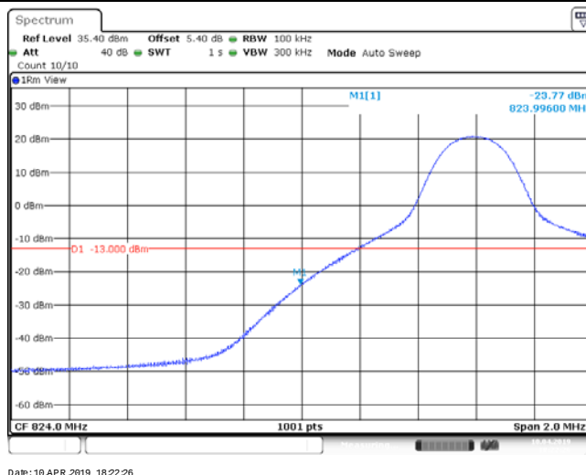
Band26_10MHz_16QAM_26840_50RB#0
