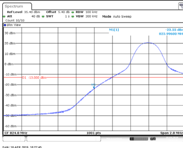
Band26_10MHz_64QAM_26840_50RB#0
