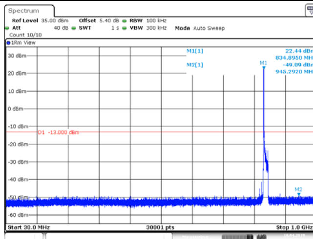
Band26_15MHz_64QAM_26965_1RB#0
