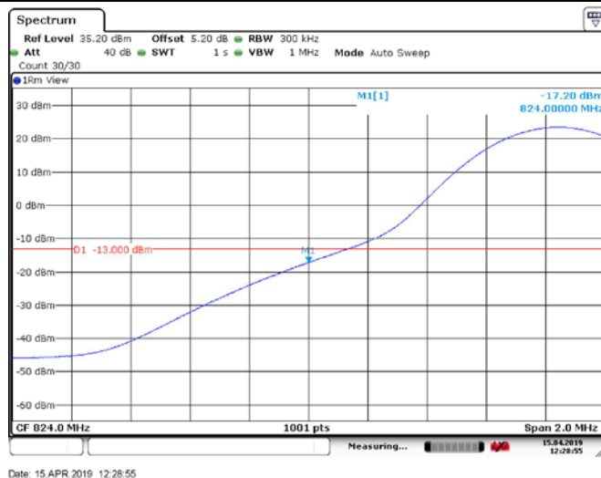
Band26_15MHz_QPSK_26865_50RB#0
