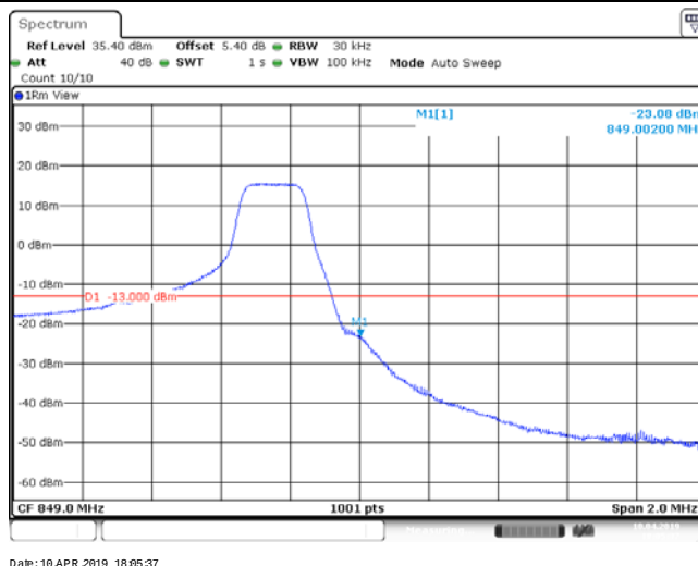
Band26_1.4MHz_64QAM_27033_6RB#0
