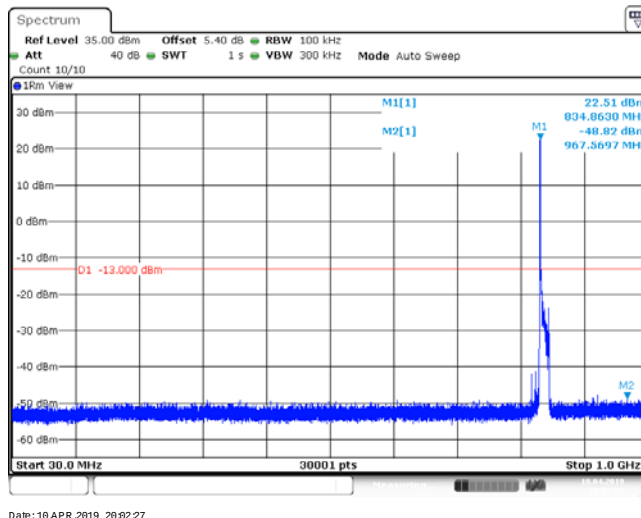
Band26_15MHz_QPSK_26965_1RB#0
