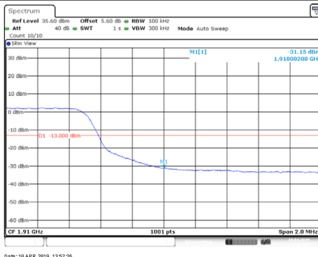
Band2_15MHz_QPSK_18675_1RB#0
