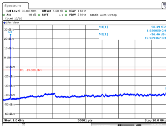
Band2_20MHz_64QAM_18700_1RB#0
