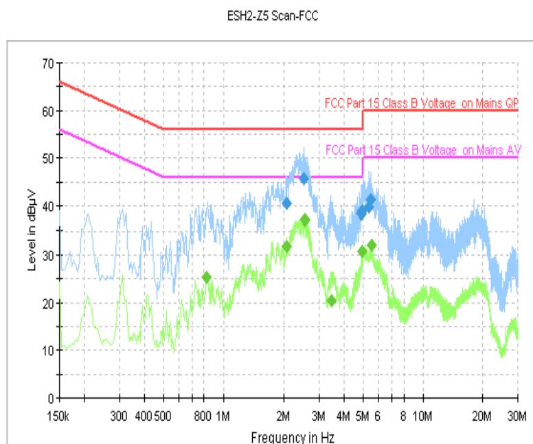
Fig. 34 AC Power line Conducted Emission (Idle, AE2)
