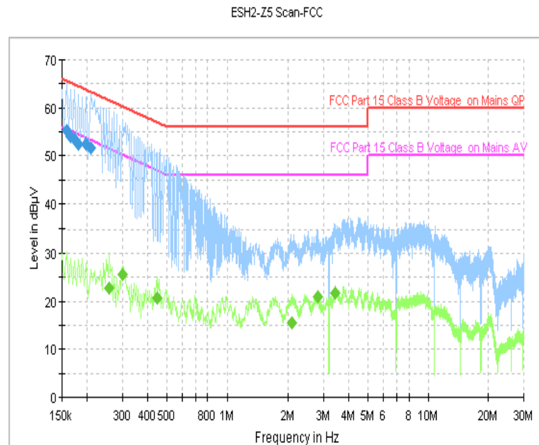
Fig. 35 AC Power line Conducted Emission (Idle, AE3)
