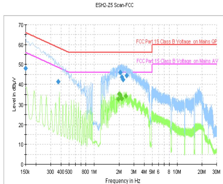
Fig. 33 AC Power line Conducted Emission (Idle, AE1)
