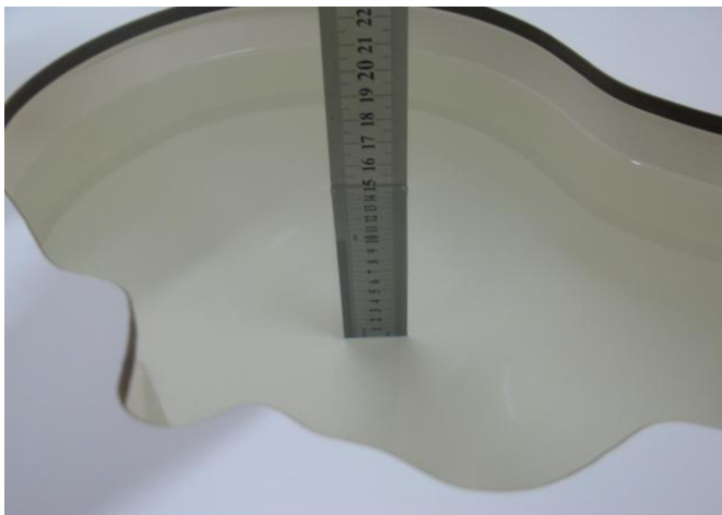
Photo 20:HSL 2450MHz depth (15.1cm)
