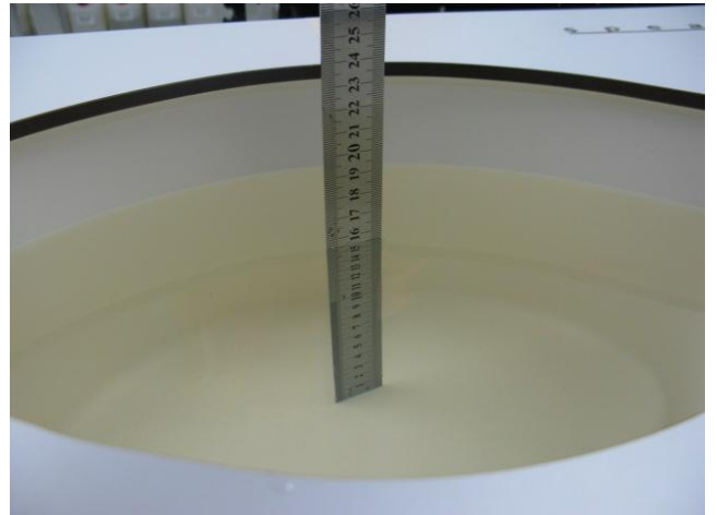
Photo 19:MSL 1800MHz depth (15.3cm)
