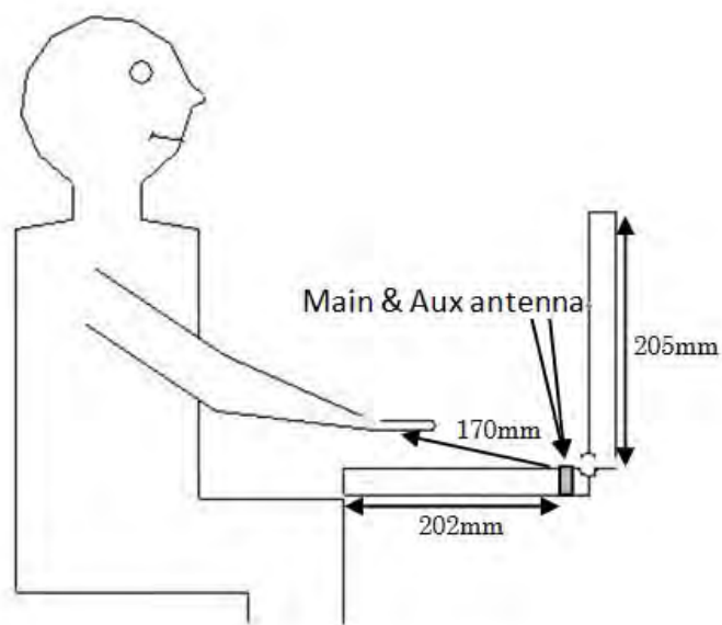
Fig.8 Antenna-to-user separation distance
