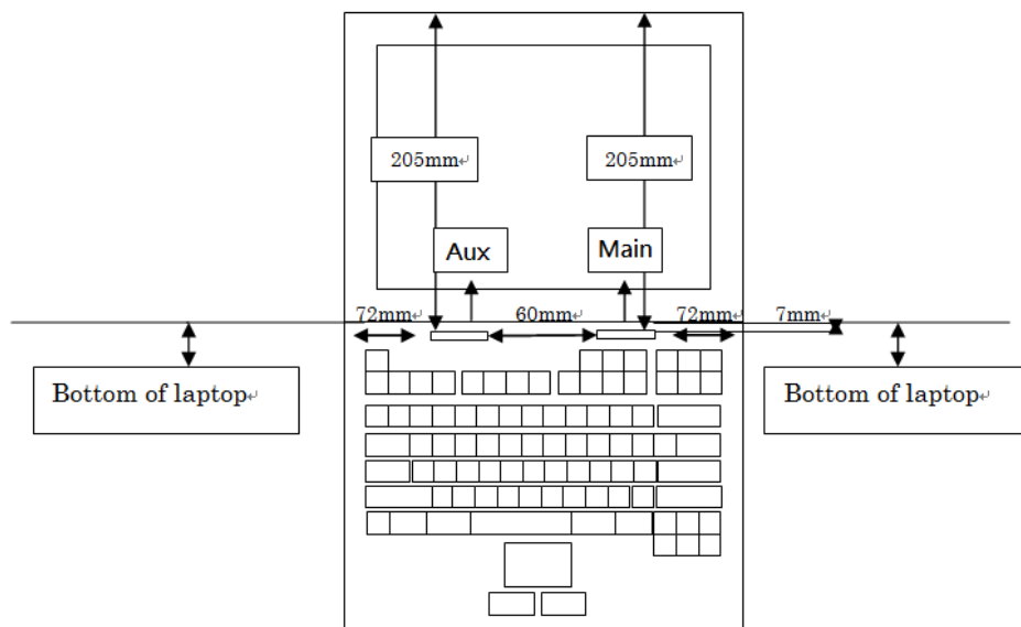
Fig.7 Antenna position of EUT (Front view)
