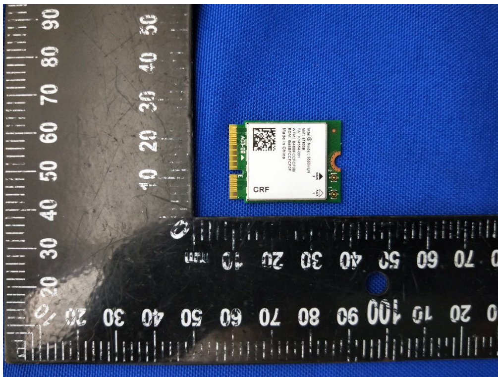
RF Module TOP VIEW (WITH SHIELDING)
