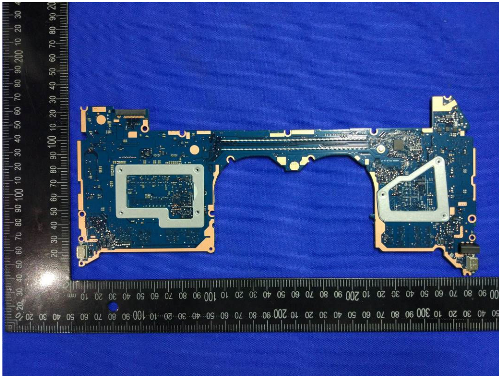
WRT-W09, WRT-W19, WRT-W29(without GPU) MAIN BOARD REAR VIEW
