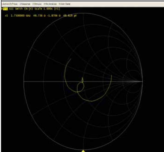
Impedance Test-Body
